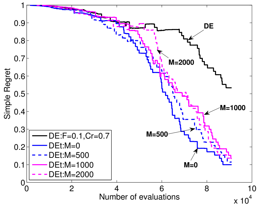
(b) Truncated-DE compared to normal DE, \lambda = 10 .
