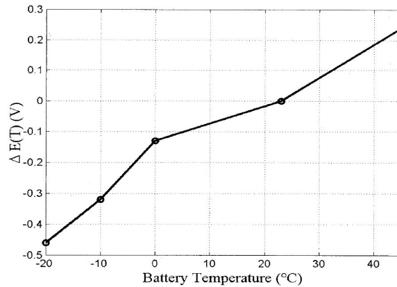
Figure 25. Temperature-dependent potential-correction term. Reference temperature is at 23°C.
