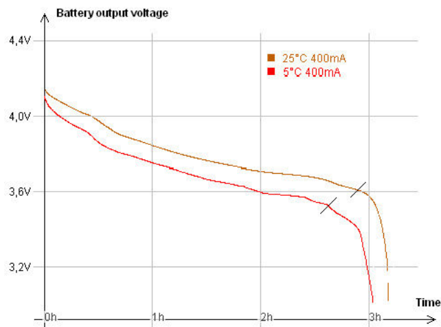
Figure 24. Battery output voltage under different temperature conditions.
