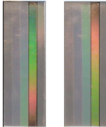
Figure 21. Left: temperature visualization 18 min at 6C test without cooling. Right: the same image 34 min into the test with cooling [77].
