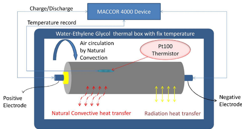
Figure 14. Experiment set-up [73].
