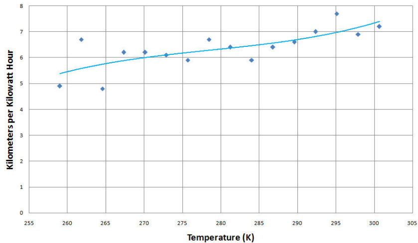
Figure 23. Impact of temperature on electrical performance.
