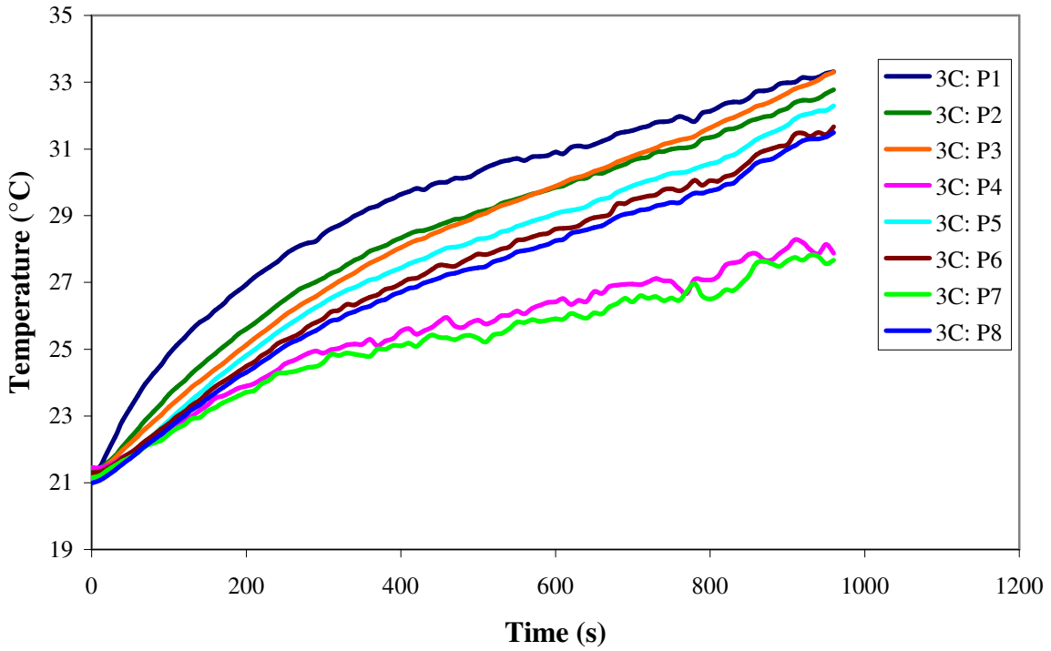
Figure 58. Cell surface temperature at 3C discharge rate with cooling air velocity of 2 m/s at air temperature of 21°C.
