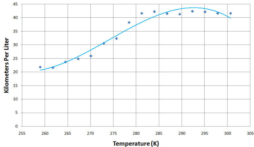
Figure 22. Impact of temperature on fuel economy.
