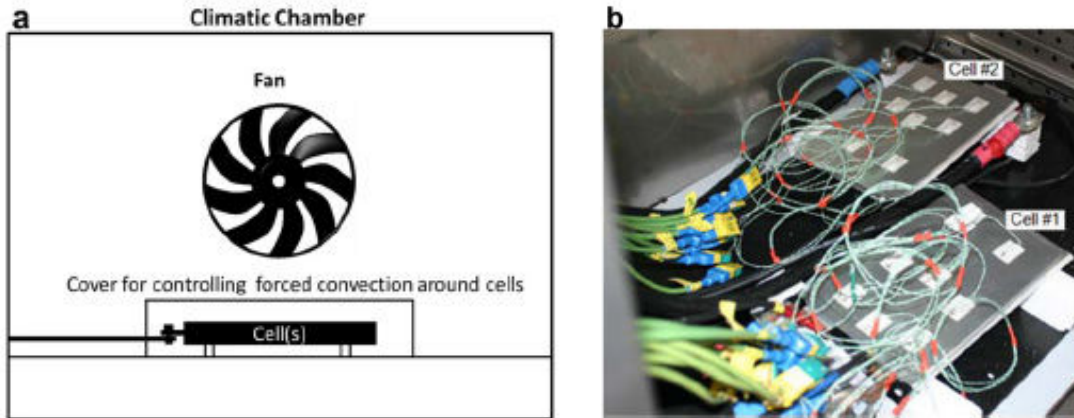
Figure 17. a) Schematic of Li-ion cell test set up, b) instrumented cell in climatic chamber [31].
