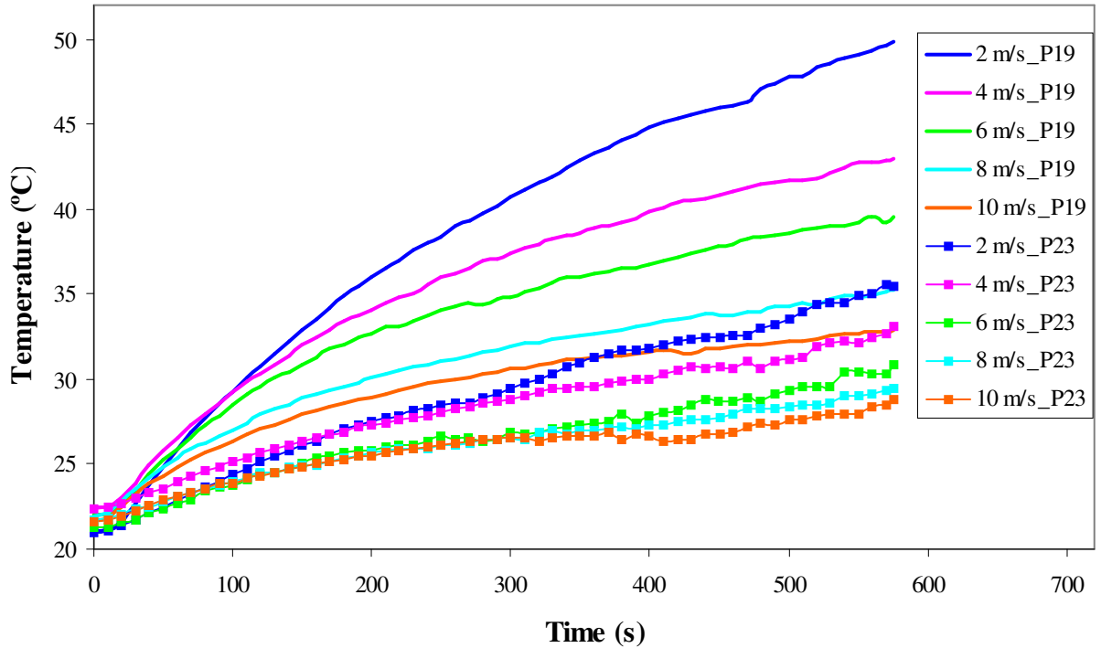
Figure 65. Cell surface temperature of surface 2R (P19 and P23) at different cooling air velocity for 5C discharge rate.
