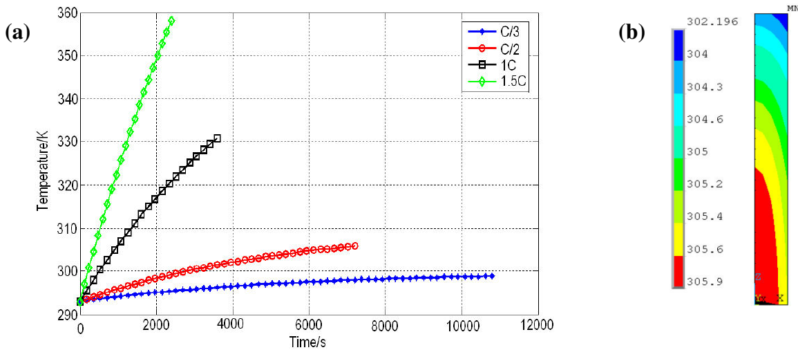
Figure 34. a) Battery inner temperature rise at different discharge rates, b) temperature field [72].
