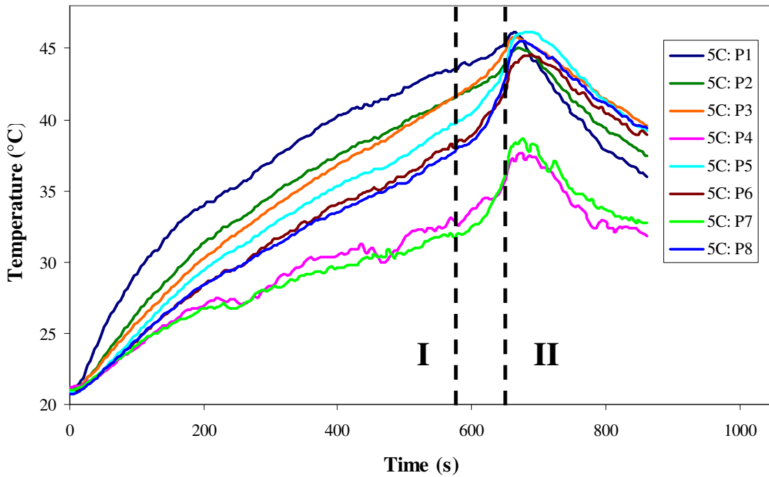
Figure 72. Cell surface temperature evolution under 5C discharge rate at cooling air velocity of 2 m/s for abuse discharge at first cell.
