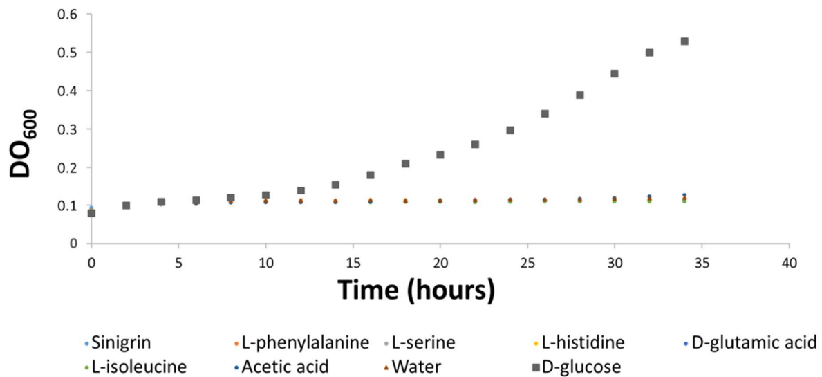
FIG 4 Growth curves of X. campestris pv. campestris strain ATCC 33913 in minimal medium (MME) supplemented with sinigrin, L-phenylalanine, L-serine, L-histidine, L-glutamic acid, L-isoleucine, acetic acid, D-glucose or water. Molecules were concentrated at 10 mM.
