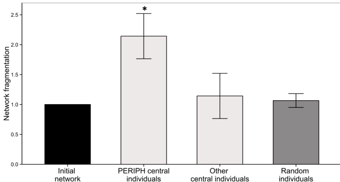
Figure 5: Evolution of network stability after the simulated removal of individuals
