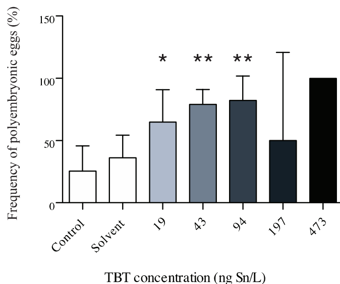
Figure 2.6. Frequency of the polyembryonic eggs (among the total number of abnormal eggs) found during a 21-d exposure to tributyltin (TBT). Error bars represent standard deviation over all abnormal egg produced (★: p < 0.05 ; ★★: p < 0.01 ).
