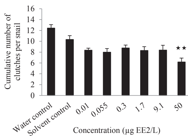
Figure 5.1. Effect of EE2 on the cumulative number of egg clutches per snail in the 56-d test with adult snails. Error bars represent the standard error. Asterisks indicate a significant difference ( 0.001 < p < 0.01 ) between data obtained in treatments and the control.
