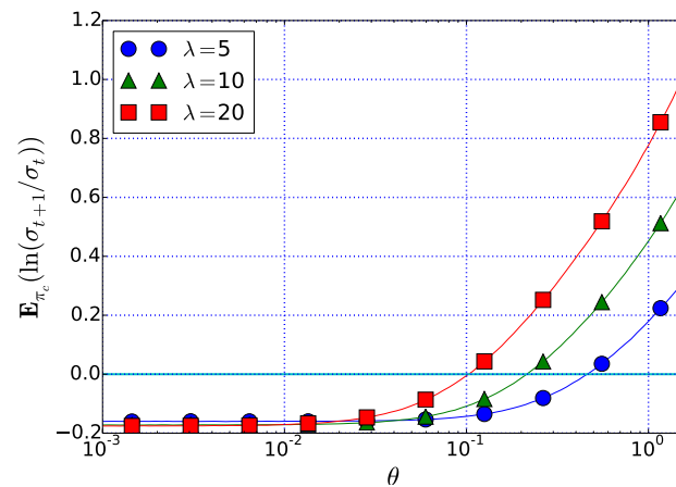
Figure 6: Average of the logarithmic adaptation response \Delta_t = \ln(\sigma_{t+1}/\sigma_t) for the (1, \lambda) -CSA-ES plotted against the constraint angle \theta , for \lambda \in \{5, 10, 20\} , c = 1/\sqrt{2} , d_\sigma = 1 and dimension 2. Values below zero (straight line) indicate premature convergence.
