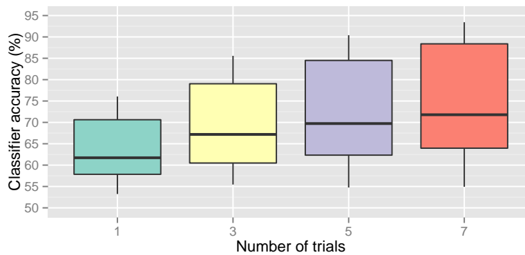
Figure 5.7 – Classifier accuracy depending on the size of trials clusters
