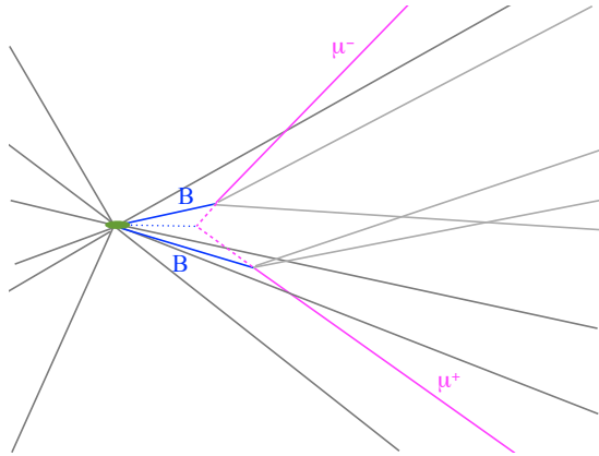
Figure 3.3: Schematic representation of a combinatoric background event for B_{(s)}^0 \rightarrow \mu\mu .
