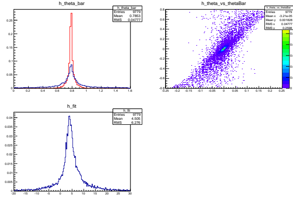
Figure 4.17: Top-left: for \alpha = 1 distribution of \bar{\theta} (red) and \theta (blue); top-right: \theta - \frac{\pi}{4} (y axis) vs \bar{\theta} - \frac{\pi}{4} (x axis); bottom-left: distribution of (\theta - \frac{\pi}{4})/(\bar{\theta} - \frac{\pi}{4}) , whose mean can be used as a rough estimation of the coefficient between \theta and \bar{\theta} .
