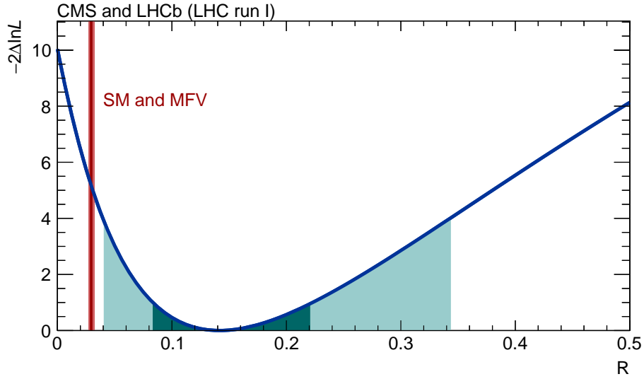
Figure 3.32: Test statistic -2\Delta \ln L as a function of \mathcal{R} = \mathcal{BR}(B^0 \rightarrow \mu\mu)/\mathcal{BR}(B_s^0 \rightarrow \mu\mu) . The dark and light cyan areas are the \pm 1\sigma and \pm 2\sigma regions. The SM prediction with its uncertainty is indicated by the red line.
