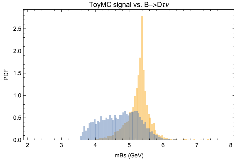
Figure E.4: Distribution of the “best” reconstructed invariant mass of the B_s^0 candidate ( i.e. whose value is closest to the nominal one) for MC generated signal events (orange) and the B^0 \rightarrow \bar{D}\tau^+\nu_\tau background (light blue).
