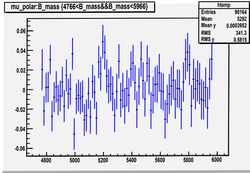
Figure 3.11: Average value of the ‘polar_angle’ variable as a function of m_{\mu\mu} for b\bar{b} \rightarrow \mu\mu X MC generated events.
