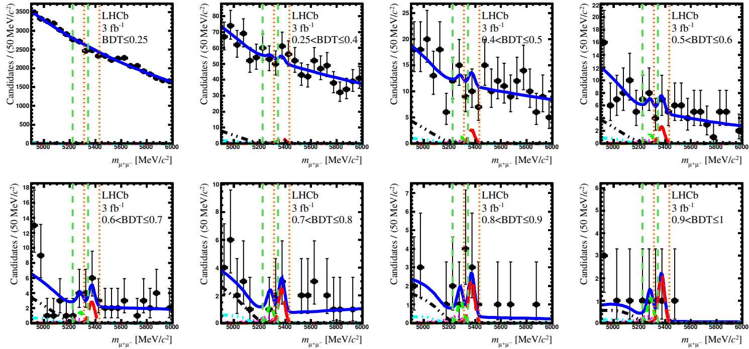
Figure 3.27: Fit results in the eight BDT bins. The contribution from the peaking B_{(s)}^0 \rightarrow hh^{(l)} is the dashed pink line, the one from B_{(s)}^0 \rightarrow \pi^+(K^-)\mu^+\nu_\mu is the dashed black line, the one from B^{0(+)} \rightarrow \pi^{0,(+)}\mu^+\mu^- is the dashed cyan line; the B_s^0 \rightarrow \mu^+\mu^- signal is indicated in red, the B^0 \rightarrow \mu^+\mu^- signal component in green, and the fit result is the continuous blue line.
