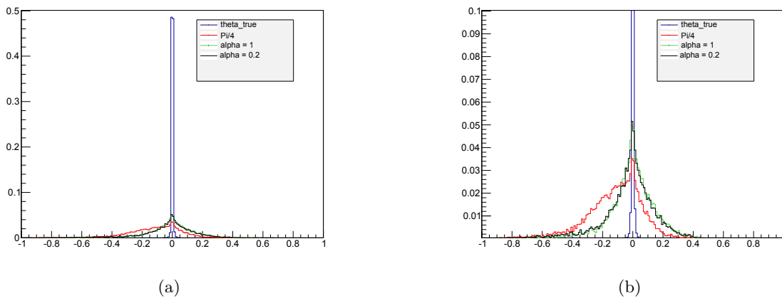
Figure 4.19: Precision on the reconstructed solution whose value is closest on the true one ( i.e. 2 \frac{|\xi_{best} - \xi_{true}|}{|\xi_{best}| + |\xi_{true}|} ) found for different approximations of \theta .
