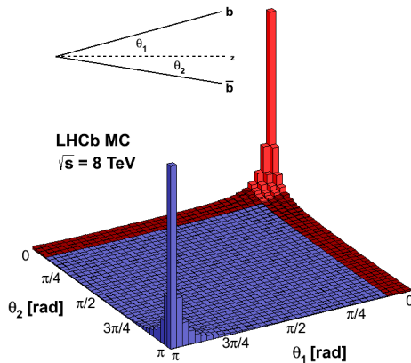
Figure 2.5: Angular correlation between the two b quarks produced in proton-proton collision.
