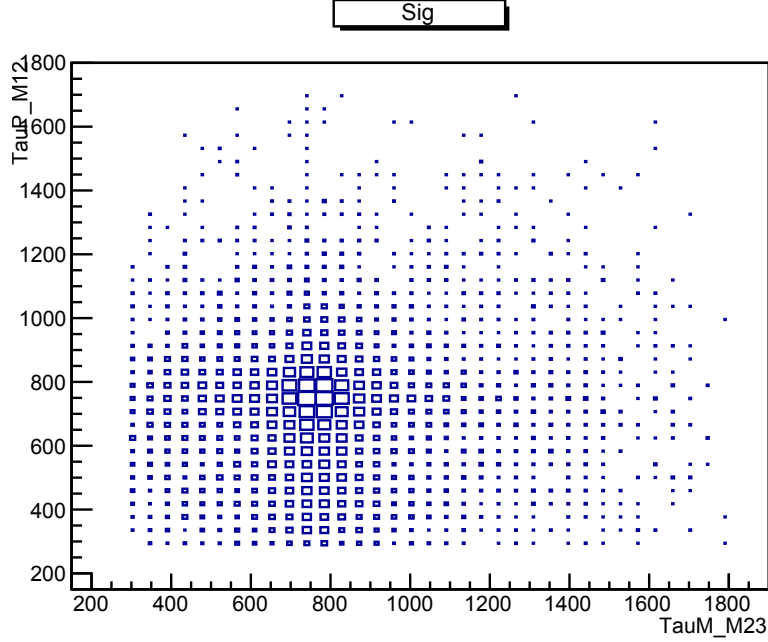
Figure 4.4: Dalitz plane of the m_{\pi^+\pi^-} variables for pions coming from a \tau \rightarrow 3\pi\nu decay.
