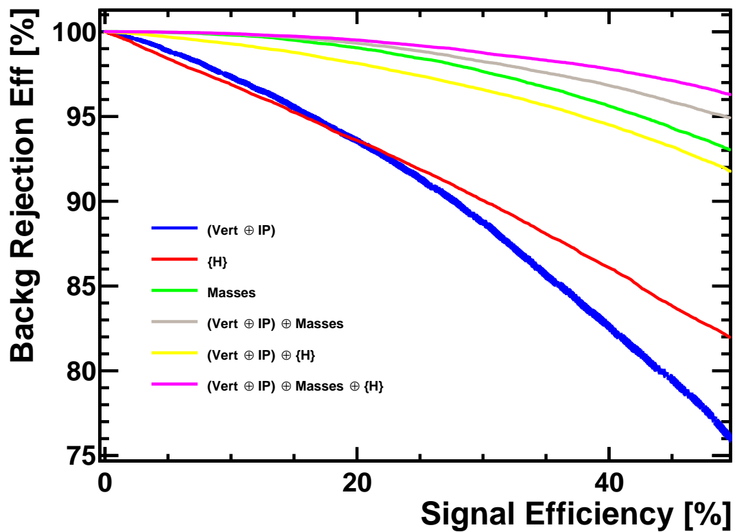
Figure C.2: ROC curves obtained with the output variables of several BDT classifiers trained with different sets of input variables. A statistically significant improvement is observed (pink line) when the elements of the H matrix are added to the set of the input variables of the classifier. Zoom of Fig.C.1 in the low signal efficiency region.
