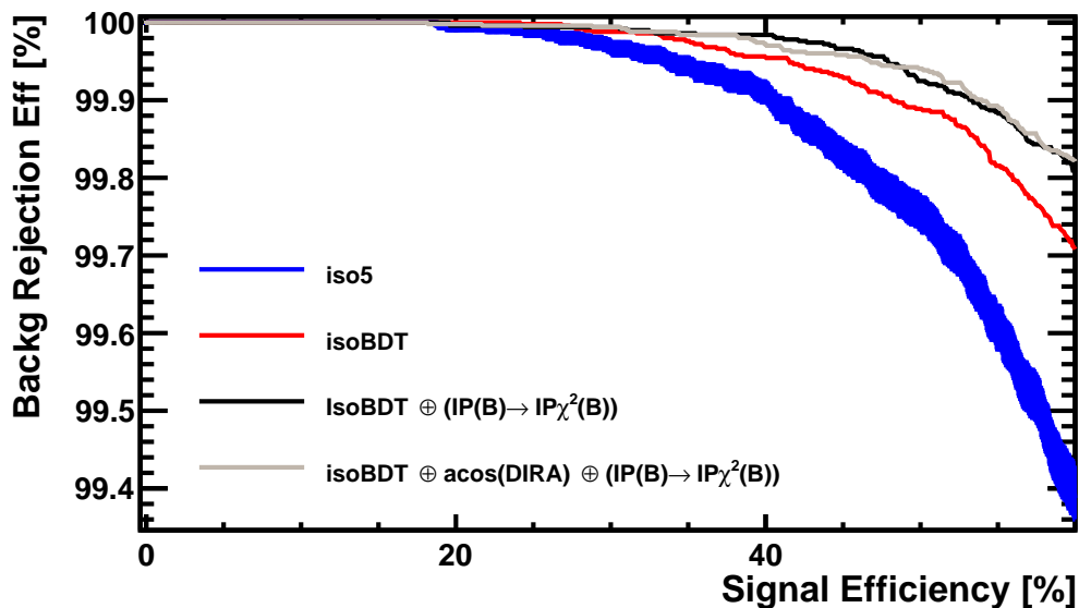
Figure 3.56: ROC curves of BDT classifiers trained using the basic set of 11 input variables plus the combinations shown in the plot. “iso5” is the standard isolation variable, “acos(DIRA)” is one of the two pointing related variables.
