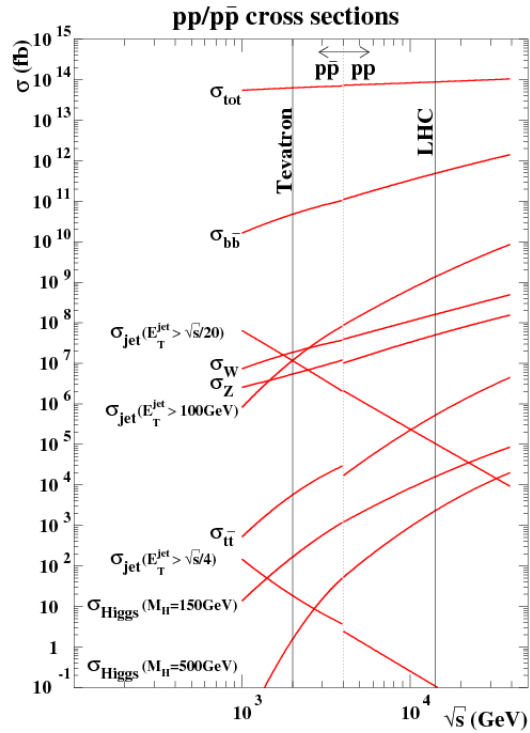
Figure 2.15: pp cross section for different processes as a function of the energy in the center of mass of the two proton beams ( \sqrt{s} ).
