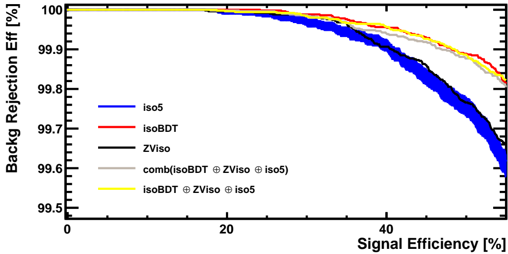
Figure 3.49: ROC curves of the four final BDT classifiers trained with different muon isolation variables. “comb(isoBDT⊕ZViso⊕iso5)” is the ROC curve of the classifier using the combination of all isolations, “isoBDT⊕ZViso⊕iso5” is the ROC curve of the classifier using the three isolations as separate input of the BDT classifier.
