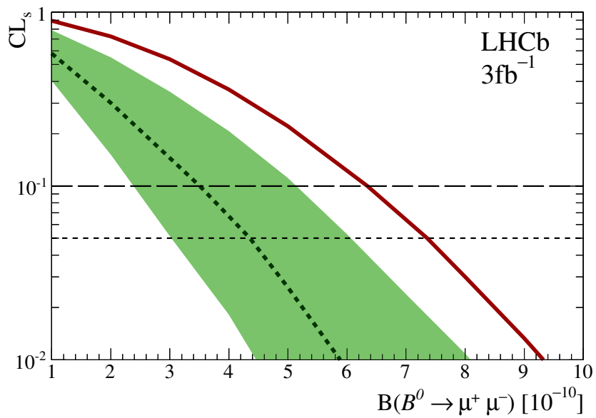
Figure 3.26: CL_s as a function of different hypotheses on \mathcal{BR}(B^0 \rightarrow \mu^+ \mu^-) . The dashed black line is the median of the expected CL_s distribution for the background only hypothesis, the green band represents its 1\sigma range, and the solid red curve is the observed CL_s .
