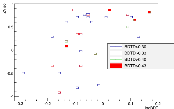
Figure 3.51: Values of the Z_{\text{Viso}} isolation variable as a function of the ones of the isoBDT for those events removed by different cuts on the output of the final BDT trained with the isoBDT muon isolation variable. For the color convention see Tab.3.22.
