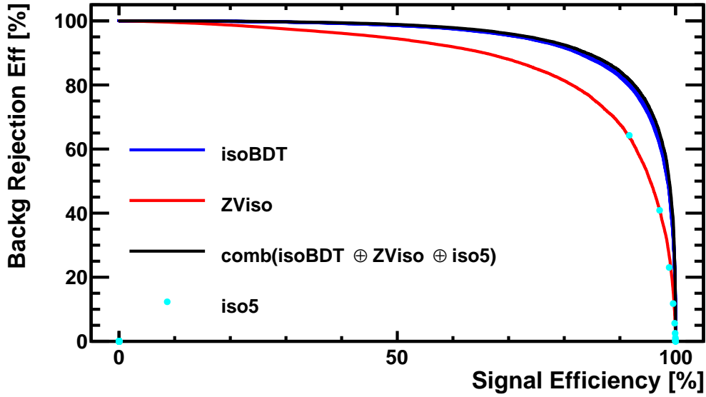
Figure 3.47: ROC curves of the four isolation variables. The standard isolation variable (here called “iso5”) has isolated points being a discrete variable, while all others are continuous lines, being calculated from continuous distributions.
