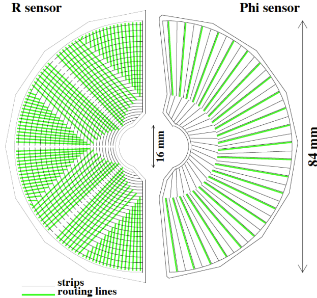
Figure 2.8: VELO sensors geometries.
