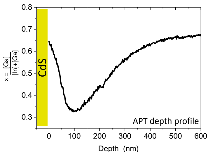
Figure 5.6: Ga ratio ( x ) as a function of thin film depth for CIGSe sample x=0.5 prepared using 3-stage process. This measurement is performed in APT by preparing tip parallel to thin film growth direction.
