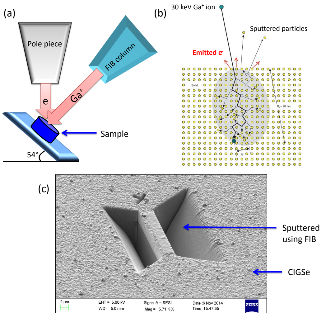
Figure 2.11: Schematic diagram depicting (a) relative position of Ga ion source and electron source in SEM/FIB. (b) Various mechanisms upon interaction of high energy Ga ions with material. (c) CIGSe lamella prepared after sputtering surrounding region with Ga ions in FIB.
