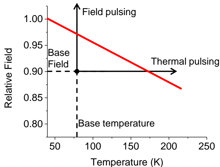
Figure 2.15: Two different modes of pulsing (field and thermal) to trigger field evaporation.
