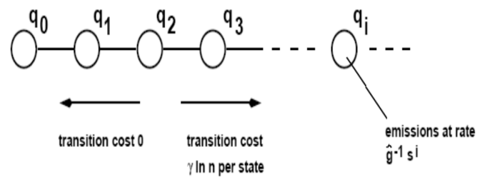
Figure A.1: The infinite-state automaton A_{s,\gamma}^* ; in state q_i , messages are emitted at a spacing in time that is distributed according to f(x) = \alpha_i e^{-\alpha_i x} , where \alpha_i = \hat{g}^{-1} s^i and \gamma is a parameter that controls the ease with which the automaton can change states.
