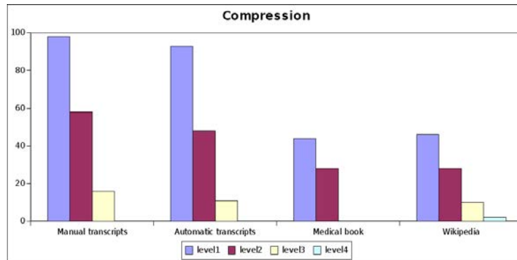
Figure 4.9: Compression statistic
