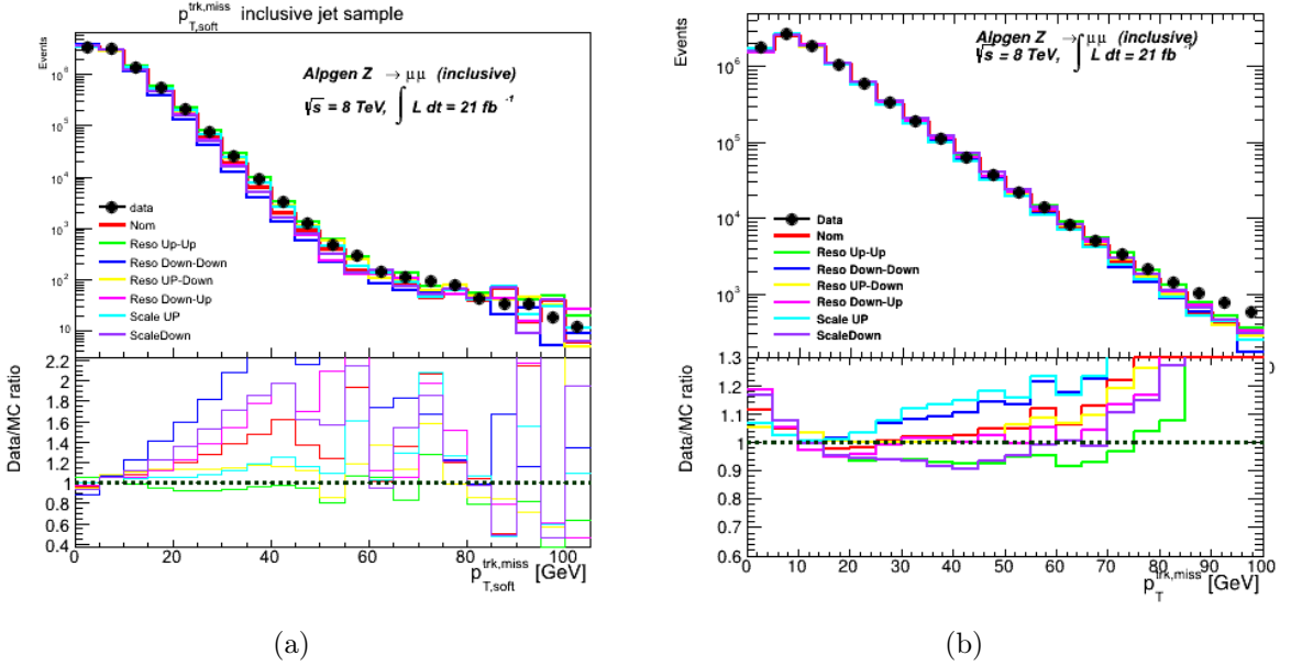
Figure 5-14: Distributions of p_{T,soft}^{miss} varied according to equation (5.7) are shown in (a) along with the corresponding total p_T^{miss} distributions (b) for the Z \rightarrow \mu\mu inclusive sample. The results are derived for Track MET-Cl-j derived using \Delta R method at \sqrt{s} = 8 TeV.
