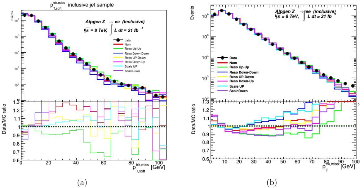
Figure 5-15: Distributions of p_{T,soft}^{miss} varied according to equation (5.7) are shown in (a) along with the corresponding total p_T^{miss} distributions (b) for the Z \rightarrow ee inclusive sample. The results are derived for Track MET-Cl-j derived using \Delta R method at \sqrt{s} = 8 TeV.
