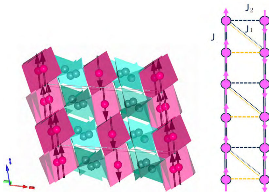
Figure 8.14: (Left) Representation of the magnetic structure of SrCoGe 2 O 6 ; (Right) the schematic drawing of exchange interactions, and here magnetic moments were added arbitrarily in order better to exhibit the triangular exchange interaction.
