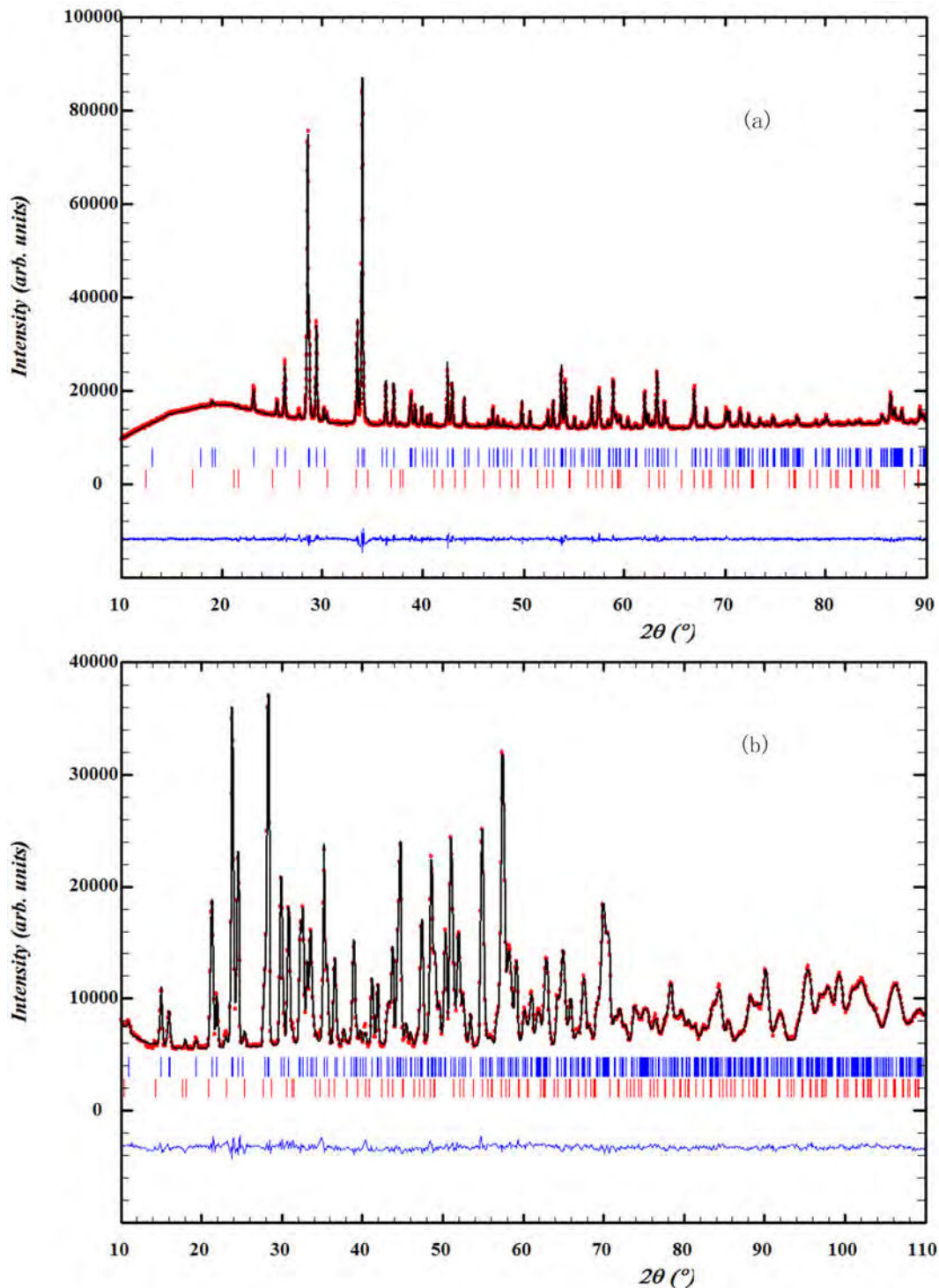
Figure 8.2: Rietveld refinement plots of SrCoGe 2 O 6 for XRPD (a) and NPD (b) patterns taken at room temperature. Observed (red), calculated (black), and difference (blue) plots are shown. Bragg reflections from the main phase are denoted by blue tick marks. The lower set of Bragg reflections belong to a Sr 3 CoGe 5 O 14 impurity phase.
