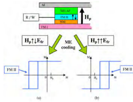
Figure 1.8: Schematics of a ME-RAM cell. [17]
