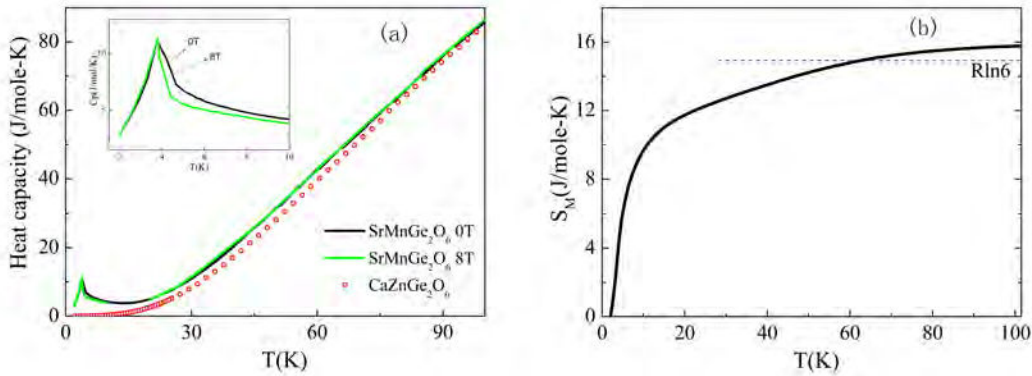
Figure 8.10: (a) Specific heat capacity of SrMnGe 2 O 6 and CaZnGe 2 O 6 which is employed as a lattice analog. Inset shows the comparison of HC at 0T and 8T. (b) The magnetic entropy released via magnetic ordering.
