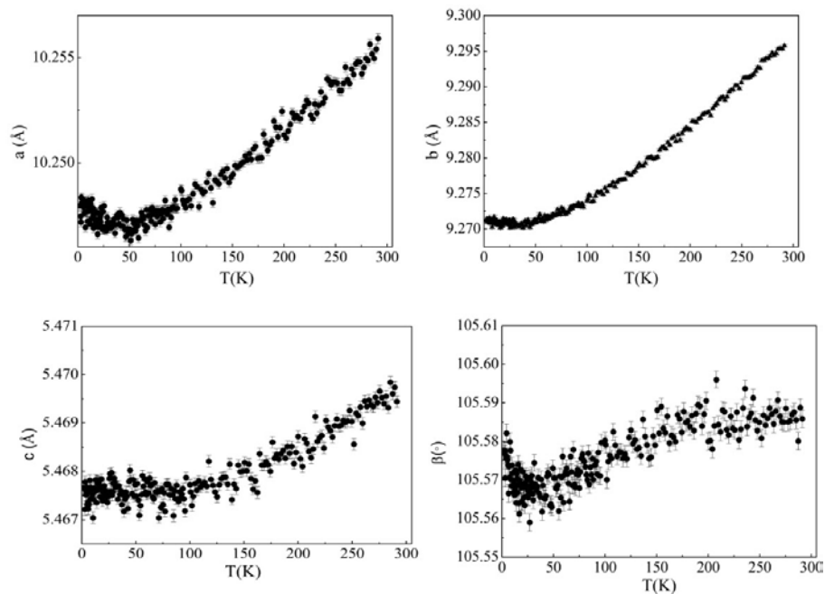
Figure 8.16: Lattice parameters of SrCoGe 2 O 6 as a function of temperature derived from NPD data.
