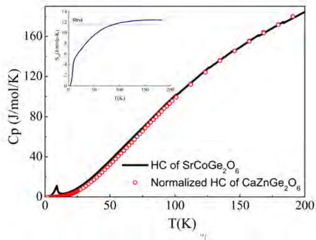
Figure 8.7: Specific heat capacities of SrCoGe 2 O 6 and CaZnGe 2 O 6 which is used as a lattice standard after normalizing its HC at 200K. Inset shows the magnetic entropy for SrCoGe 2 O 6 .
