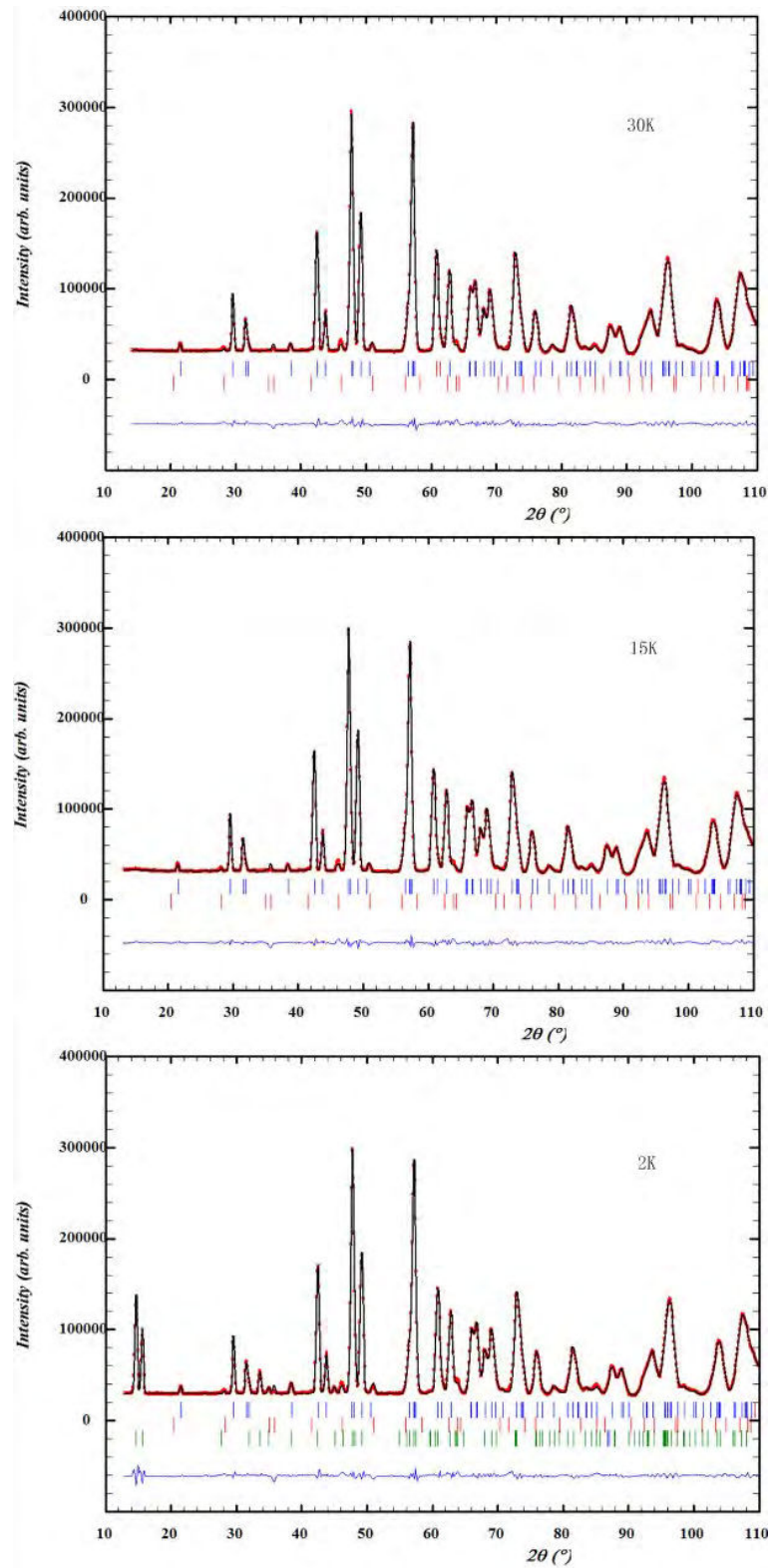
Figure 8.13: Observed (symbols) and calculated (line) powder neutron diffraction patterns for SrCoGe 2 O 6 at 30, 15 and 2K. The green tick marks shows the magnetic reflections. The nuclear reflections of the main phase are denoted by blue tick marks. The reflections marked in red belong to a Sr 3 CoGe 5 O 14 impurity phase. The blue line shows the difference between the observed and calculated diffraction patterns.
