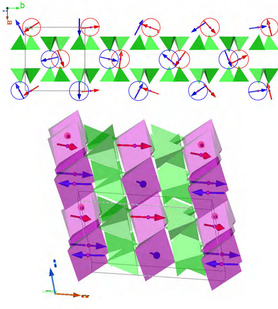
Figure 8.20: Cycloidal spiral magnetic structure of SrMnGe 2 O 6 below T_N .
