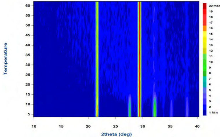
Figure 5.8: Plot of neutron powder diffraction scans showing up the magnetic transition at 15K using a wavelength of 2.52\text{\AA} .
