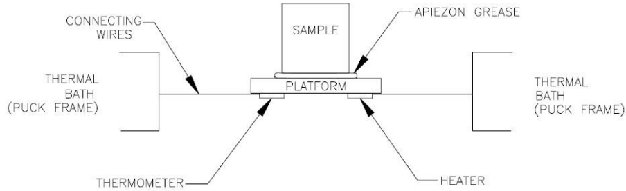
Figure 2.11: Thermal connections to sample and sample platform[12]
