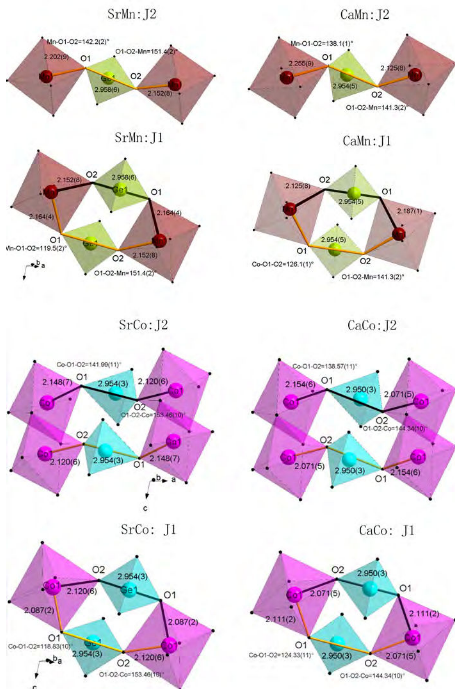
Figure 8.5: The polyhedral drawing shows the two interchain interactions J1 and J2 for SrMnGe 2 O 6 , SrCoGe 2 O 6 , CaMnGe 2 O 6 and CaCoGe 2 O 6 , respectively.
