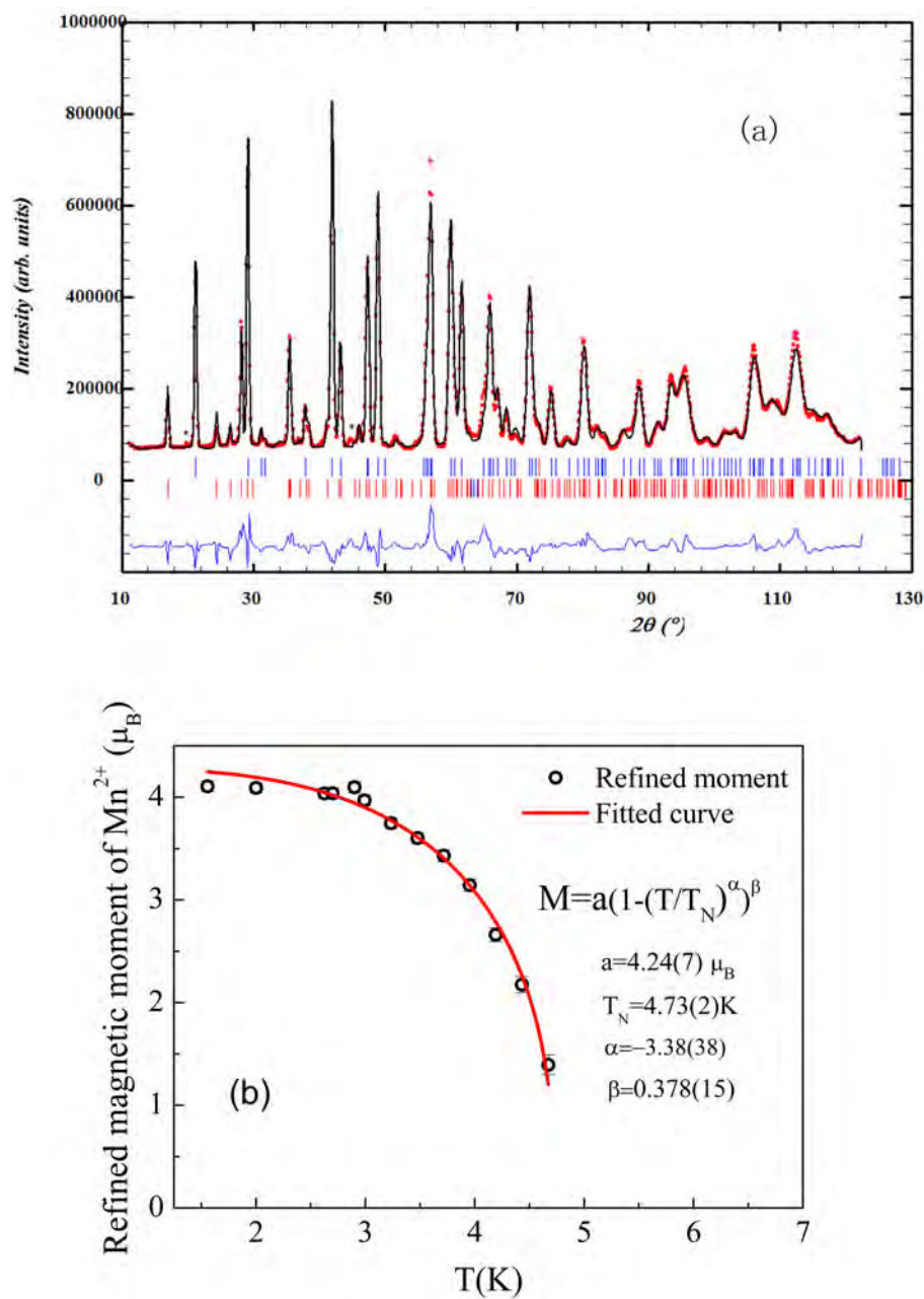
Figure 8.19: (a) Plot of refined NPD data at 2K for SrMnGe 2 O 6 . Symbols show the observed NPD pattern, and line represents the calculated one. The blue line shows the difference between them. (b) Temperature dependence of the refined Mn 2+ magnetic moments.
