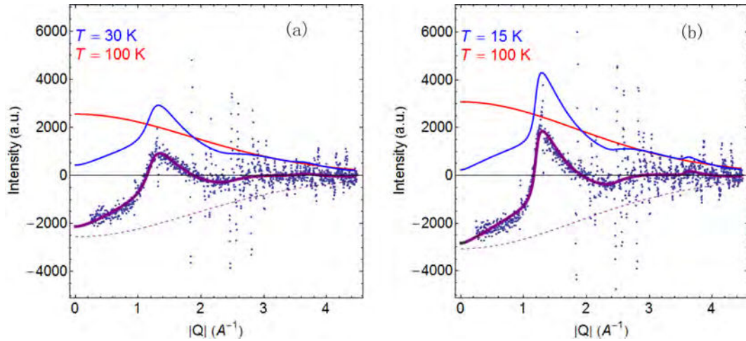
Figure 6.13: Diffuse neutron scattering by subtracting the NPD pattern at 100 K from patterns at 30 K (a) and 15K (b). The peak was well fitted by a model of 1D scattering. Red line shows the structure factor at paramagnetic regime (100K), blue line represents the simulated signal at 30K and 15K, the purple line shows the fit result to the experimental data (scatter points).
