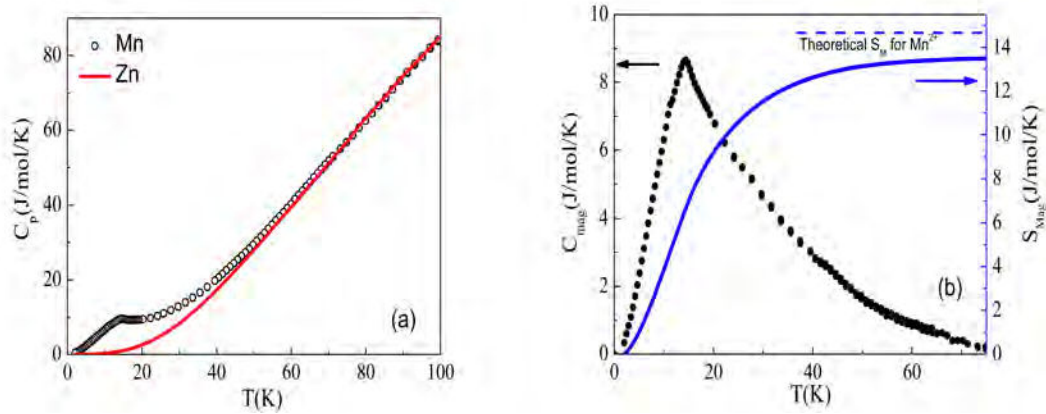
Figure 5.5: (a) Specific heat capacity of \text{CaMnGe}_2\text{O}_6 and \text{CaZnGe}_2\text{O}_6 which is used as a lattice standard. (b) (black) The magnetic component of the specific heat capacity of \text{CaMnGe}_2\text{O}_6 ; (blue) The entropy released through magnetic ordering. Blue dash line represents the theoretical maximum.
