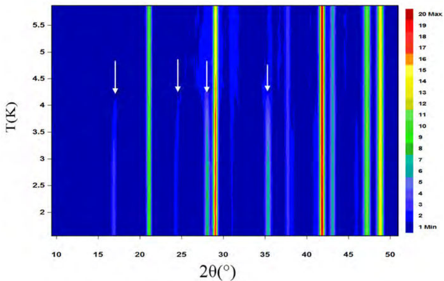
Figure 8.17: NPD patterns as a function of temperature showing a magnetic satellite reflections at 4.5K. Note: arrows mark the appearance of magnetic reflections.
