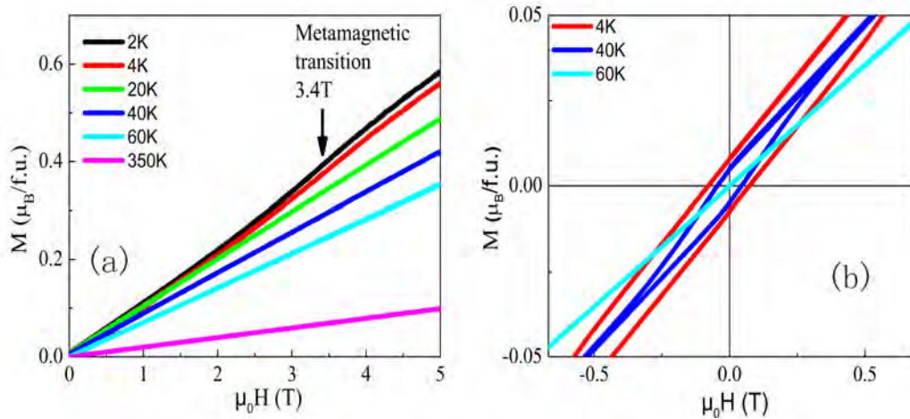
Figure 5.6: (a) Isothermal magnetization curves of \text{CaMnGe}_2\text{O}_6 collected at T = 2, 4, 20, 40, 60 and 350 K. (b) The magnetic hysteresis loops for \text{CaMnGe}_2\text{O}_6 at various temperature 4, 40 and 60 K.
