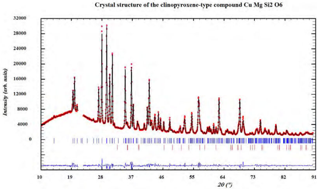
Figure 4.3: Rietveld plot for the refinement of \text{Cu}_{0.8}\text{Mg}_{1.2}\text{Si}_2\text{O}_6 from PXR data.
