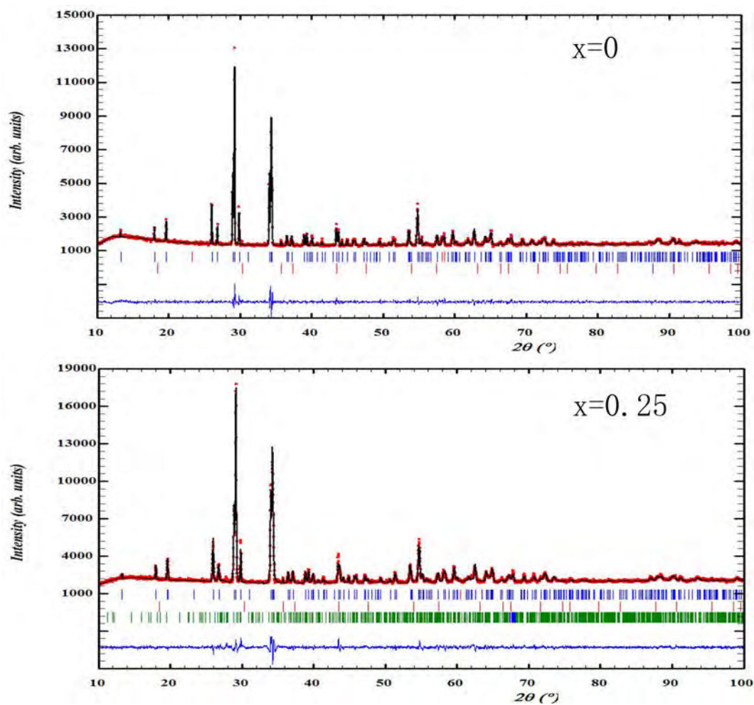
Figure 7.2: Rietveld refinement of samples with x=0 and 0.25 from XRD data taken at room temperature. Observed (red), calculated (black), and difference (blue) plots are shown. Bragg reflections are denoted by blue tick marks. The red tick marks present the Bragg reflections belong to a \text{Co}_2\text{GeO}_4 impurity phase. For sample with x=0.25 , the accommodated impurity phase \text{CaGeO}_3 during refinement is marked with green tick marks.
