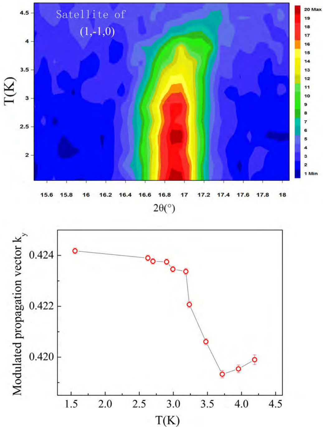
Figure 8.18: (upper) The evolution of the magnetic satellite of reflection (1,-1,0) as a function of temperature, (lower) the modulated propagation vector k_y variation of temperature refined from NPD data.
