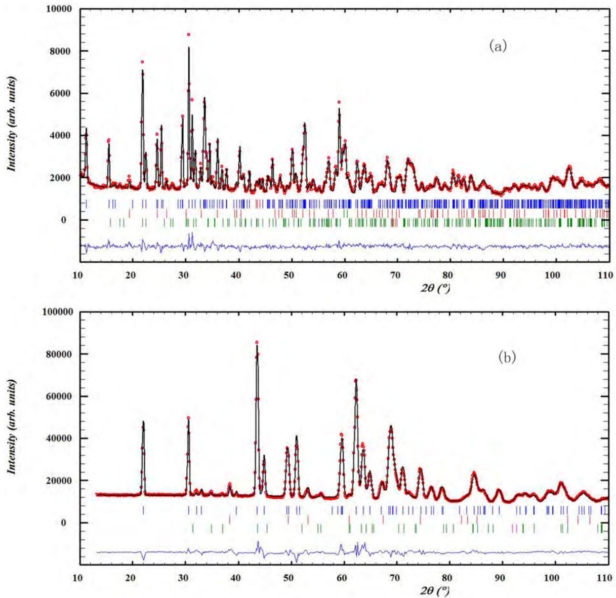
Figure 6.3: Rietveld refinement of \text{CaMnSi}_2\text{O}_6 of NPD data taken at room temperature with neutron wavelengths of 1.28 \text{ \AA} (a) and 2.52 \text{ \AA} (b). Observed (red), calculated (black), and difference (blue) plots are shown. Bragg reflections of \text{CaMnSi}_2\text{O}_6 are denoted by blue tick marks. The middle set of Bragg reflections belong to a \text{CaCO}_3 (R-3c) impurity phase, and the lowest set of tick marks denote another impurity phase \text{CaCO}_3 (Pmcn).
