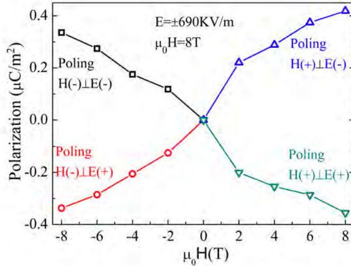
Figure 5.15: The induced electric polarization as a function of applied magnetic field with different ME annealing manners.
