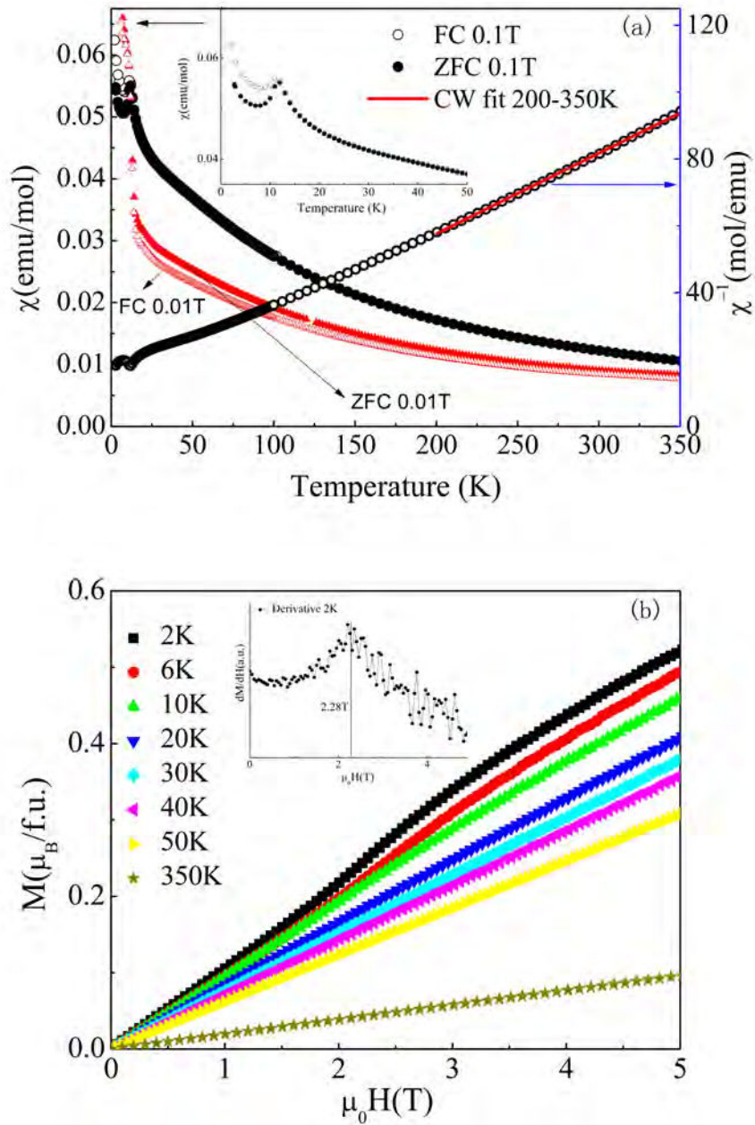
Figure 6.6: (a) Temperature dependence of the magnetic susceptibility of \text{CaMnSi}_2\text{O}_6 under magnetic fields of 0.1 and 0.01T. The Curie-Weiss fit for inverse magnetic susceptibility was presented with red solid line. Inset shows the low temperature regime. (b) Isothermal magnetization curves of \text{CaMnSi}_2\text{O}_6 between 2K and 350 K. Inset presents the dM/dH curve at 2 K, showing the magnetic field induced metamagnetic transition under magnetic field of 2.28T.
