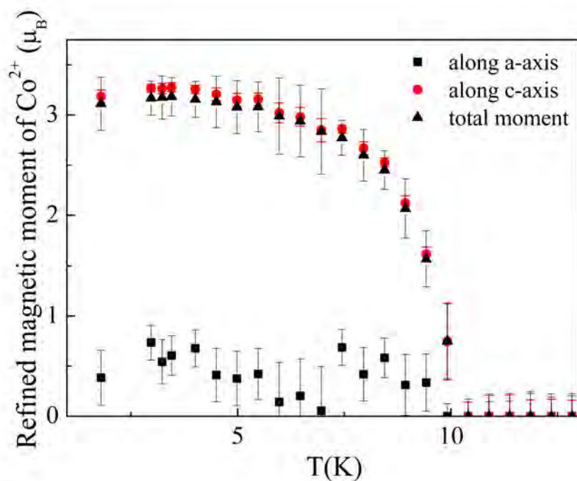
Figure 8.15: Evolution of the refined Co 2+ magnetic moment components as a function of temperature.
