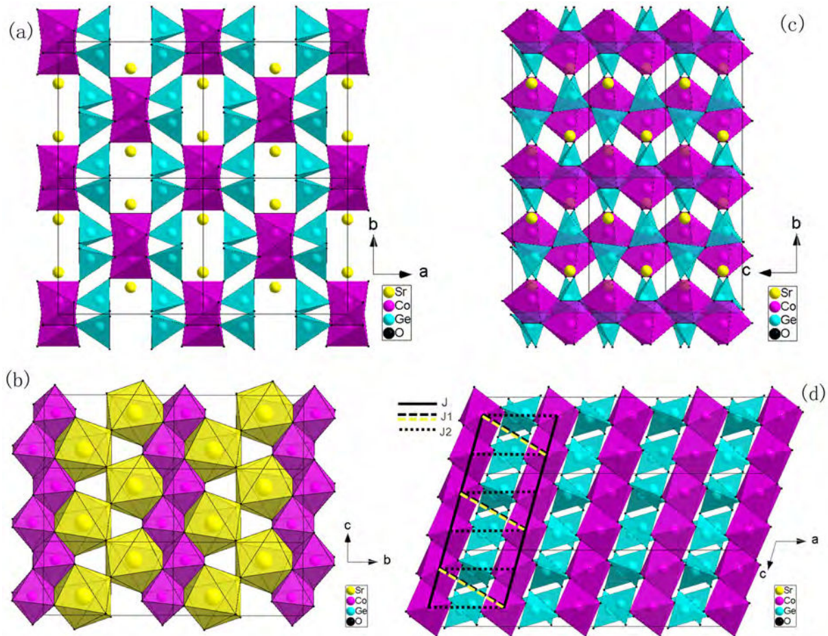
Figure 8.3: Projections of the SrCoGe 2 O 6 structure (SrMnGe 2 O 6 also shares similar manner) along different axes, derived from NPD at room temperature: (a) The alternate stacking of layers consist of CoO 6 octahedra and GeO 4 tetrahedra. (b) CoO 6 octahedra chains with zigzag characteristic and SrO 6 octahedra non-connected chains. (c) The corner-sharing GeO 4 tetrahedra chains characterized by O-rotation(close to E-chain). (d) The CoO 6 zigzag chains bridged by GeO 4 tetrahedra through O 3 -O 3 edge of each tetrahedron; three possible magnetic interaction pathways J (solid line), J 2 (dashed line) and J 1 (dotted line) are marked; note that for J 1 and J 2 , black line represents the coupling via GeO 4 tetrahedron in the back, and yellow line denotes the interaction via GeO 4 tetrahedron in the front.
