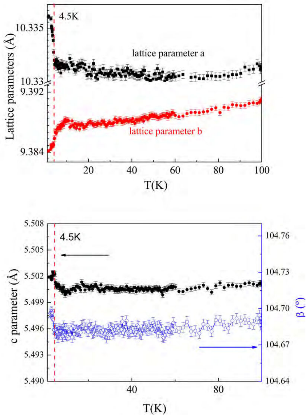
Figure 8.22: Temperature dependent lattice parameters for SrMnGe 2 O 6 .
