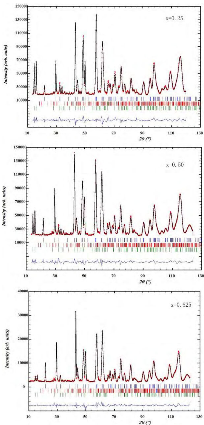
Figure 7.18: Observed (symbols) and calculated (line) powder neutron diffraction patterns for \text{CaCo}_{1-x}\text{Mn}_x\text{Ge}_2\text{O}_6 ( x=0.25, 0.5, 0.625 ) at 2 K. The green tick marks show the magnetic reflections. The nuclear reflections are denoted by blue tick marks. The reflections marked in red belong to a \text{CaGeO}_3 impurity phase. The blue line shows the difference between the observed and calculated diffraction patterns.
