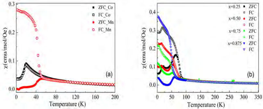
Figure 7.10: (a) Temperature dependence of the magnetic susceptibility (ZFC and FC) of \text{CaCoGe}_2\text{O}_6 and \text{CaMnGe}_2\text{O}_6 under external magnetic field with 100 Oe. (b) Temperature-dependent magnetic susceptibilities of \text{CaCo}_{1-x}\text{Mn}_x\text{Ge}_2\text{O}_6 ( x=0.25, 0.5, 0.75, 0.875 ) series measured at 100 Oe.
