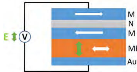
Figure 1.15: Model of storage media with electric field write and magnetic field read.
