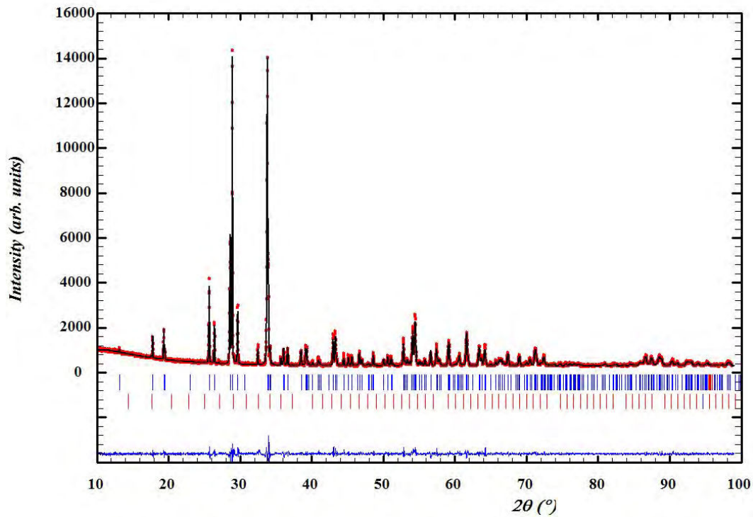
Figure 7.5: Rietveld refinement of \text{CaMnGe}_2\text{O}_6 from XRD data taken at room temperature. Observed (red), calculated (black), and difference (blue) plots are shown. Bragg reflections are denoted by blue tick marks. The lower set of Bragg reflections belong to a \text{Ca}_3\text{Mn}_2\text{Ge}_3\text{O}_{12} impurity phase.
