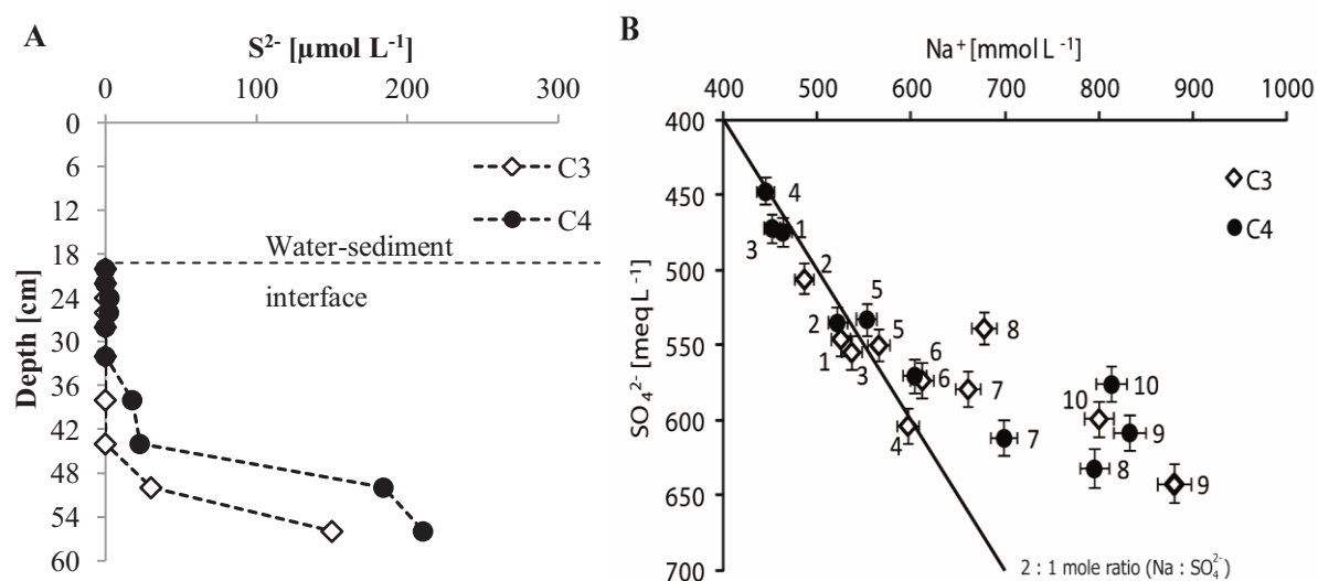
Figure V-10: Evolution of the dissolved \text{S}^{2-} concentration (A) and the \text{SO}_4^{2-} vs. Na concentrations (B) in the porewater of the sediment layers in columns C3 and C4.
