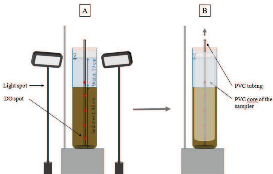
Figure V-1: Schematics of the constructed Winogradsky columns with the position of the dissolved oxygen spots (A), and the sampling set-up consisting of a PVC tube and a PVC support (B).
