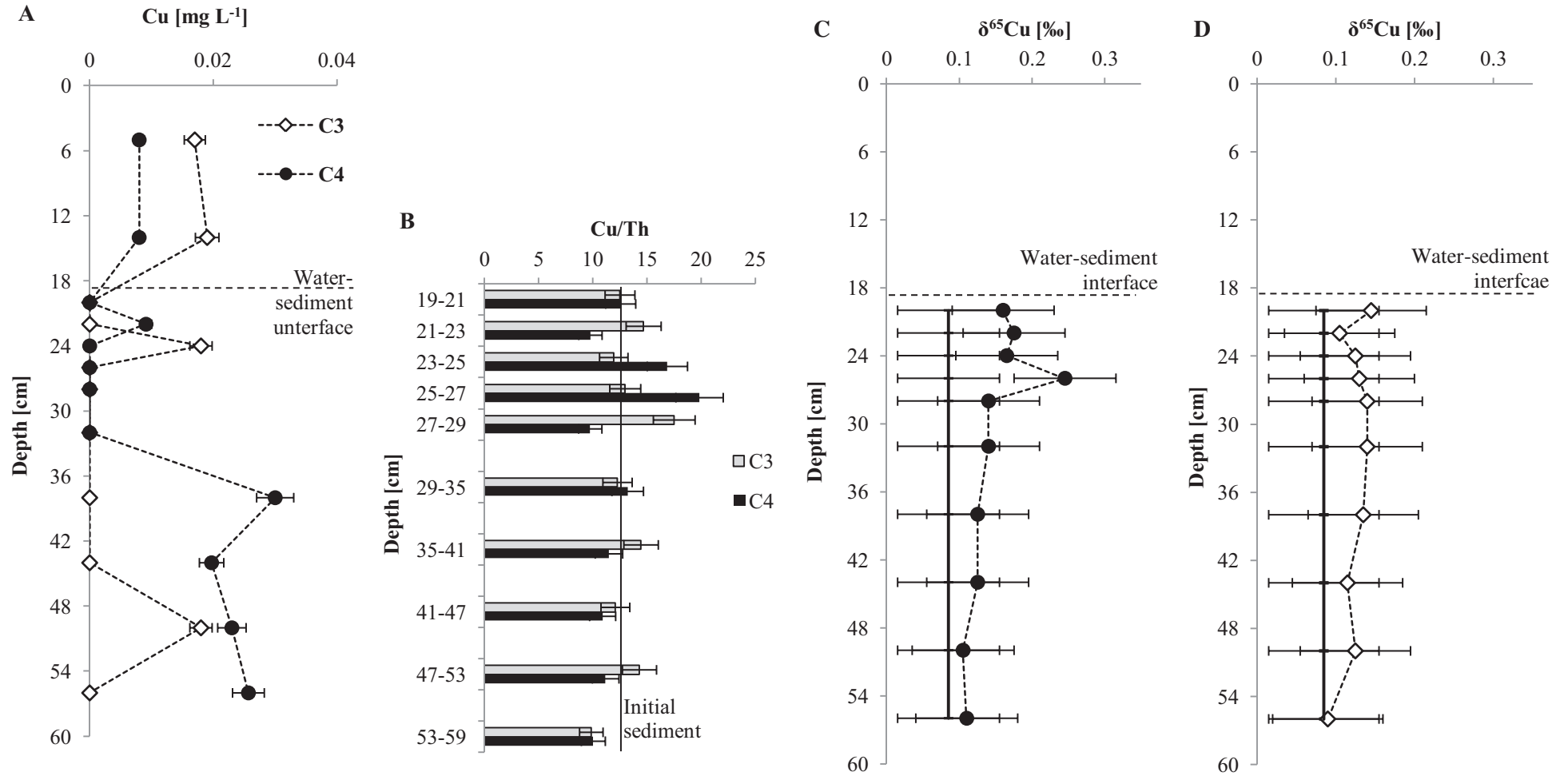
Figure V-14: Depth profiles of Cu concentrations in the porewater of the columns C3 and C4 (A), Th normalized Cu concentrations (B), and the \delta^{65}\text{Cu} of the sediment-bound Cu in the columns C4 (C) and C3 (D) compared to \delta^{65}\text{Cu} of the initial sediment. Error bars denote the 2s of the Cu isotope measurements of the geological standards ( \pm 0.07\text{‰} , n=15 ).
