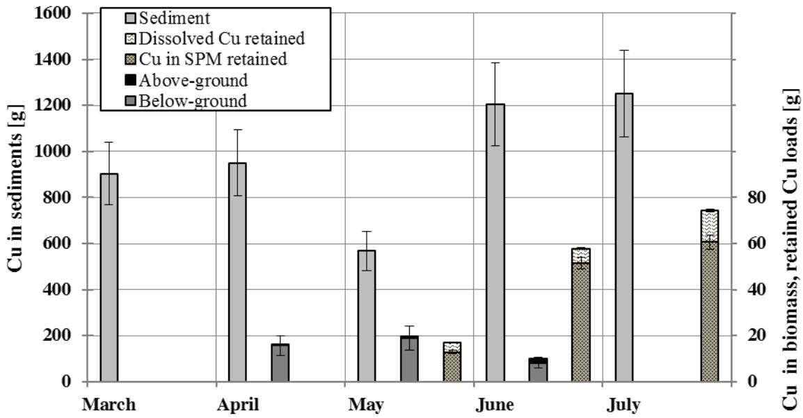
Figure IV-S1: Estimated Cu stocks in wetland sediments, wetland vegetation (above- and below-ground stocks) and dissolved Cu and Cu in suspended particulate matter (SPM) retained by the wetland. Error bars account for the reproducibility of Cu measurements in replicates (n=2).
