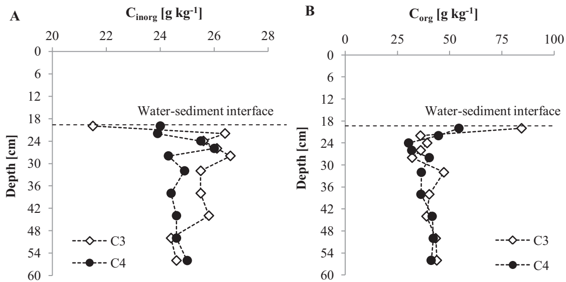
Figure V-2: Sediment-bound inorganic (A) and organic (B) carbon concentrations along the depth profile of columns C3 and C4.
