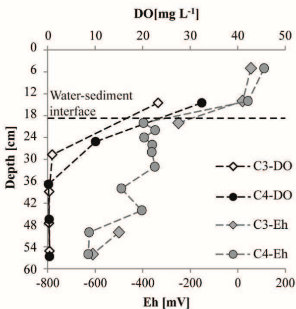
Figure V-4: Dissolved oxygen (DO) concentration and the redox potential (Eh) in the columns C3 and C4 (due to inconsistent values in the C3 Eh is not displayed between 19 and 48 cm depth).
