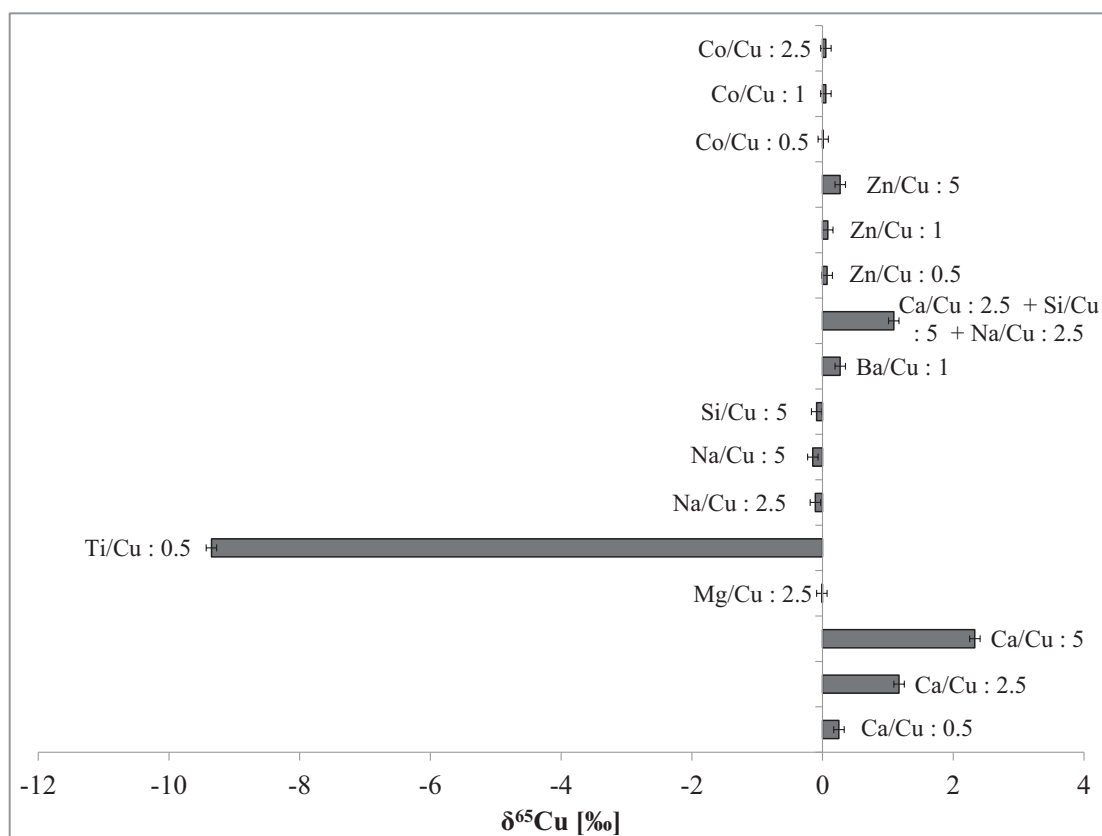
Figure II-9: Test of the spectral interferences caused by the spiking of the Cu standard with matrix elements that might be present in purified samples following a single purification.
