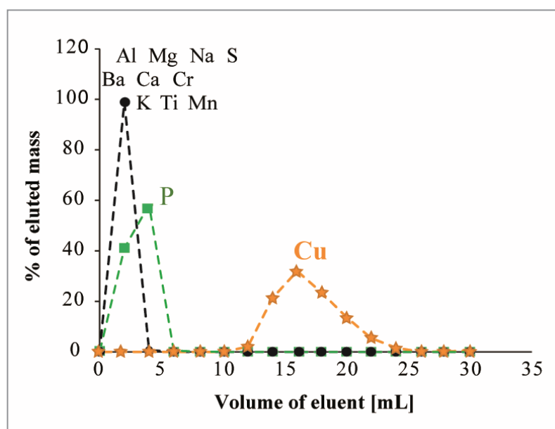
Figure II-5: Cu elution curve of the plant samples using 2 mL AGMP1.
