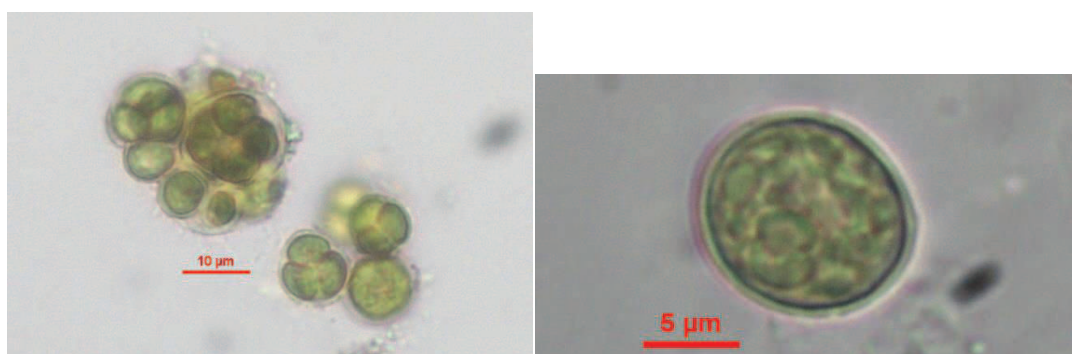
Figure V-5: Colonial and unicellular forms of Tetracystis/Chlorococcum sp.
