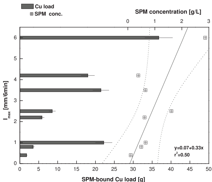
Figure III-8: The export of SPM and SPM-bound Cu loads in runoff collected at the outlet of the vineyard catchment (Rouffach, France) as influenced by the rainfall intensity.
