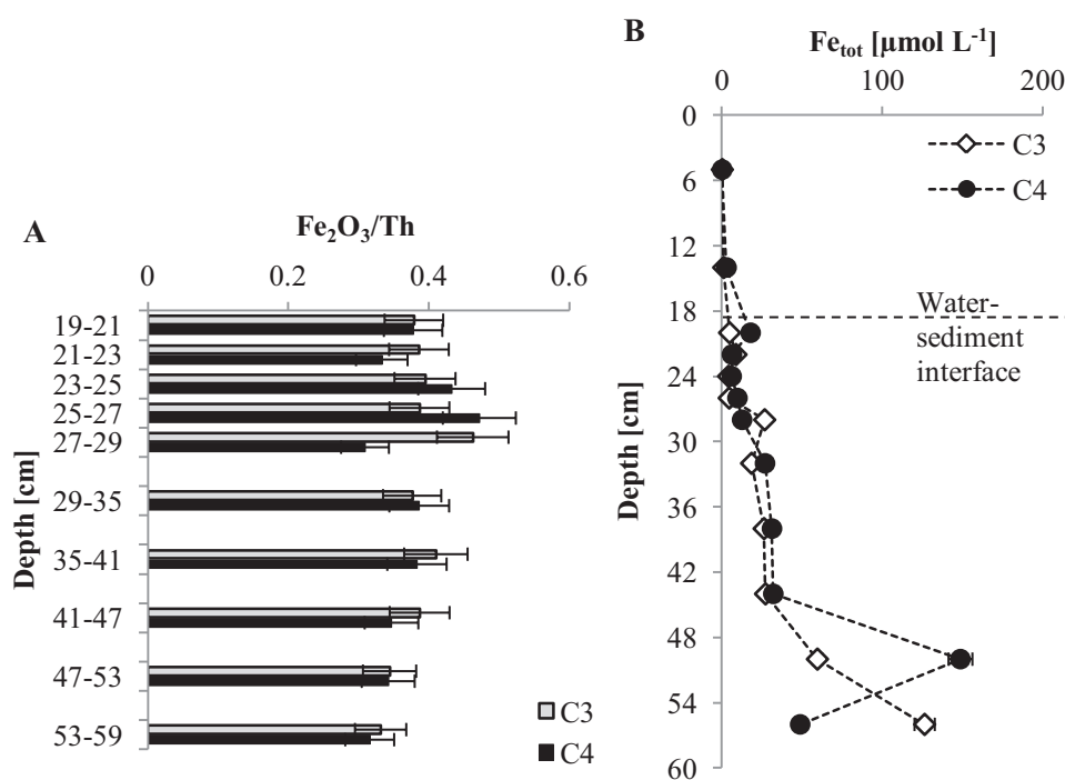
Figure V-7: The Th normalized Fe concentrations in the sediment layers (A) and Fe tot concentrations in the overlying and the porewater (B) of the columns C3 and C4.
