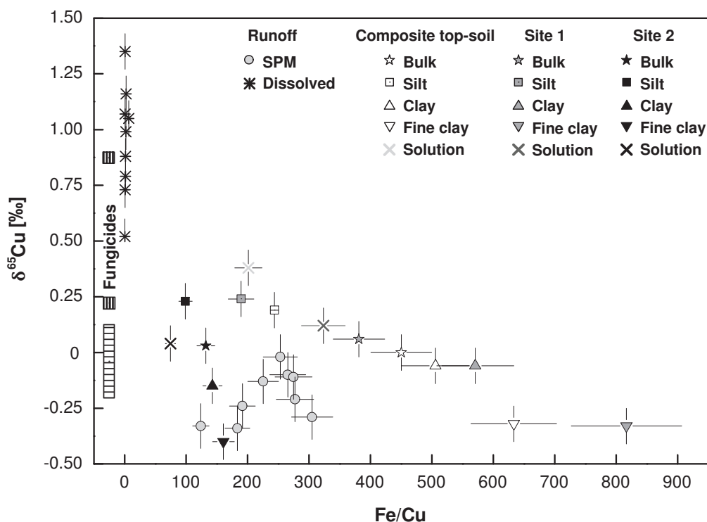
Figure III-5: \delta^{65}\text{Cu} values of the SPM-bound and dissolved Cu in runoff collected at the outlet of the catchment (Rouffach, France). The soil fractions of a composite top-soil and the surface soils at the two sites in weeded inter-rows are also displayed as a function of the Fe/Cu molar ratios. The vertical bars represent the range of \delta^{65}\text{Cu} values of the Cu-fungicides applied in 2011 (horizontal hatching) and not applied in 2011 (vertical hatching). Note that the difference between site 1 and 2 is in the Cu concentrations of the soils (Fe concentrations are similar).
