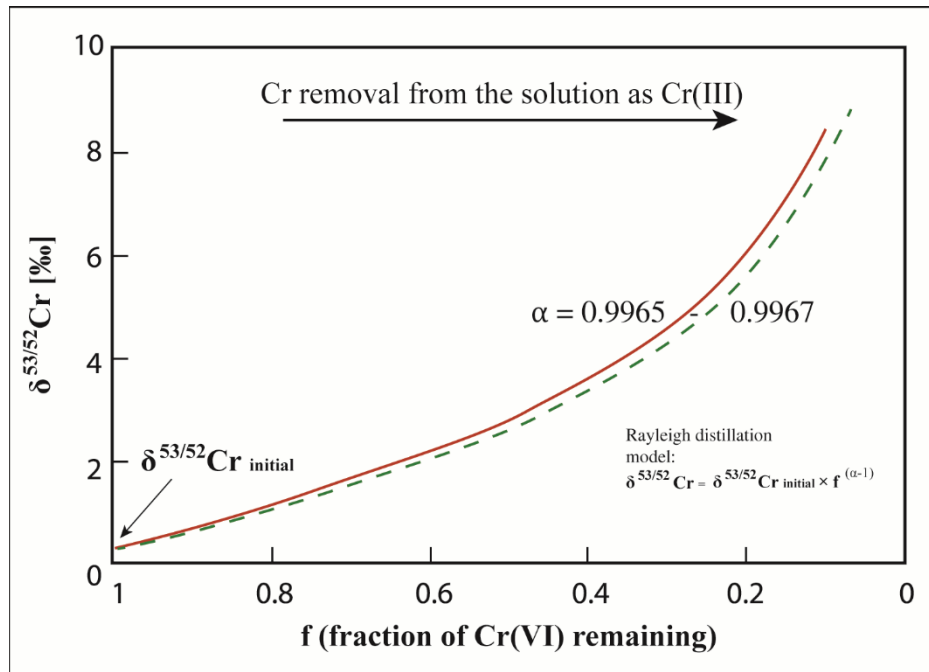
Figure I-5: Cr(VI) reduction leads to the removal of Cr from groundwater as insoluble Cr(III). The Rayleigh distillation model fits the Cr isotope fractionation produced by the Cr reduction by different reducing agents (magnetite, sediment). (Figure modified from Ellis et al. 2002). 95
