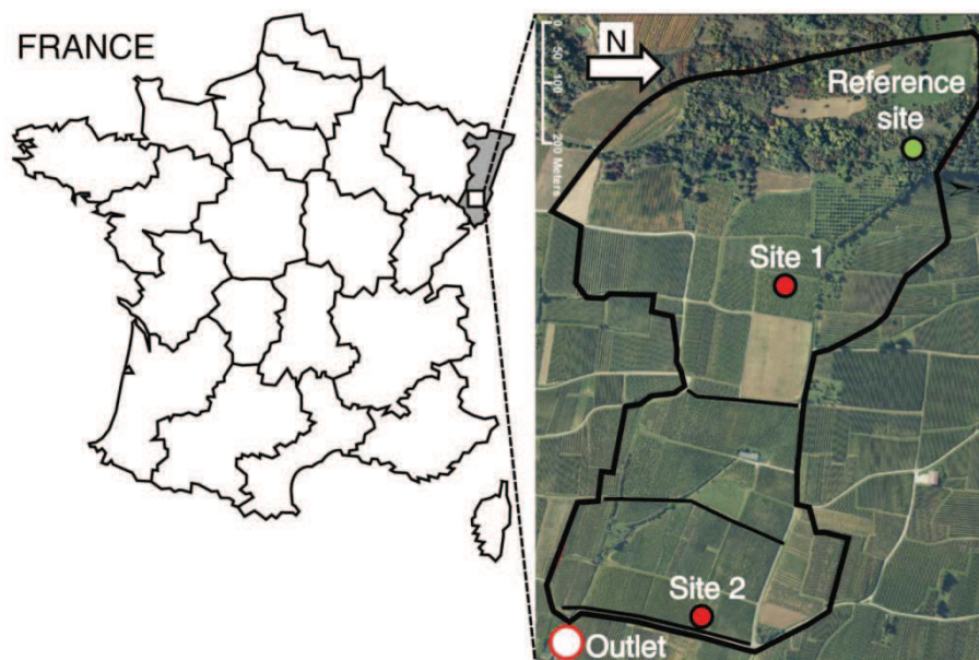
Figure III-1: The map of the study site (Rouffach, Alsace, France) with the sampling sites and the outlet displayed. The composite topsoils were collected along the three displayed transects.
