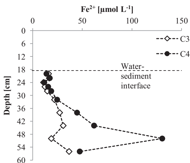
Figure V-8: Ferrous iron ( Fe^{2+} ) concentrations in the porewater of the sediment layers in the columns C3 and C4. Fe^{2+} is produced by the reductive dissolution of Fe^{3+} . Fe^{2+} was not analyzed in the overlying water.
