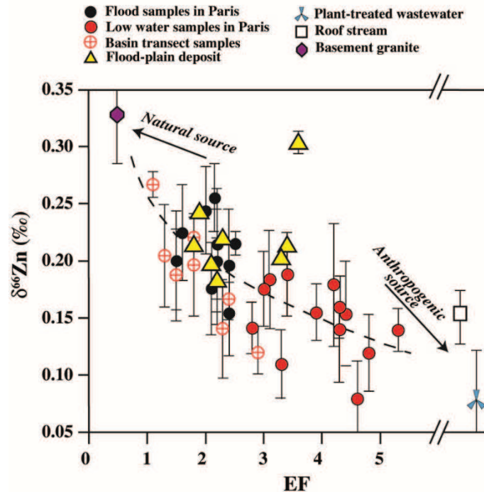
Figure I-6: Zn isotope ratios versus Zn enrichment factors (EF) showing the relative contribution of the two end-members to the Zn load in the suspended sediments in the Seine river. The end-members are the natural geogenic Zn (granites) and the anthropogenic Zn from the wastewater treatment plant and the roof runoff. (Figure from Chen et al. 2009). 92
