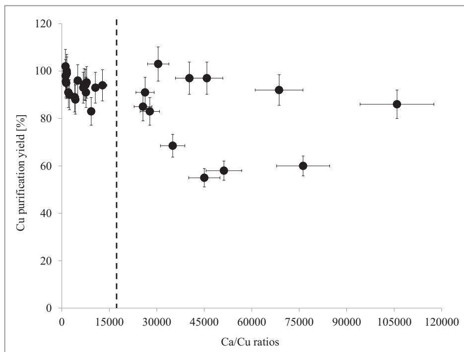
Figure II-7: The Cu purification yield performed on the water samples from Rouffach as a function of the Ca to Cu concentration ratios.
