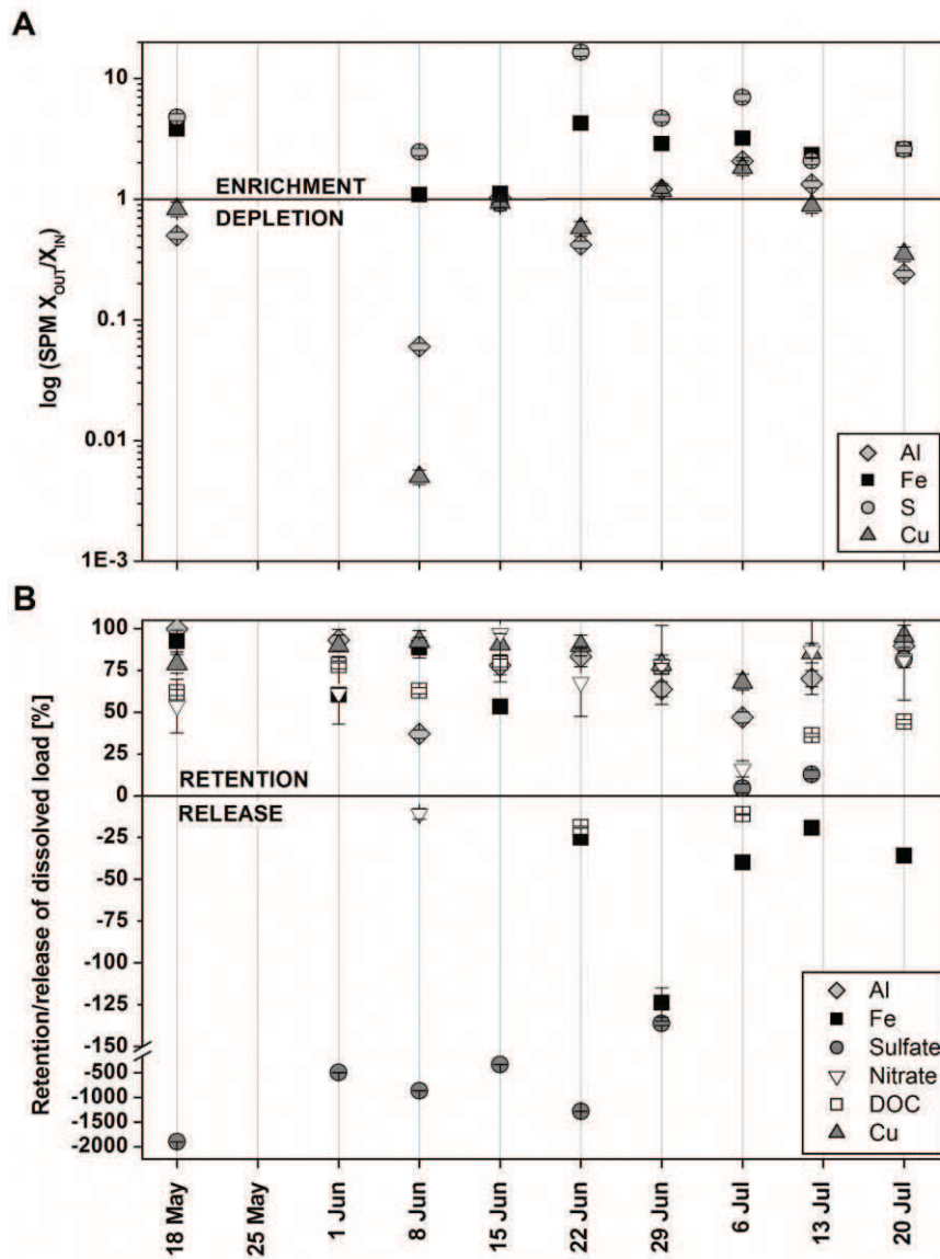
Figure IV-3: Transport of Al, Fe, Cu, S, sulfate, nitrate and dissolved organic carbon (DOC) in the stormwater wetland. Outlet/inlet ratios of elemental concentrations in suspended particulate matter (SPM) (A) and retention or release of dissolved load in the wetland (B). The errors bars given for the ratios were calculated via error propagation and incorporates analytical uncertainties of concentration measurements of elements and chemical species.
