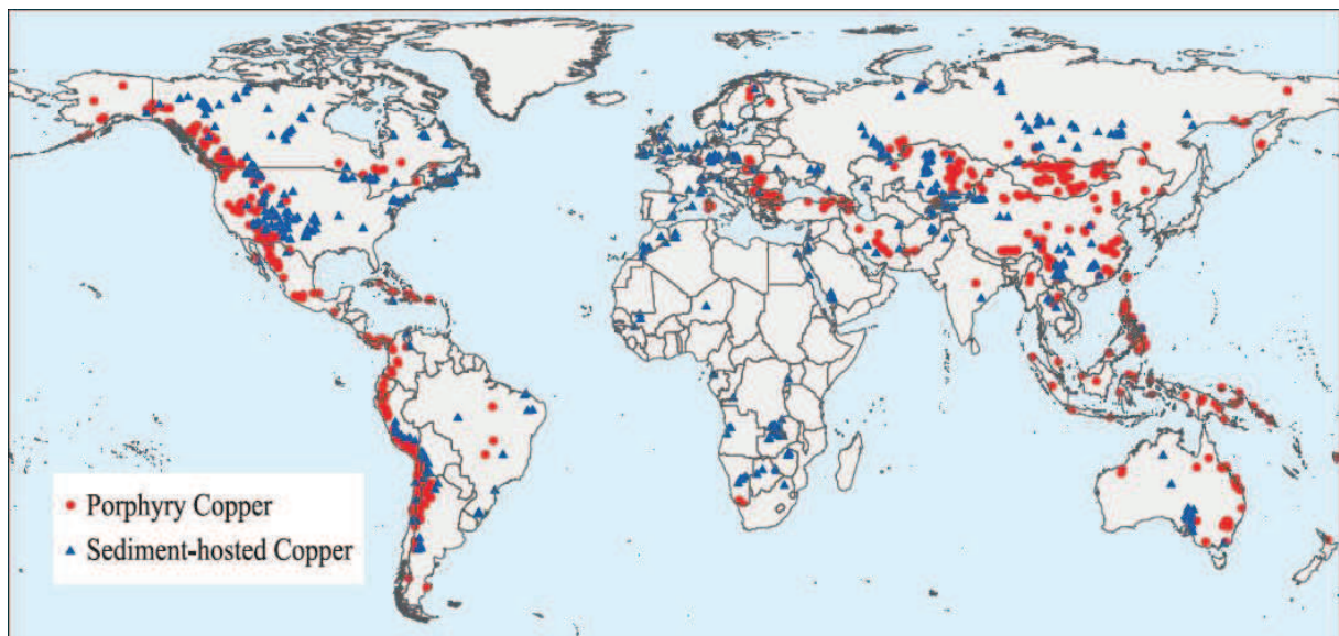
Figure I-2: Distribution of known Cu deposits in 2008. Red dots indicate Cu associated with igneous intrusions (porphyry Cu deposits) and blue dots indicate Cu contained in sedimentary rocks (sediment-hosted Cu deposits). (Map prepared by the US Geological Survey) 37
