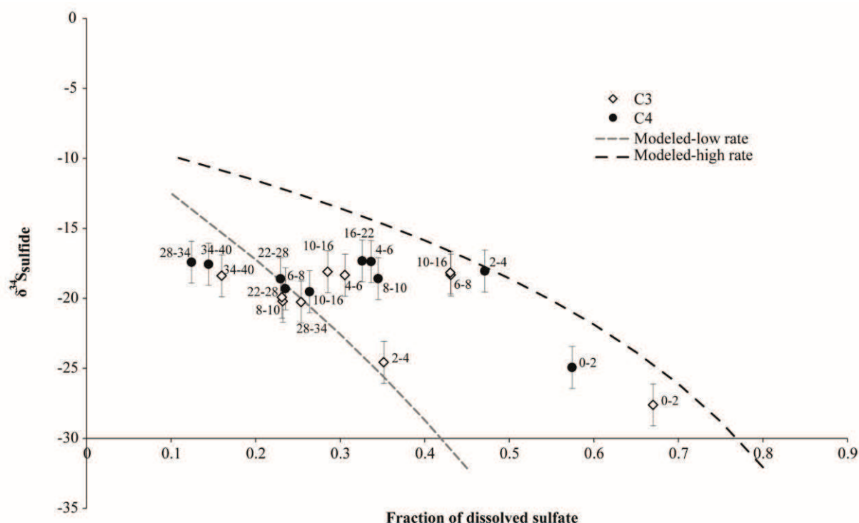
Figure V-17: Theoretical and observed \delta^{34}\text{S} values of reduced sulfides in the column sediments for low and high rates of sulfate reduction. The depth of the layers is displayed close to the symbol (in cm below the WSI).
