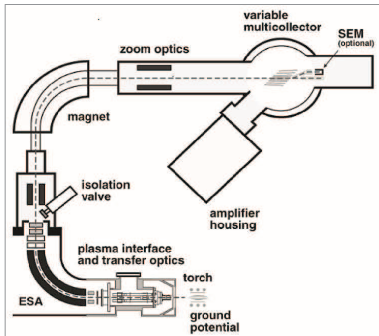
Figure II-8: The schematic image of a double focusing multicollector ICP-MS (ESA: Electric sector analyzer (Figure from Goldstein and Stirling, 2003)). 36
