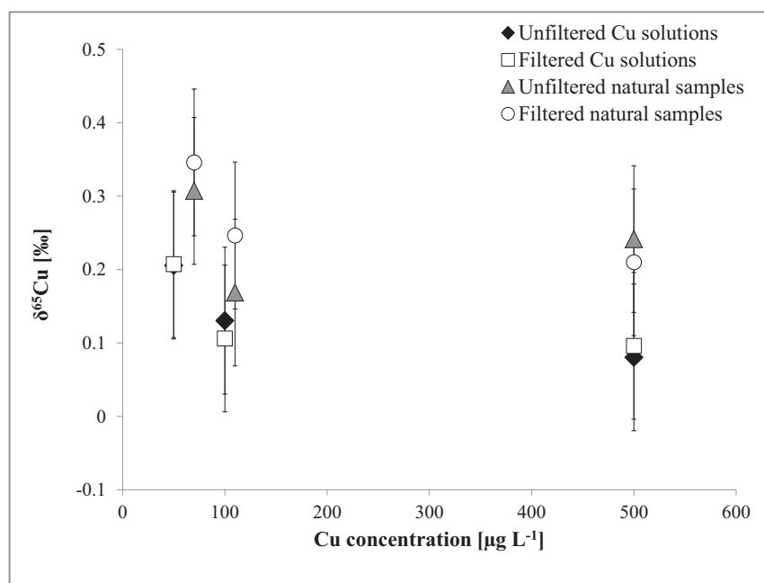
Figure II-2: Cu isotope ratios of unfiltered and filtered Cu solutions and natural samples added with Cu at different concentrations.
