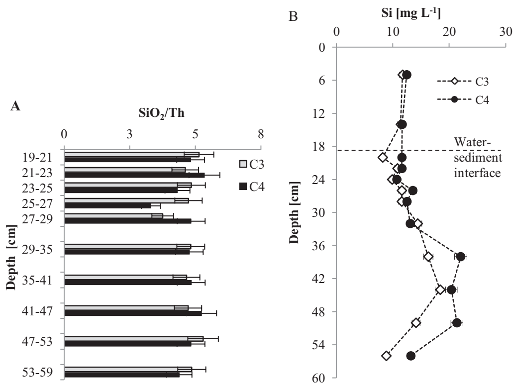
Figure V-12: The Th normalized Si concentrations in the sediment layers (A) and Si concentrations in the overlying and the porewater (B) of the columns C3 and C4.
