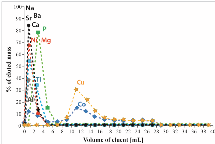
Figure II-4: Elution discretization of a soil sample (50 mg) using 3 mL resin AGPM1.
