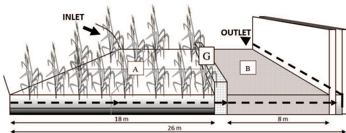
Figure IV-2: Scheme of the constructed stormwater wetland (Rouffach, France, year of construction 2002). The wetland is composed of a vegetated forebay (A) and the gravel filter (B), separated by a gabion barrier (G), a box filled with rocks whose role is to enhance the dispersion of water ahead of the gravel filter.
