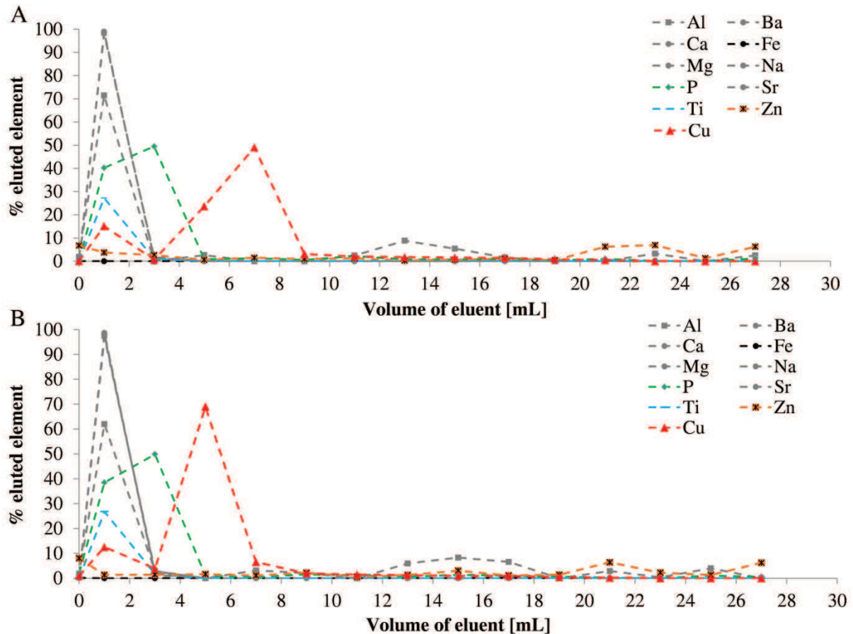
Figure II-6: Elution of Cu and matrix components of the selected "critical" wetland water sample concentrated 100 times (A) and 130 times (B).
