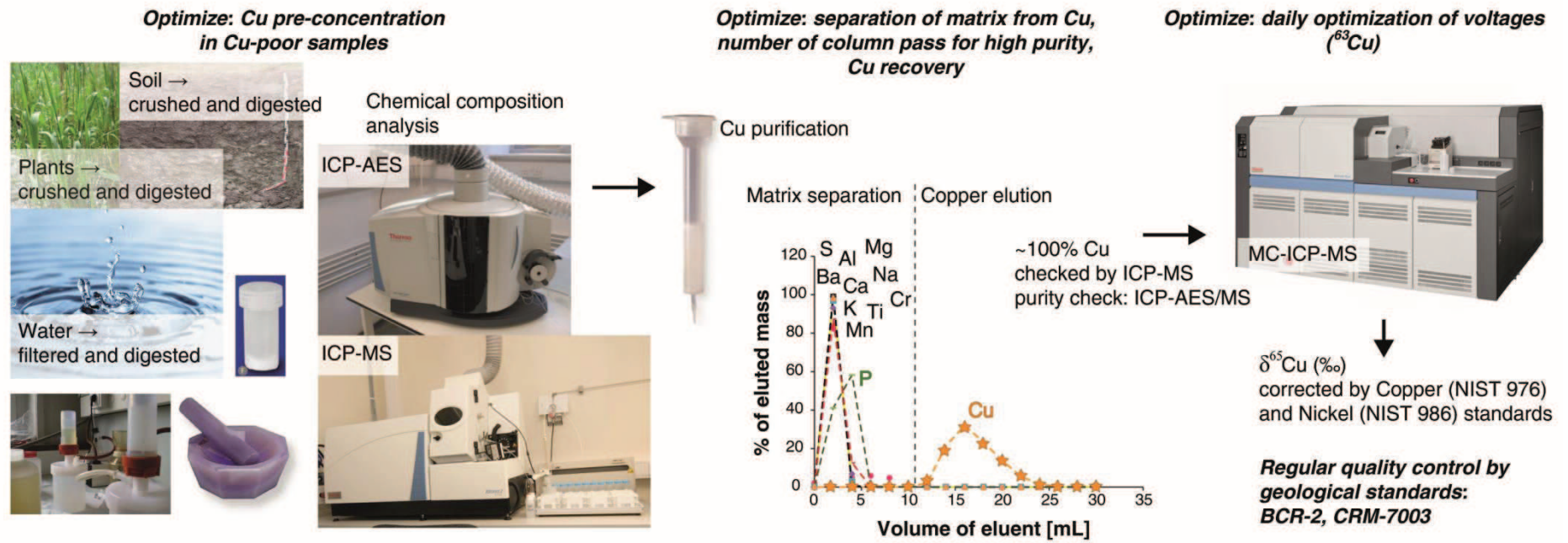
Figure II-1: Schematic of the different steps of the methodology applied and adapted in this thesis to measure Cu isotope ratios in soil, sediment, vegetal, and water samples.
