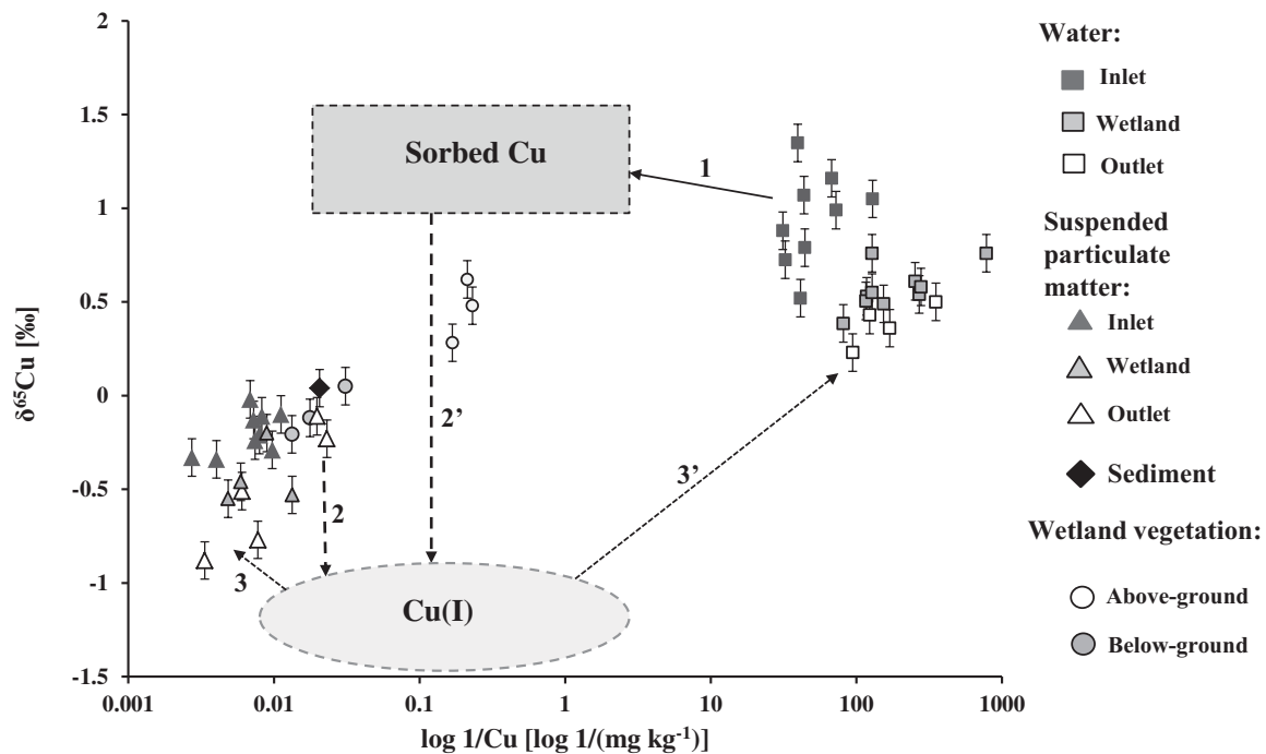
Figure IV-4: Conceptual model of Cu transport and transformation in the wetland. 1) Sorption of dissolved Cu to the sediment and enrichment in ^{65}\text{Cu} of the sorbate, 2+2') Reduction of Cu(II) within the sediment of the sorbed (2') and retained particulate (2) Cu forming an isotopically lighter Cu(I) pool, 3+3') Contribution of the isotopically lighter Cu(I) to Cu associated with the dissolved phase (3') and SPM (3) outflowing the wetland under high-flow conditions.
