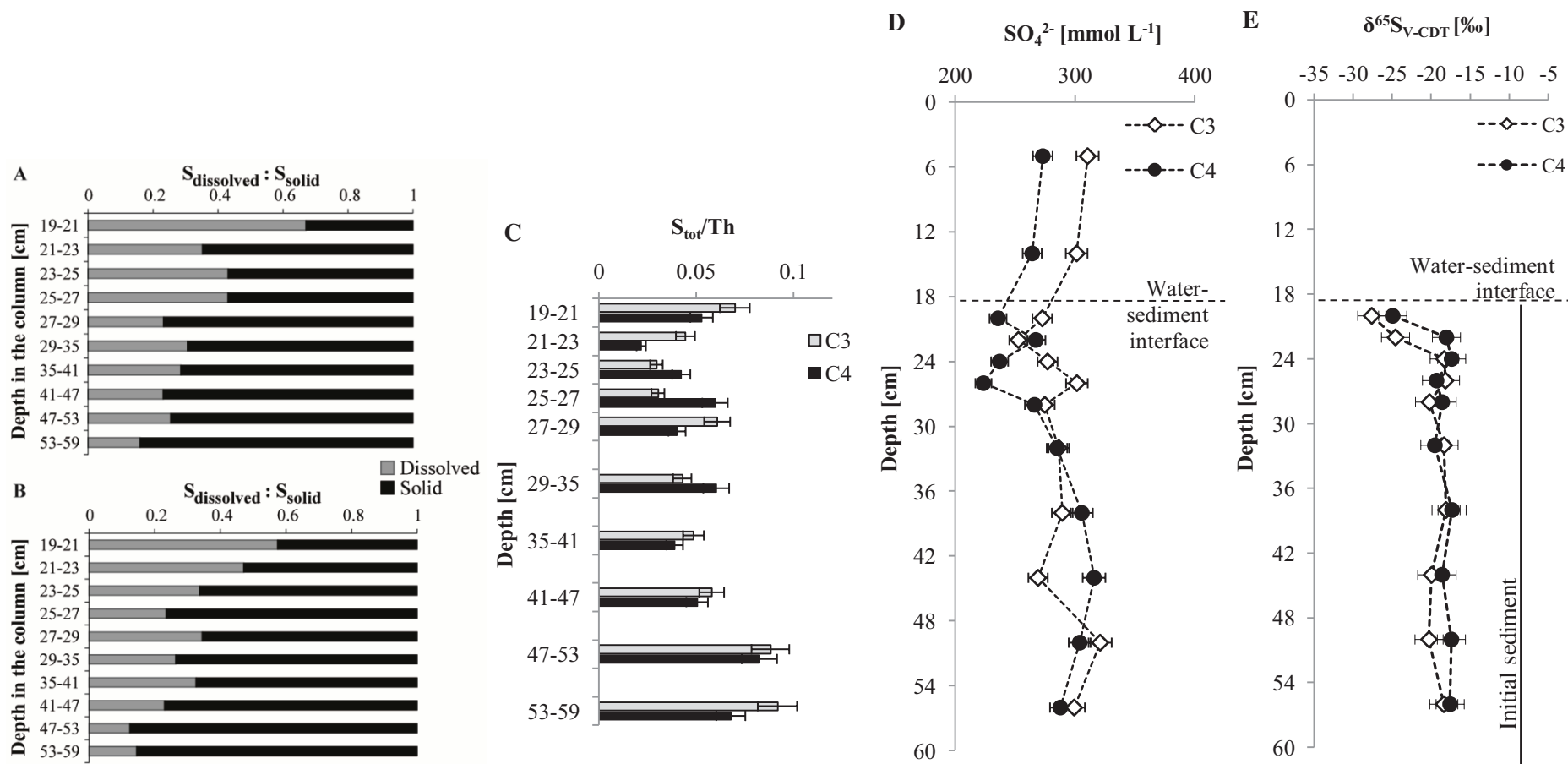
Figure V-11: Total sulfur partitioning between the porewater and the sediment phases in C3 (A) and C4 (B), Th normalized S_{tot} concentrations in the sediment layers (C), and SO_4^{2-} concentrations in the overlying water and the porewater (D), sulfur isotope ratios in the sediment phase compared to the sulfur isotope ratio in the initial sediment (E).
