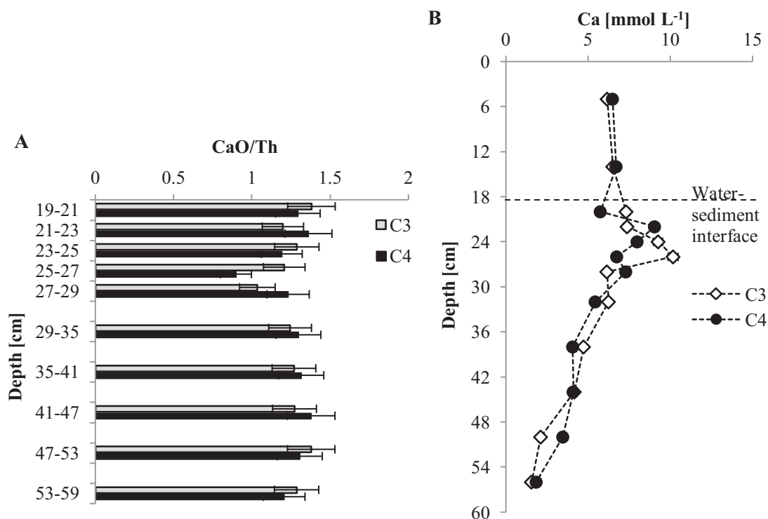
Figure V-13: Th normalized Ca concentrations in the sediment (A) and Ca concentrations in the overlying and the porewater (B) of the columns C3 and C4.
