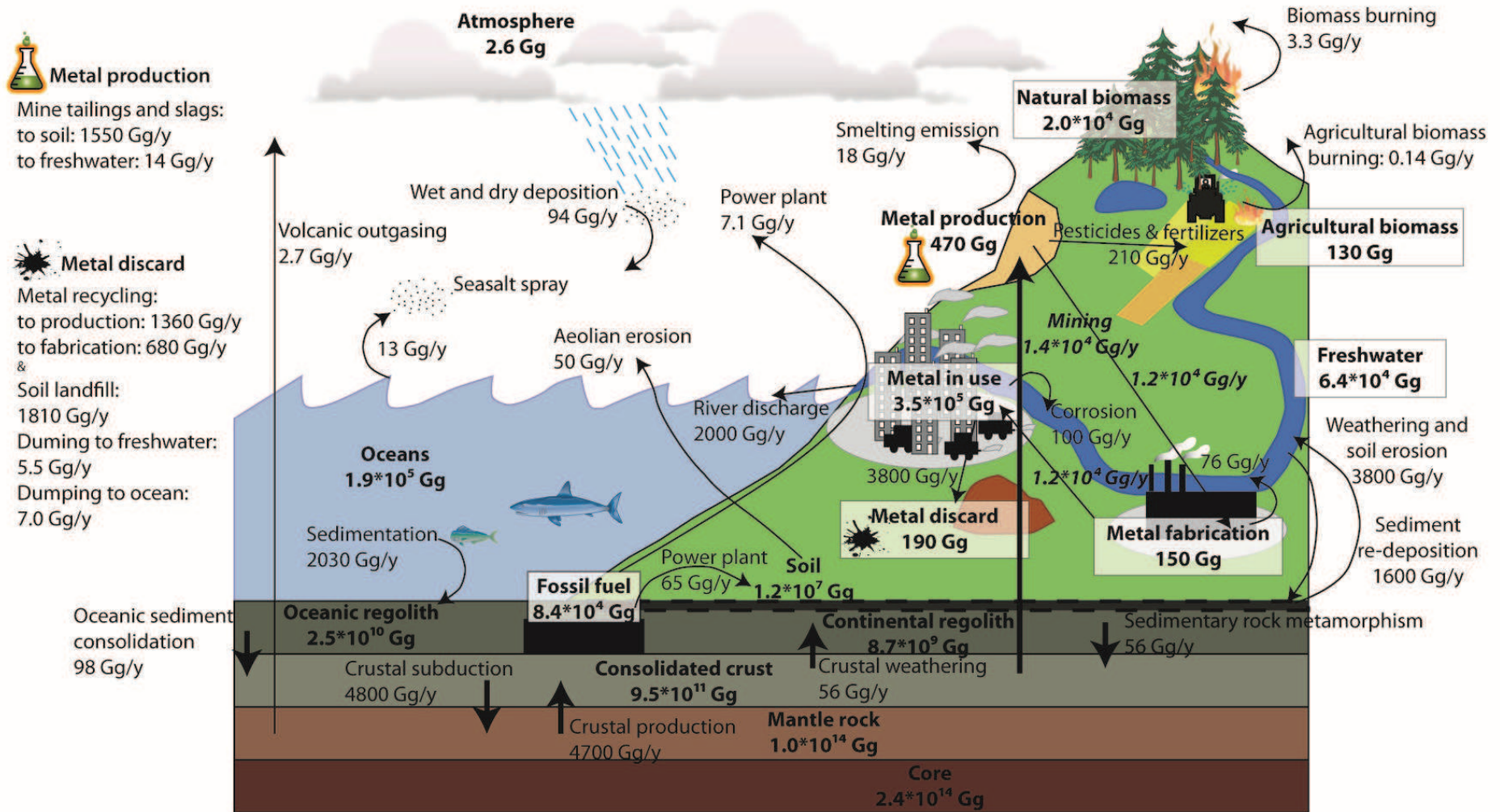
Figure I-1: The global cycle of Cu (Figure based on data in Rauch and Graendel, 2007). 1
