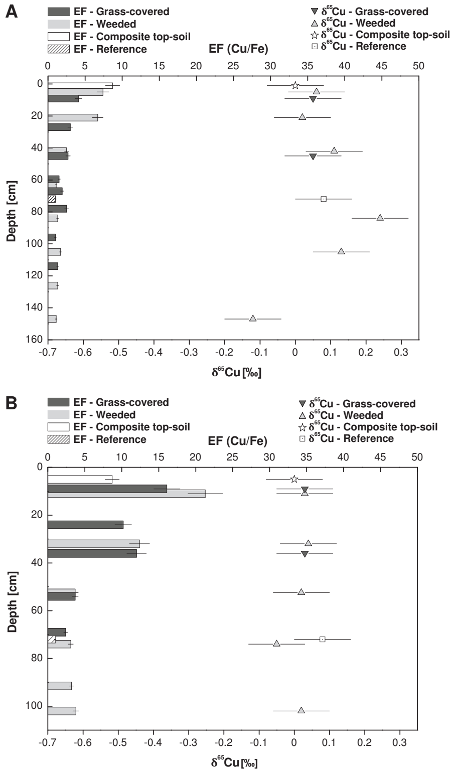
Figure III-4: Enrichment factor of Cu (EF) and \delta^{65}\text{Cu} values in the soil depth profiles at site 1 (A) and site 2 (B) of the vineyard catchment (Rouffach, France). The deepest soil horizon (67-77 cm) at an uncultivated reference site and the composite top-soil (0-5 cm) are also shown.
