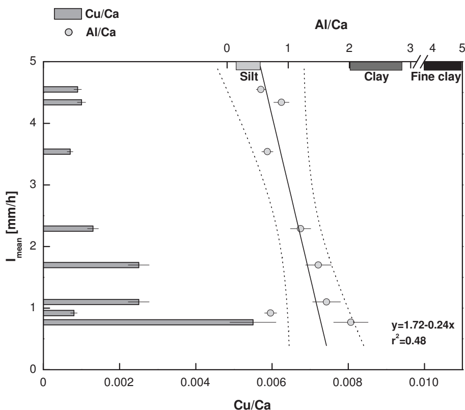
Figure III-6: Weekly mean rainfall intensity as a function of the Ca normalized Cu concentrations and Al to Ca molar ratios of the SPM in runoff at the outlet of the vineyard catchment (Rouffach, France). Error bars correspond to the propagated analytical uncertainties.
