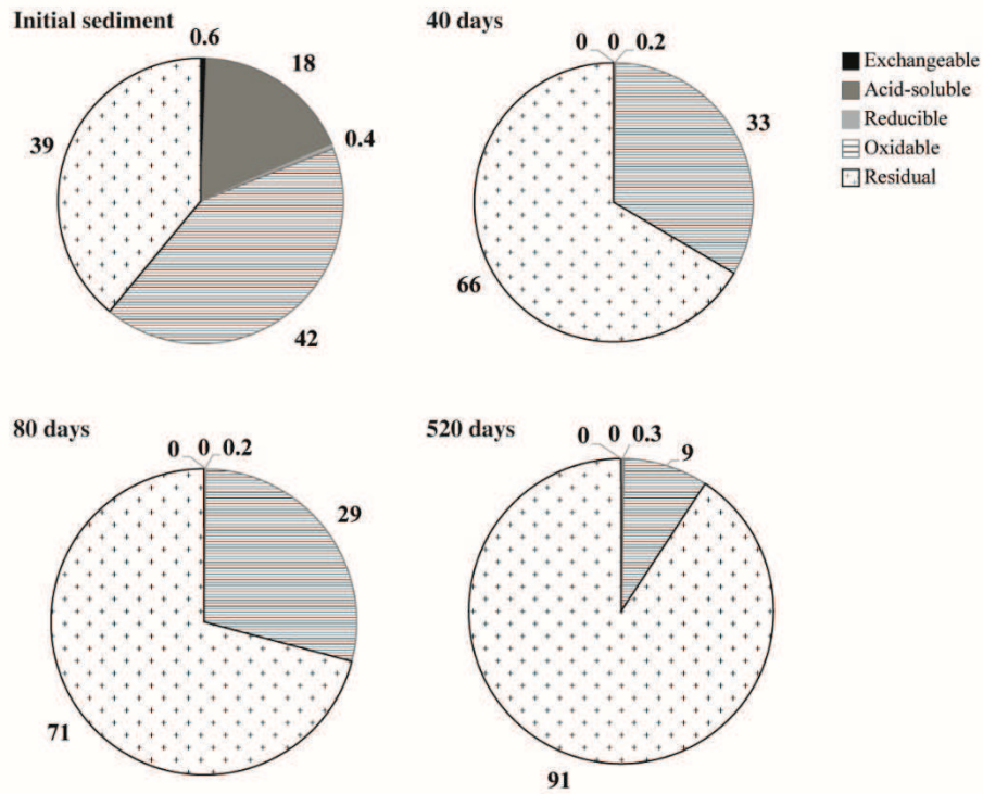
Figure V-15: Temporal changes in the Cu partitioning using sequential chemical extractions of the initial sediment, after 40 days, 80 days and 520 days.
