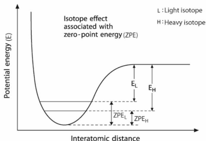
Figure I-4: Schematic potential energy curve for the interaction of two atoms in a stable molecule (Figure modified from Hoefs, 2009).
