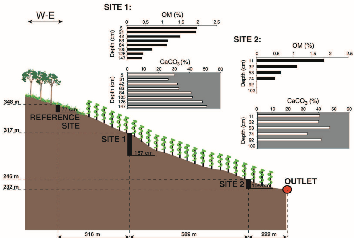
Figure III-2: Schematic of the vineyard catchment at Rouffach (Alsace, France), showing the soil sampling locations (1 and 2) and the reference site, as well as the runoff sampling at the outlet of the catchment. The altitudes of the sampling sites and their distance from each other are also displayed. The depth variations of the carbonate (CaCO 3 ) and the organic matter (OM) contents in the soil under weeded inter-rows at the two sampling sites are also shown.
