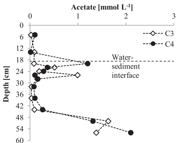
Figure V-3: Acetate concentration profile in the porewater of the sediment layers in the columns C3 and C4. Acetate is considered as the most important fermentation acid produced by the degradation of organic matter under anaerobic conditions. 28
