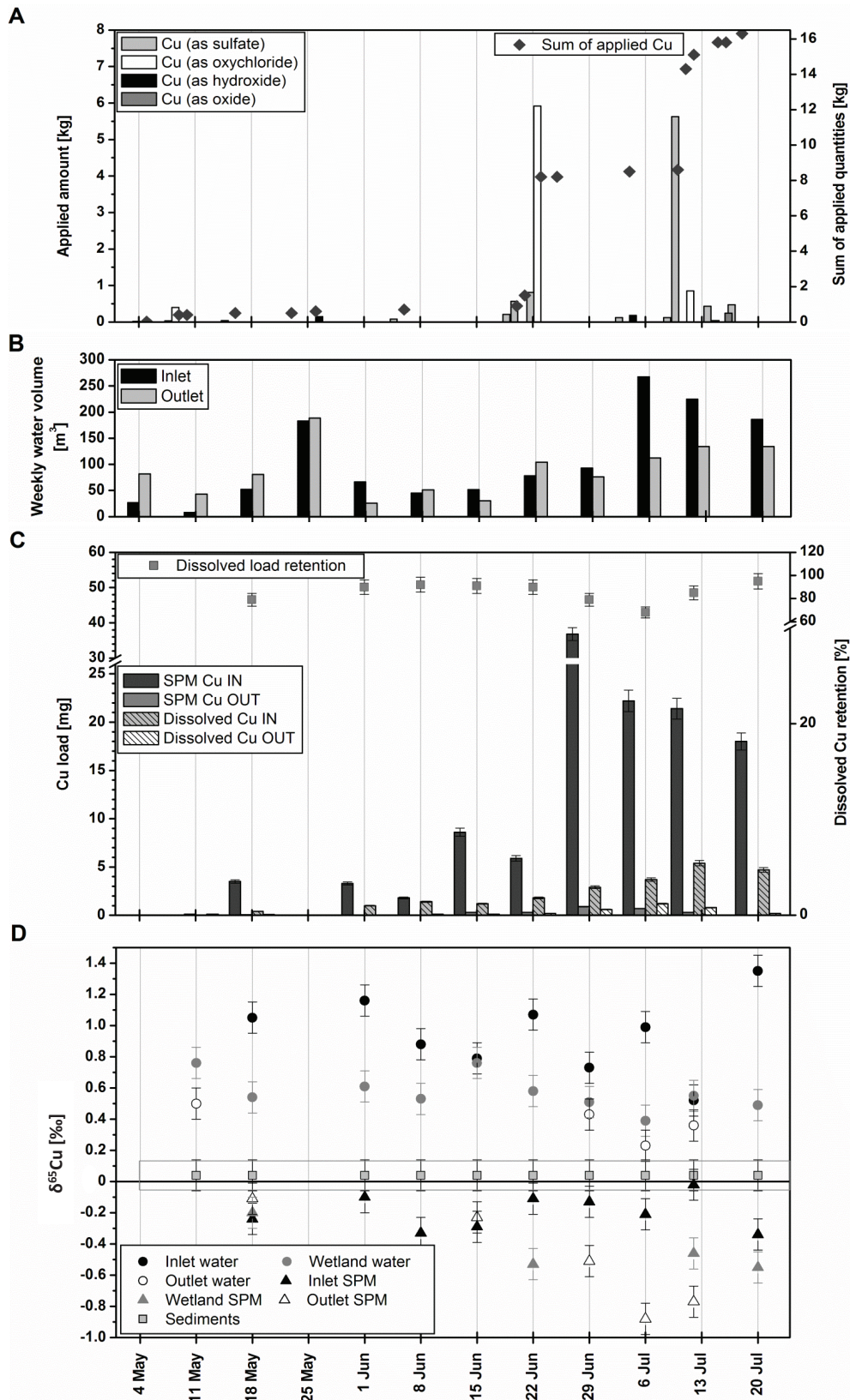
Figure IV-1: Use of Cu-based fungicides (in terms of metallic Cu) (A) and temporal change of hydrological conditions (B), Cu loads (C) and \delta^{65}\text{Cu} values (D) at the stormwater wetland (Rouffach, France) from May 4 to July 20 2011. The horizontal bar in figure D represents the \delta^{65}\text{Cu} of sediments-bound Cu. Error bars correspond to the total analytical uncertainty ( \pm 0.10 ‰, n=3 for \delta^{65}\text{Cu} measurements).
