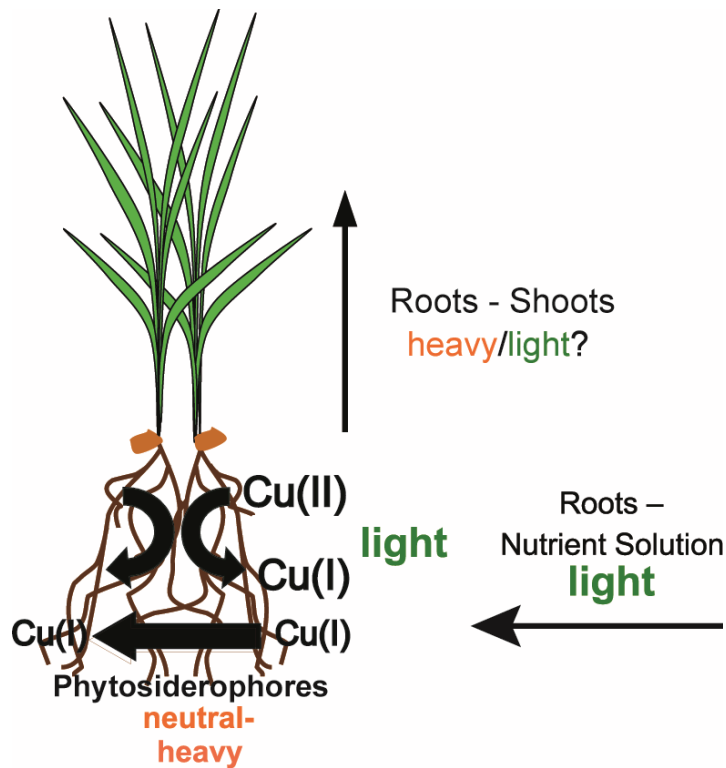
Figure I-8: Cu isotopes to study Cu uptake and translocation mechanisms by plants (Figure modified from Jouvin et al., 2012). 99
