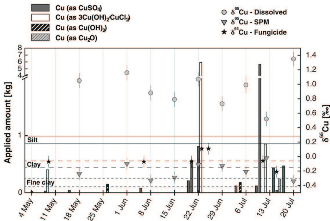
Figure III-3: Cu amounts and δ 65 Cu of the applied Cu fungicides and δ 65 Cu of runoff-associated Cu in the dissolved and the SPM-bound phases from May 11 to July 20 (Rouffach, France). A runoff sample could not be collected on May 25. Horizontal bars represent the δ 65 Cu range in the soil size fractions in the catchment (i.e. silt, clay, “fine clay”). Error bars correspond to the reproducibility of the Cu isotope measurements evaluated on geological reference materials (± 0.08‰).
