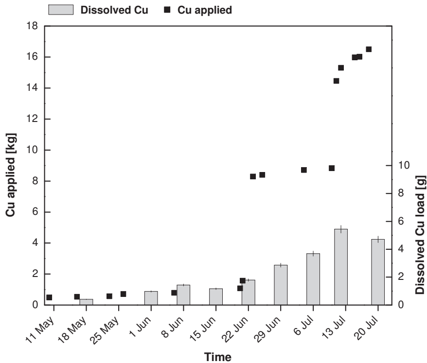
Figure III-7: The relationship between Cu fungicide applications (cumulated) and weekly dissolved Cu loads in runoff collected at the outlet of the vineyard catchment (Rouffach, France).
