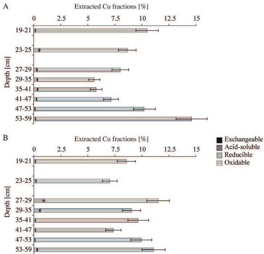
Figure V-16: Spatial changes in the geochemical partitioning of Cu using sequential chemical extractions in the columns C3 (A) and C4 (B). The residual Cu fraction accounts for the difference between the sum of all extractable Cu fractions and total Cu in the sediment and is not represented.
