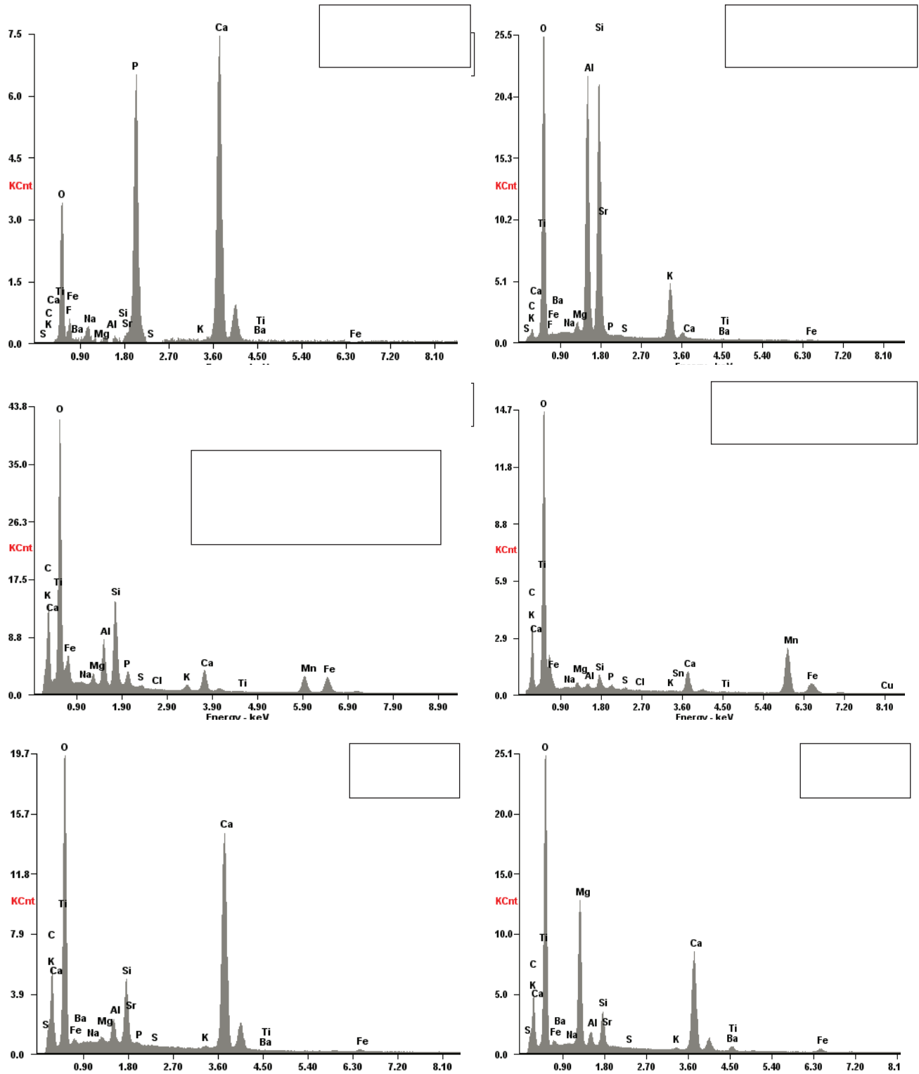
Figure IV-S2: EDS spectra of mineral and organic particles in SPM at the stormwater wetland (Rouffach, France) on July 20 2011.
