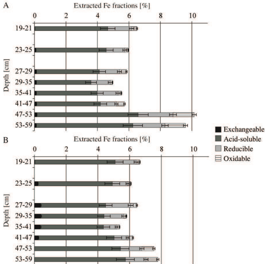
Figure V-9: Partitioning of extractable Fe phases (exchangeable, acid-soluble, reducible, oxidable) in the sediment layers of the columns C3 (A) and C4 (B) the residual Fe fraction accounts for the difference between the sum of all extractable Fe fractions and total Fe in the sediment and is not represented.
