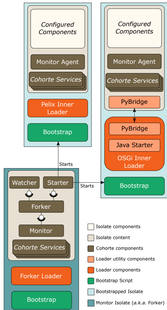
FIGURE 5.1 – Vue globale de Cohorte Runtime
