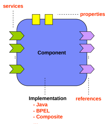
FIGURE 2.4 – Composant SCA
