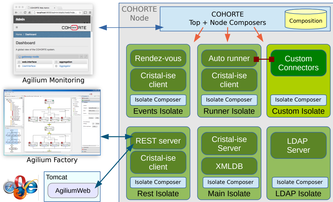
FIGURE 7.1 – Vue globale d’Agilium NG
