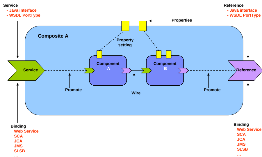
FIGURE 2.5 – Composite SCA
