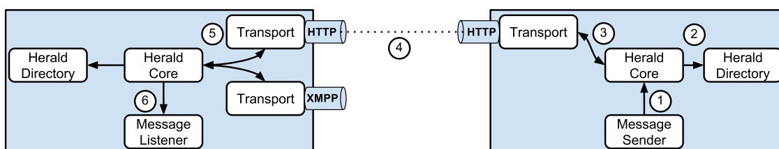
FIGURE 4.3 – Transmission de message Herald
