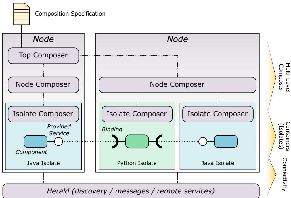
FIGURE 6.1 – Vue globale de Cohorte Composer
