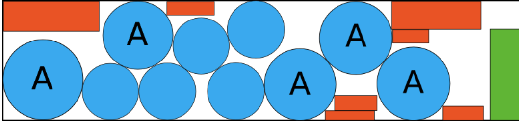
Figure 5.4 – A valid loading plan. Shapes in blue are stacks, those marked A should be alternated. Shapes in orange are side tires. And the shape in green is a tail end. (top view)
