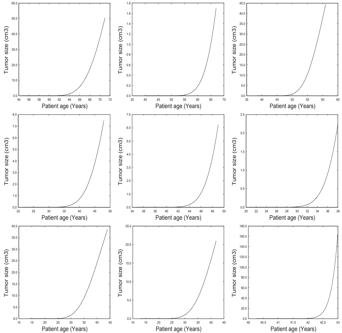
Figure A.4: First method of fit: evolution of tumor volume in time. From upper left to bottom right: patient 1 till patient 9.
