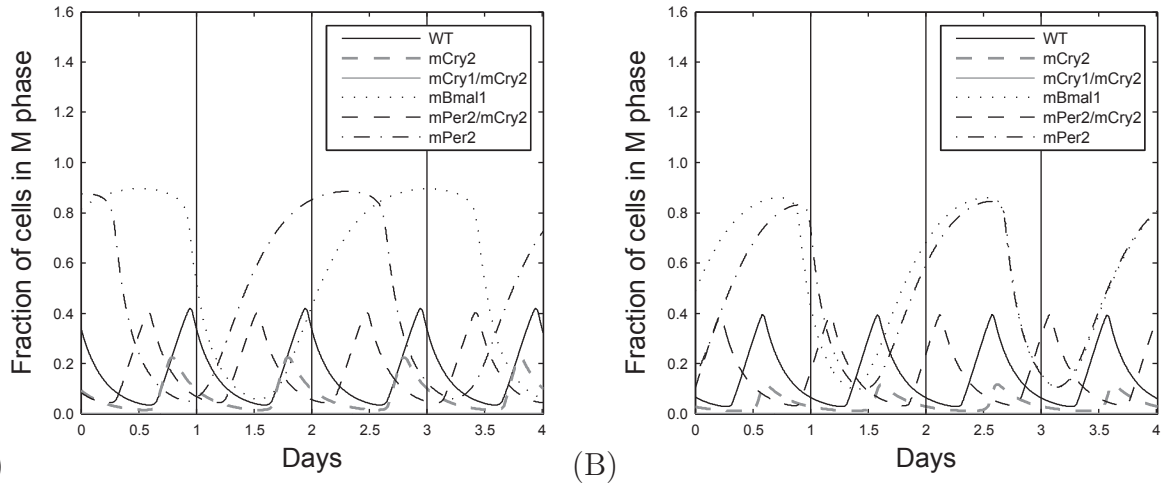
Figure 2.6: Effects of mutating circadian genes on the fraction of cells entering mitosis. (A) Autonomous period of the cell cycle is equal to 28 h. (B) Autonomous period of the cell cycle is equal to 20 h.
