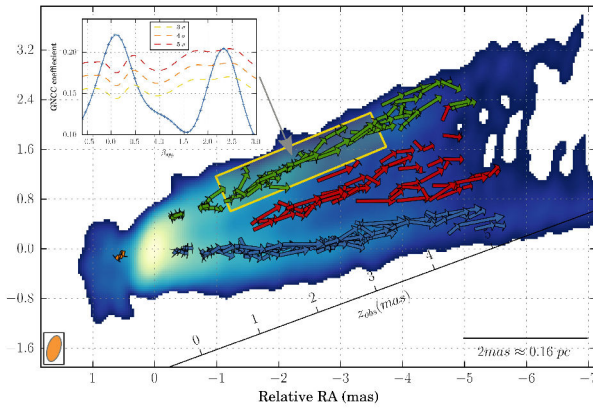
Figure 4.2: Courtesy of Mertens et al. (2015). Kinematics study of the inner jet of M87 reveal the presence of a two-flow structure with speeds ranging from 0.5c on the edges to \Gamma \approx 6 in the spine.
