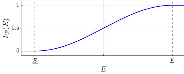
Figure 6.3 – Qualitative plot of the adaptive gain k_E(E) for \underline{E} = 1 \times 10^{-5} and \overline{E} = 1 \times 10^{-4} used to tune the effect of the active camera velocity optimization depending on the current status of the structure from motion estimation.
