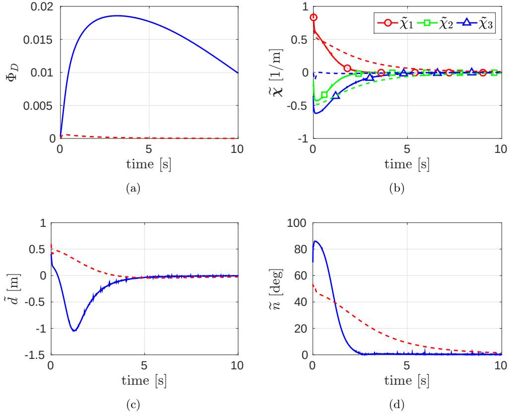
Figure 5.13 – Simulation results for plane estimation employing three adaptive moments of degree \delta = 2 and optimizing for both vector \theta and the camera linear velocity \mathbf{v} (solid lines). Fig. (a): the value of \Phi_D is now \approx 10^7 times larger than in the previous case of Fig. 5.12(a). This then allows for a quick convergence of the error quantities \tilde{\chi}(t) (Fig. (b)), \tilde{d}(t) (Fig. (c)) and \tilde{n}(t) = \arccos(\mathbf{n}^T(t)\hat{\mathbf{n}}(t)) (Fig. (d)). For a comparison, in all plots dashed lines correspond to the use of the five moments ( x_g, y_g, \mu_{20}, \mu_{11}, \mu_{02} ): it is worth noting how, despite the increased measurement set (five moments vs. only three), the estimation convergence results still slower than in the weighted moment case.
