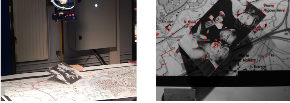
Figure 5.9 – Experimental setup for the estimation of the plane parameters in presence of outlier measurements. Note the introduction of the inclined picture in the observed scene on the right.
