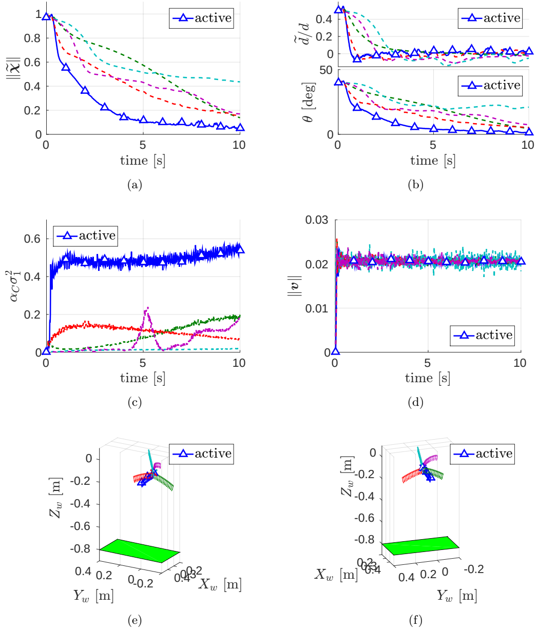
Figure 5.8 – Experimental results for the estimation of the plane parameters using discrete image moments method C with an active strategy (blue lines) or a random acceleration (purple line) or a constant linear velocity (green, red and cyan lines). Fig. (a): normalized norm of the estimation error \tilde{\chi} . Fig. (b): relative error between estimated and actual distance d and angle between the estimated and actual normal \mathbf{n} . Fig. (c): smallest eigenvalue \sigma_1^2 of the 3 \times 3 matrix \Omega \Omega^T multiplied by \alpha_C . Fig. (d): camera linear velocity norm. Fig. (e) and Fig. (f): geometric 3-D trajectory of the camera with arrows indicating the optical axis and a green patch representing the plane to be estimated.
