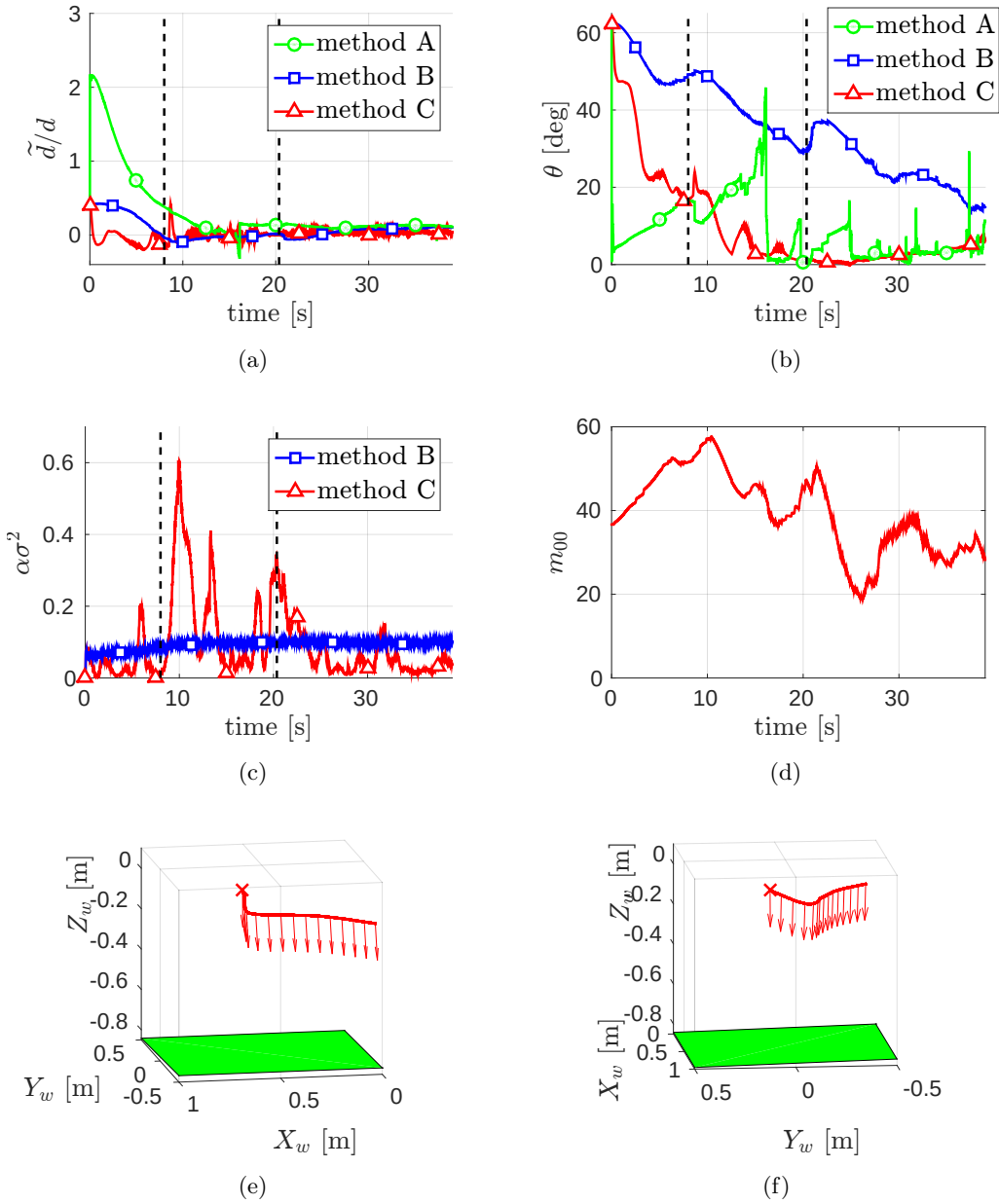
Figure 5.10 – Experimental results for plane estimation in presence of outlier measurements using homography decomposition (method A – green lines), 3-D points estimation (method B – blue lines) or image moments (method C – red lines). Fig. (a): relative error between estimated and actual distance d ; Fig. (b): angle between the estimated and actual normal \mathbf{n} ; Fig. (c): product \alpha\sigma methods B and C; Fig. (d): evolution of the image moment m_{00} ; Fig. (e) and Fig. (f): geometric 3-D trajectory of the camera with arrows indicating the optical axis and a green patch representing the plane to be estimated.
