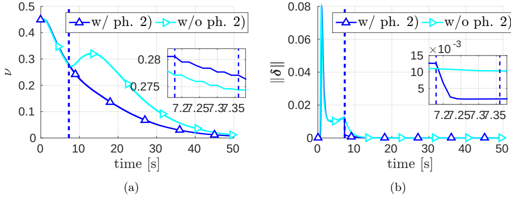
Figure 7.4 – Importance of implementing phase 2) of Fig. 6.2 in the regulation of 4 point features starting from a different initial camera pose. Behavior of the error norm \nu(t) (Fig. (a)) and of \|\delta(t)\| , the measure of misalignment between vectors \mathbf{e} and \dot{\mathbf{e}} (Fig. (b)). In both plots, the blue lines represent the behavior of case I (full implementation of the switching strategy of Sect. 6.2.3), while cyan lines represent the direct switch from phase 1) to phase 3) without the action of vector \ddot{\mathbf{q}}_w = \ddot{\mathbf{q}}_\delta in (6.14). The small picture-in-picture plots provide a zoomed view of the switching phase.
