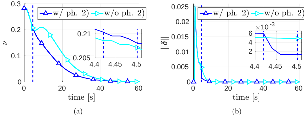
Figure 7.2 – Importance of implementing phase 2) of Fig. 6.2 in the regulation of 4 point features. Behavior of the error norm \nu(t) (Fig. (a)) and of \|\delta\| , the measure of misalignment between vectors \mathbf{e} and \dot{\mathbf{e}} (Fig. (b)). In both plots, the blue lines represent the behavior of case I (full implementation of the switching strategy of Sect. 6.2.3), while cyan lines represent the direct switch from phase 1) to phase 3) without the action of vector \ddot{\mathbf{q}}_w = \ddot{\mathbf{q}}_\delta in (6.14). The small picture-in-picture plots provide a zoomed view of the switching phase.
