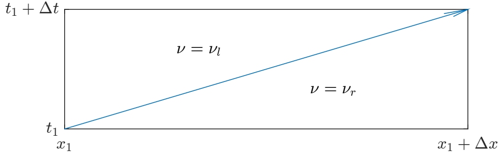
Figure B.7 – Shock speed propagation on the plane (x, t) . Figure modified from [LeV02].
