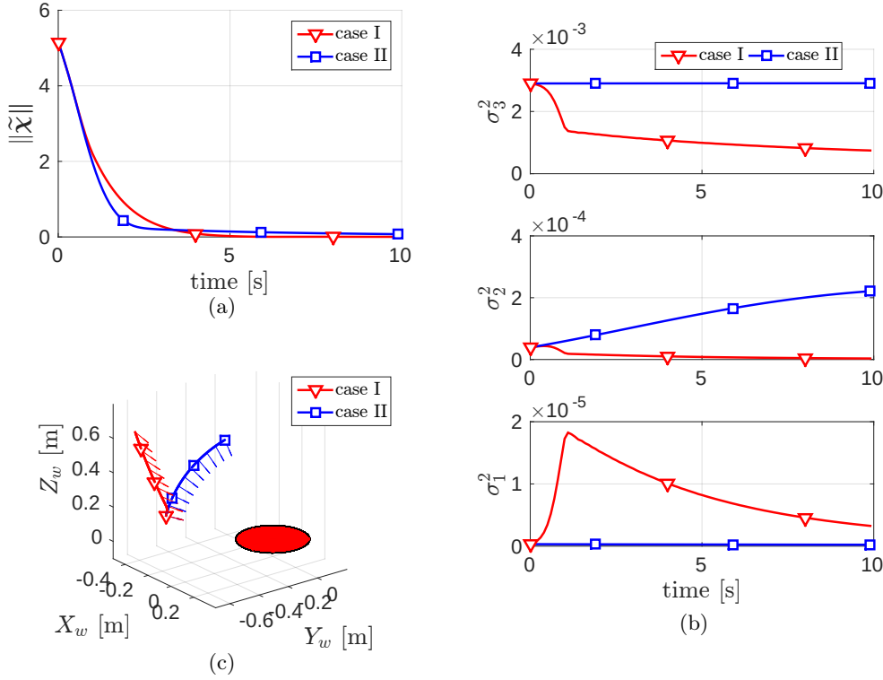
Figure 5.17 – Simulation results for the dense moments case. Fig. (a): behavior of \|\tilde{\chi}(t)\| for case I (red lines) and case II (blue lines). Fig. (b): behavior of the three eigenvalues of matrix \Omega\Omega^T for case I (red lines) and case II (blue lines). Note how the convergence rate of case II is initially faster than in case I due to a higher value of the two largest eigenvalues \sigma_2^2, \sigma_3^2 (see Fig. (b)) which are not being controlled. However, once the smallest eigenvalue \sigma_1^2 becomes dominant, the maximization of \sigma_1^2 operated in case I results, as expected, in a faster convergence rate of the estimation error. Fig. (c): 3-D Cartesian trajectory followed by the camera for case I (red line) and case II (blue line) together with the planar circle used to generate image moments. In case I, the camera has a larger velocity along the Z -axis that results in a larger \sigma_1^2 .
