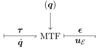
Figure 2.7 – Bond graph representation of the robot geometric Jacobian. The Jacobian (2.14) can be represented as a Modulated Transformer (MTF), function of the robot joint configuration (top arrow). The generalized effort and flows variables are indicated on the top and bottom of the MTF ports.
