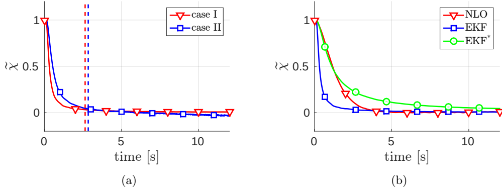
Figure 5.5 – Experimental results for the depth estimation of a point feature using an EKF. Fig. (a): behavior of the estimation error for case I (solid red line) and case II (solid blue line). The two vertical dashed lines indicate the times T_1 = 2.64 s and T_2 = 2.84 s at which the estimation error drops below the threshold of 3 cm. Note how the use of an active strategy for optimizing the direction of the camera linear velocity results, again, in improved performance of the estimator. Fig. (b): behavior of the estimation error for the nonlinear observer (solid red line) and the EKF (solid blue line) in case I. The green line (labeled EKF* in the legend) finally represents the estimation error for the EKF in case I when the estimator is initialized with a covariance of \hat{\chi}(t_0) 10 times larger than in the blue line case.
