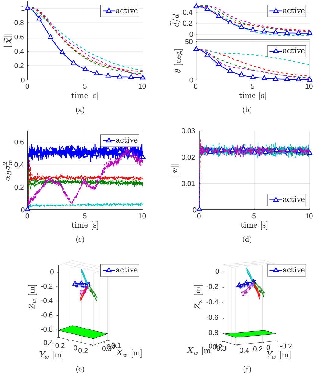
Figure 5.7 – Experimental results for the estimation of the plane parameters using 3-D points (method B) with an active strategy (blue lines) or a random acceleration (purple line) or a constant linear velocity (green, red and cyan lines). Fig. (a): normalized norm of the estimation error \tilde{\mathbf{x}} ; Fig. (b): relative error between estimated and actual distance d and angle between the estimated and actual normal \mathbf{n} . Fig. (c): smallest eigenvalue \sigma_m^2 of the N \times N matrix \Omega \Omega^T multiplied by \alpha_B . Fig. (d): camera linear velocity norm. Fig. (e) and Fig. (f): geometric 3-D trajectory of the camera with arrows indicating the optical axis and a green patch representing the plane to be estimated.
