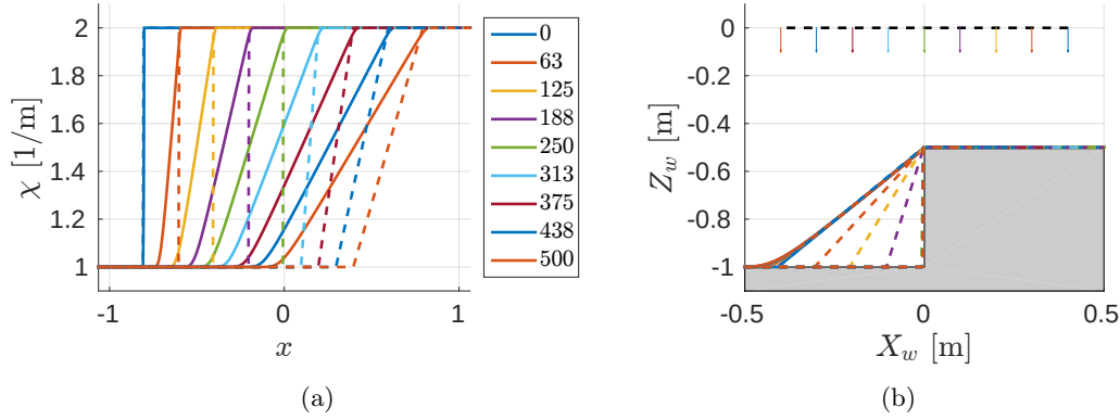
Figure B.6 – Photometric depth estimation for a rarefaction wave. Fig. (a) evolution of the actual (dashed) and numerically propagated (solid) disparity map at equally spaced iterations (check the legend). Fig. (b) reconstruction of the environment from the actual (dashed) and numerically propagated depth maps with arrows representing the camera position and the direction of the optical axis, and using the same color code as in Fig. (a).
