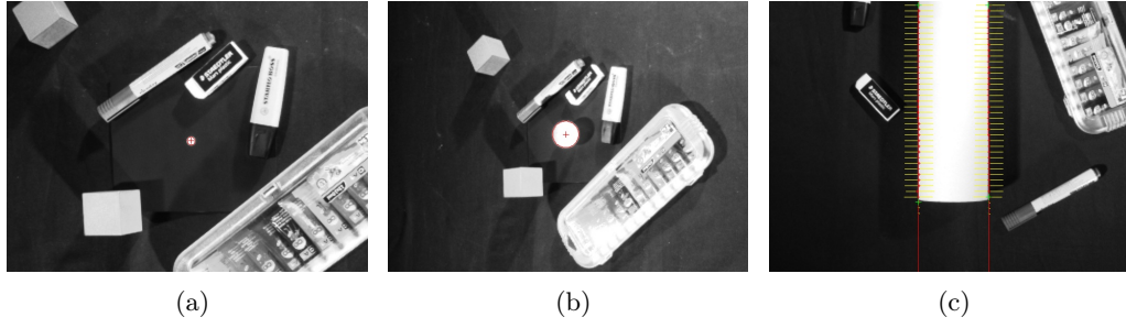
Figure 5.3 – Camera snapshots for the point feature Fig. (a), the sphere Fig. (b) and the cylinder Fig. (c) experiment. The result of the image processing is highlighted in red.
