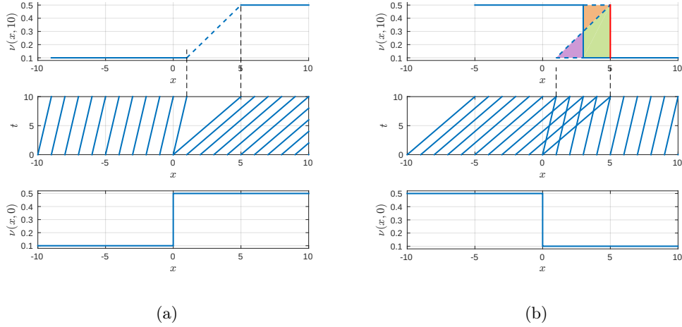
Figure B.5 – Time-space evolution of a rarefaction and shock wave. Fig. (a): evolution of a rarefaction wave. Fig. (b): evolution of a shock wave. For both figures, from bottom to top we show: (i) the initial condition \nu(x, 0) , (ii) some of the characteristic curves emanating from x = -10 + k with k = 0, 1, \dots, 20 , and (iii) the final condition \nu(x, 10) . This picture is similar to some reported in [LeV02].
