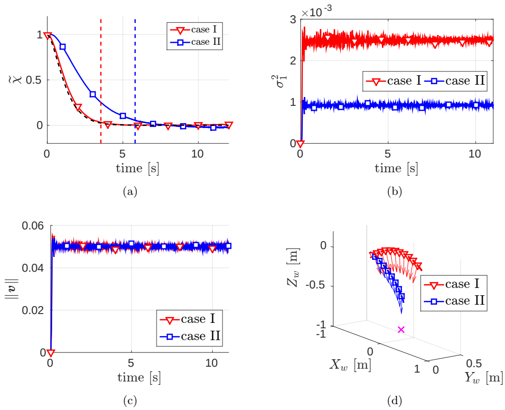
Figure 5.4 – Experimental results for the depth estimation of a point feature. Fig. (a): behavior of the estimation error for case I (solid red line) and case II (solid blue line), and for an ‘ideal’ second order system (4.15) with desired poles at \sigma_{max}^2 (dashed black line). The two vertical dashed lines indicate the times T_1 = 3.54 s and T_2 = 5.81 s at which the estimation error drops below the threshold of 3 cm. Fig. (b): behavior of \sigma_1^2(t) for case I (red line) and case II (blue line). Fig. (c): camera linear velocity norm \|v\| for case I (red line) and case II (blue line). Fig. (d): Camera trajectories for case I (red line) and case II (blue line) with arrows indicating the direction of the camera optical axis. Note how the use of an active strategy for optimizing the direction of the camera linear velocity results in improved performance of the estimation for the same control effort (i.e. same velocity norm).
