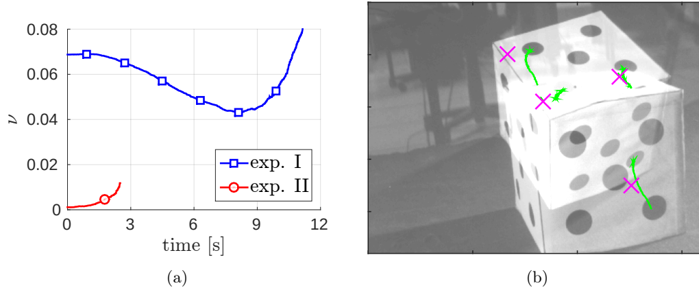
Figure 7.5 – IBVS of 4 point features using a constant approximation \chi(t) = \chi_d where the value of \chi_d is corrupted by a relative error of 9%. In the first experiment the camera starts far from the desired pose, while in the second experiment the camera starts at almost the desired pose. Fig. (a): behavior of the error norm \nu(t) for the first (blue line) and second (red line) experiments. Because of the approximated value of \chi_d , the servoing is not able to converge in both cases (thus also when starting very close to the desired pose), resulting in a loss of tracking for the point features. Fig. (b): image plane trajectory of the 4 point features during the first experiment. The four crosses indicate the desired feature positions, and the initial and final (i.e., until loss of tracking) camera images are superimposed.
