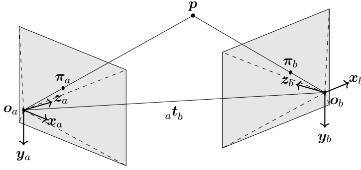
Figure 2.5 – Geometrical representation of the epipolar constraint. The points {}^a\pi and {}^b\pi represent the projections of the same point p from two camera vantage points related by the rigid transformation described by the rotation matrix {}^aR_b and the translation vector {}^a t_b .
