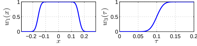
Figure 4.2 – Possible shape of the weight functions used to cope with a limited camera FOV. Left: shape of weight w_1(x) with limits x_{min} = -x_{max} = 0.2884 (normalized size of the image plane). Right: shape of weight w_3(\tau) .
