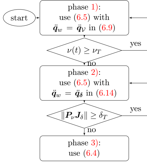
Figure 6.2 – Flowchart representation of the basic switching control strategy.
