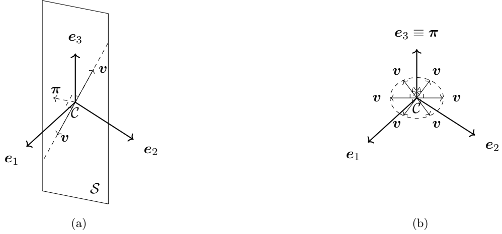
Figure 4.1 – Optimality conditions for the camera linear velocity \mathbf{v} as dictated by system (4.33). Fig. (a): when \pi \neq e_3 , vector \mathbf{v} must be orthogonal to \pi and lie on the plane \mathcal{S} spanned by \pi and e_3 (that is, \mathbf{v} must belong to a specific straight line). Fig. (b): when \pi = e_3 , any \mathbf{v} \perp e_3 is a valid solution to (4.33).
