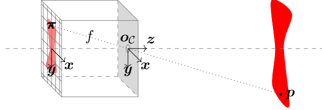
Figure 2.3 – Projection model of a pinhole camera.
