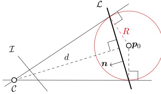
Figure 4.4 – Geometry of a spherical object. Spherical target \mathcal{O}_S and planar limb surface \mathcal{L} .
