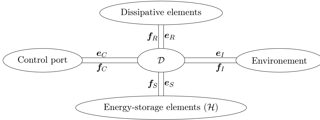
Figure C.2 – General structure of a port-Hamiltonian system with the Dirac structure \mathcal{D} in the center and the four ports representing internal energy-storage ( \mathcal{S} ) and dissipative ( \mathcal{R} ) elements and the interconnection with the control action ( \mathcal{C} ) and the environment ( \mathcal{I} ).
