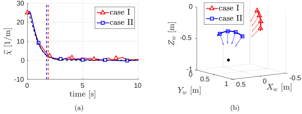
Figure 5.18 – Experimental results for the estimation of the radius of a sphere using different constant camera velocities with the same norm. Fig. (a): behavior of the estimation error \tilde{\chi}(t) for the two cases (solid blue and red lines), and for an ‘ideal’ second order system with poles at the desired locations (dashed black line). The vertical dashed lines indicate the times at which the estimation error \tilde{\chi}(t) drops below the threshold of 1 mm. Fig. (b): camera trajectories for case I (blue line) and case II (red line) with arrows indicating the direction of the camera optical axis.
