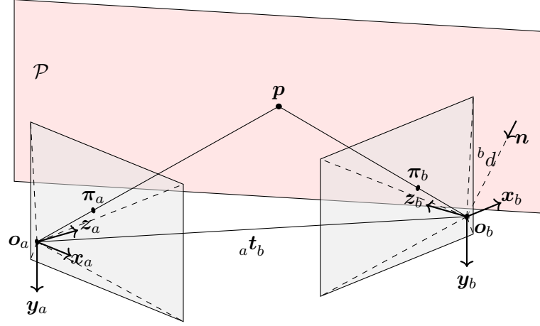
Figure 2.6 – Geometrical representation of the homography constraint. The points {}^a\pi and {}^b\pi represent the projections of the same point p from two camera vantage points related by the rigid transformation described by the rotation matrix {}^aR_b and the translation vector {}^a t_b .
