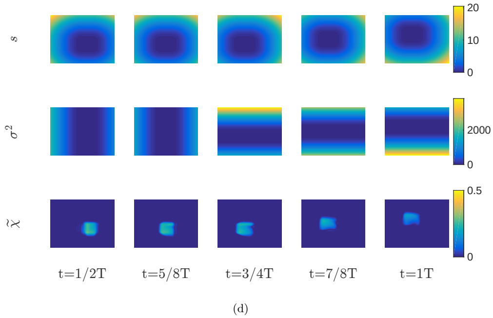
Figure B.1 – Photometric depth estimation for a planar scene. Fig. (a): camera trajectory with arrows indicating the direction of the camera optical axis and the observed textured plane. In the other plots: evolution of the image s = Y , observability eigenvalue \sigma^2 , and disparity estimation error \tilde{\chi} maps for the first (Fig. (b)) and second (Fig. (c)) quarters of period and for the second half of the time (Fig. (d)). Note that a RGB color map was used for these plots for better readability, however all of these maps are scalar.
