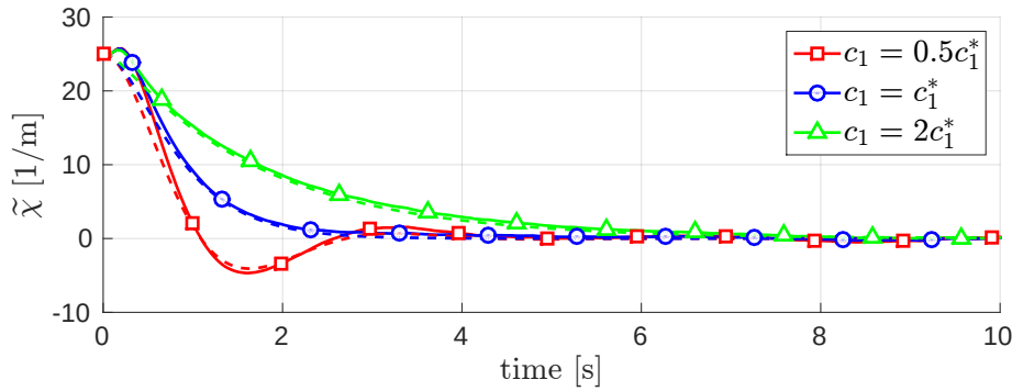
Figure 5.19 – Experimental results for the estimation of the radius of a sphere with different damping factors: c_1 = c_1^* (blue line), c_1 = 2c_1^* (green line) and c_1 = 0.5c_1^* (red line). The dashed lines represent the response of an ‘ideal’ second order system with the corresponding poles. Note again the almost perfect match between the plots.
