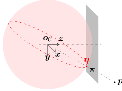
Figure 2.4 – Planar and spherical perspective projection models.
