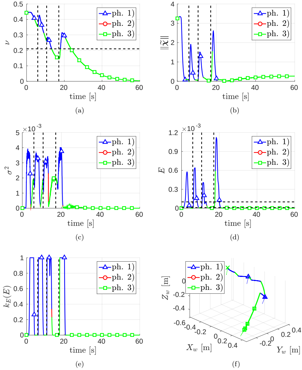
Figure 7.6 – Regulation of 4 point features using the adaptive strategy of Sect. 6.3. The three phases of Fig. 6.4 are denoted by the following color code: blue – phase 1), red – phase 2), green – phase 3). Fig. (a): behavior of the error norm \nu(t) with superimposed a horizontal dashed black line indicating the threshold \nu_T . Fig. (b): behavior of the norm of the estimation error \|\tilde{\chi}(t)\| = \|\chi(t) - \hat{\chi}(t)\| . Fig. (c): behavior of the mean eigenvalue \sigma^2 . Fig. (d): behavior of E(t) with, superimposed, two dashed horizontal lines indicating the minimum and maximum thresholds \underline{E} and \overline{E} . Fig. (e): behavior of the adaptive gain k_E(E) . In all of the previous plots, vertical dashed lines represent the times at which the target object was intentionally displaced. Fig. (f): camera 3-D trajectory with arrows representing the camera optical axis and square and circular markers representing the camera initial and final poses, respectively.
