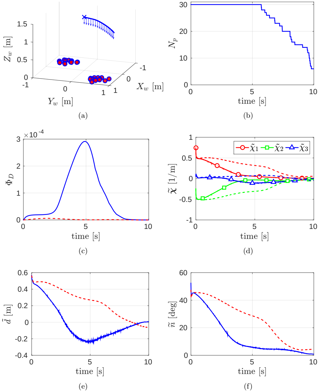
Figure 5.15 – Simulation results for plane estimation employing three constrained adaptive moments, a camera with limited FOV, and optimizing for both vector \theta and the linear velocity v (solid lines). Fig. (a): camera trajectory and direction of the optical axis during the estimation task. Fig. (b): number N_p of tracked point features over time. Fig. (c): behavior of \Phi_D(t) which reaches a maximum of \approx 2.9 \cdot 10^{-4} before starting to decrease because of the fewer tracked points. Finally the other figures show the behavior of the error quantities \tilde{\chi}(t) (Fig. (d)), \tilde{d}(t) (Fig. (e)) and \tilde{n}(t) (Fig. (f)). In dashed lines, the behavior that all quantities would have had in case no optimization of \theta had been performed.
