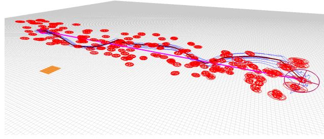
Figure 3.2 – Trajectory planning to minimize uncertainty for micro aerial vehicles. The objective is to reach the final pose (to the left) while minimizing the localization uncertainty. The resulting trajectory (black line) is more informative than the direct magenta path. From [AWCS13].
