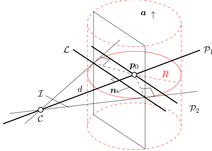
Figure 4.5 – Geometry of a cylindrical object. Camera \mathcal{C} and cylindrical target \mathcal{O}_C with the planar limb surface \mathcal{L} and the other planes of interest \mathcal{P}_1 and \mathcal{P}_2
