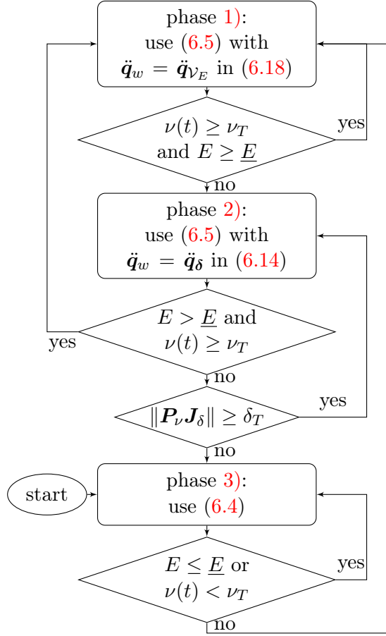
Figure 6.4 – Flowchart representation of the adaptive switching strategy exploiting the measurable error energy for triggering changes of status.
