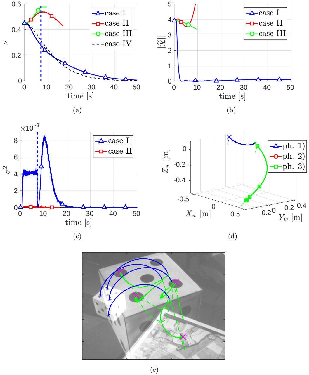
Figure 7.3 – Regulation of 4 point features starting from a different initial camera pose w.r.t. the experiments reported in Fig. 7.1. The plot pattern and color codes are the same as in Fig. 7.1. Note how, this time, a correct realization of the servoing task is obtained only in case I (blue line in Fig. 7.3(a)). In case II, the estimation error \|\tilde{\chi}(t)\| diverges (red line in Fig. 7.3(b)) because of the too small value of \sigma^2(t) (red line in Fig. 7.3(c)) during the camera motion which makes the estimation task ill-conditioned. In case III, the visual task error starts diverging because of the too rough approximation \hat{\chi} = \chi_d and the point features leave the camera FOV (green line in Fig. 7.3(a)). Note also the initial spiralling motion of the camera (blue line in Fig. 7.3(d)) that allows maximization of the value of \sigma^2(t) during phase 1) of case I.
