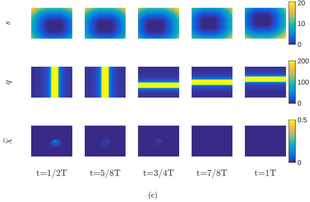
Figure B.3 – Photometric depth estimation for a planar scene with regularization of the disparity map. Evolution of the image s = Y , regularization gain q , and disparity estimation error \tilde{\chi} maps for the first (Fig. (a)) and second (Fig. (b)) quarters of period and for the second half of the time (Fig. (c)). A RGB color map was used for these plots for better readability, however all of these maps are scalar. Note how the regularization term is mostly active in the unobservable areas (compare q here with the plots of \sigma^2 in Fig. B.1).
