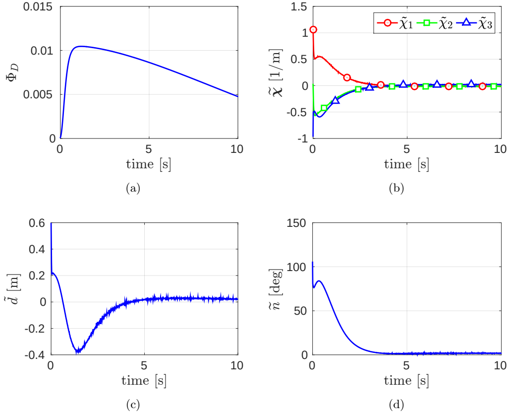
Figure 5.14 – Simulation results for plane estimation employing three adaptive moments of degree \delta = 2 and only optimizing for vector \theta . Fig. (a): note how \Phi_D(t) still reaches a range of values comparable with the previous case of Fig. 5.13(a) despite the lack of any optimization of the camera velocity \mathbf{v} . The other figures show the behavior of the error quantities \tilde{\chi}(t) (Fig. (b)), \tilde{d}(t) (Fig. (c)) and \tilde{n}(t) (Fig. (d)).
