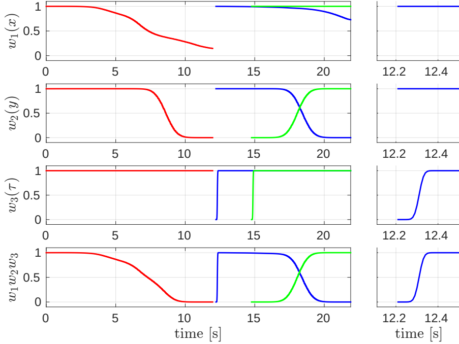
Figure 5.11 – Evolution of the switching functions and of their product for three representative point features. On the right: detailed views of the corresponding plots on the left in the time interval immediately following the introduction of the blue feature in the estimator.
