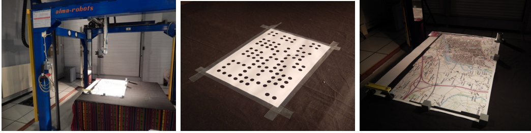
Figure 5.6 – Experimental set-up for plane estimation with the dotted pattern and the topographic map used for feature extraction and tracking.
