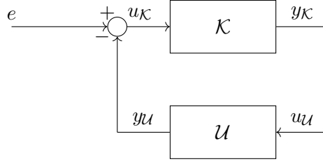
Figure C.1 – Representation of the mass-spring system as an interconnection between two subsystems. \mathcal{K} is associated to the mass and stores the kinetic energy of the system. \mathcal{U} is associated to the spring and stores the potential energy of the system.
