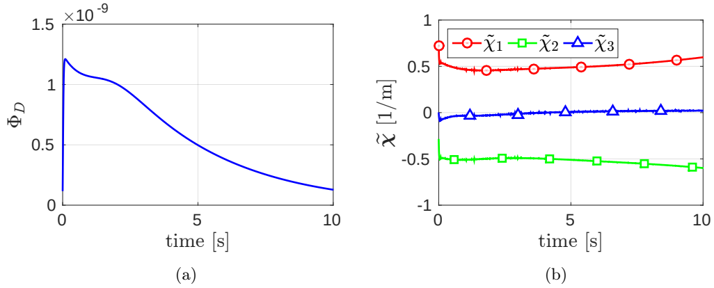
Figure 5.12 – Simulation results obtained by employing the classical discrete moment set (x_g, y_g, \mu_{20} + \mu_{02}) and optimizing for the camera linear velocity \mathbf{v} . In this case \Phi_D(t) keeps very close to zero (the scale of Fig. (a) is 10^{-9} ) and as a consequence the estimation error \tilde{\chi}(t) does not converge (Fig. (b)).
