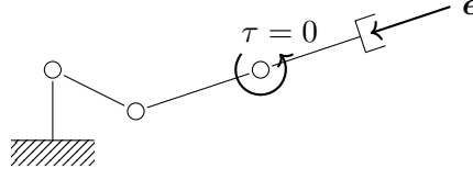
Figure 2.8 – Kinematic singularity. The compensation of the the applied force \epsilon does not require any action from the third joint since the force will be absorbed by first two joints and by the structure of the last two aligned links.
