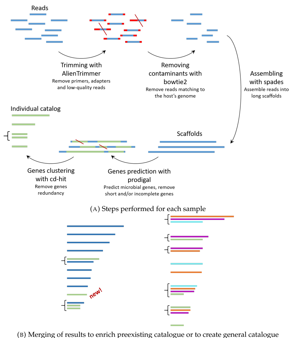
FIGURE 4.1 – Schema of the Metaraptor's steps. (A) Each read file of the samples is treated simultaneously and construct an individual catalogue from the reads. (B) The individual catalogues can enrich a pre-existing catalogue (left, not used in this thesis) or create a catalogue compiling the results of the samples of interest (right, here four samples represented with colours).
