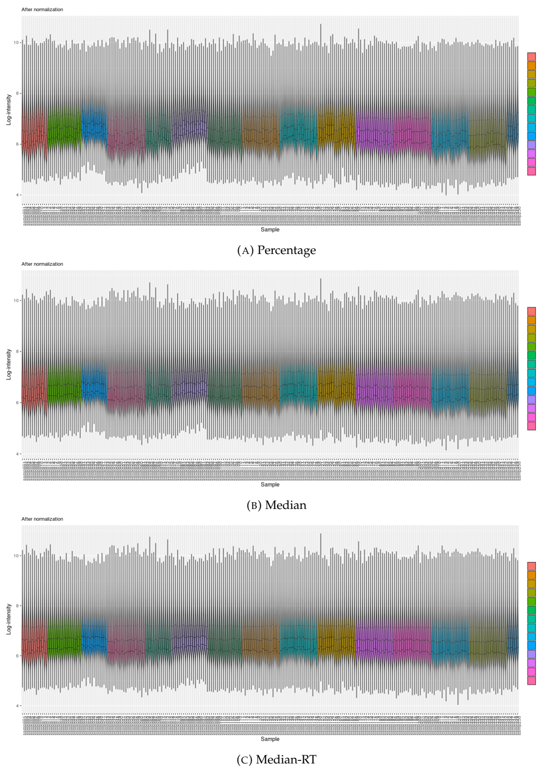
FIGURE 6.10 – Global intensity profiles of XIC after normalization by (A) percentage, (B) median and (C) median-RT. Report to Figure 6.2 for unnormalized data.
