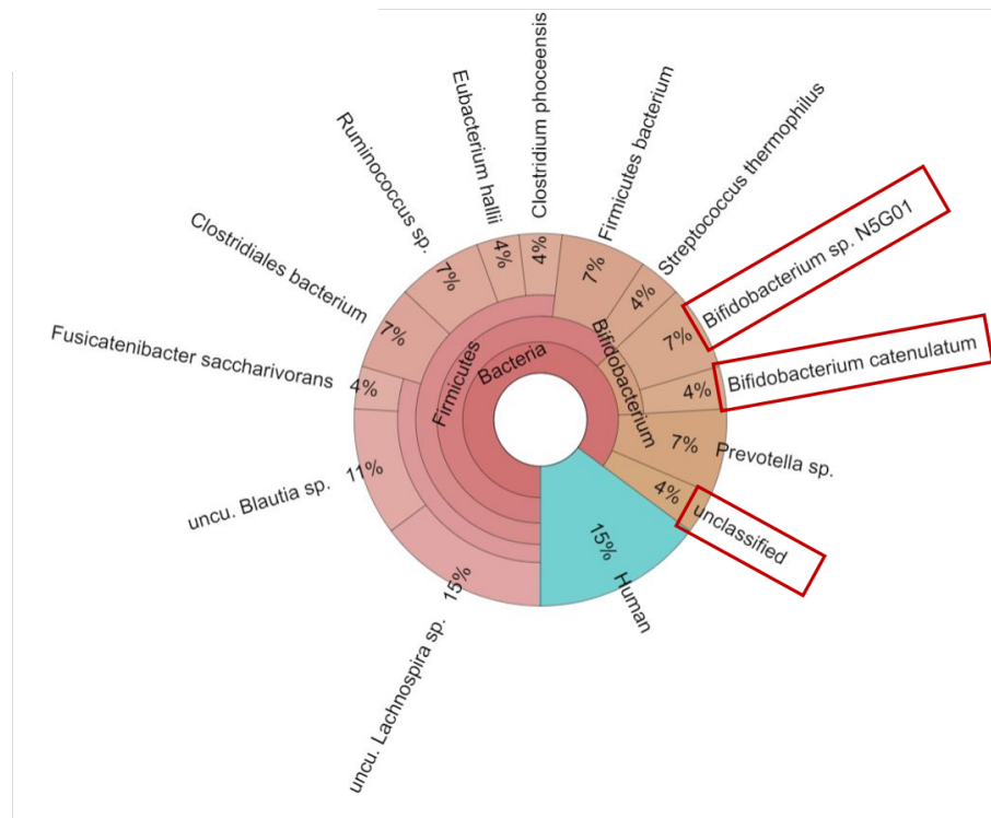
FIGURE 3.2 – Taxonomic distribution of the 27 proteins whose correlation (positive or negative) with weight loss was accentuated over time. The proteins negatively correlated are framed. The Krona chart was computed with KronaTools [107].
