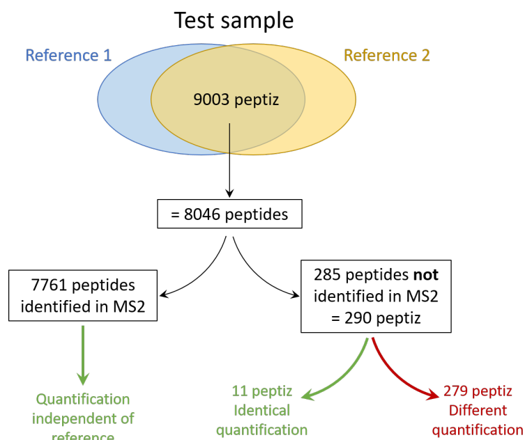
FIGURE 5.2 – Quantification of peptide of a test sample aligned with two references. After XIC alignment of the test sample with each of the reference, 9 003 peptides were quantified in the test sample whatever the reference considered. Most of these peptides corresponds to peptides identified in MS2, for which the quantification is independent on the reference used. Over the peptides for which the peptide was not identified in MS2, and therefore the quantification by XIC would be possible through alignment, large majority had quantification dependent of the reference used, thus probably misaligned with at least one of the two reference.
