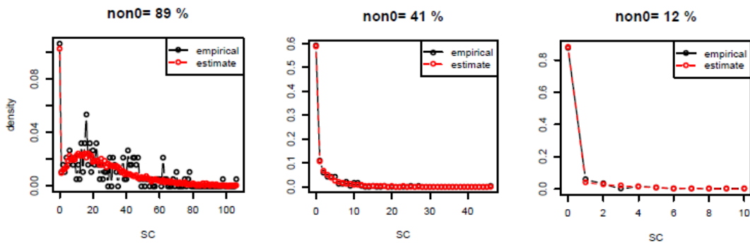
FIGURE 7.2 – Empirical SC of three groups containing 89% (left), 41% (center) and 12% (right) of values greater than 0, and their estimation by zero-inflated negative binomial model.
