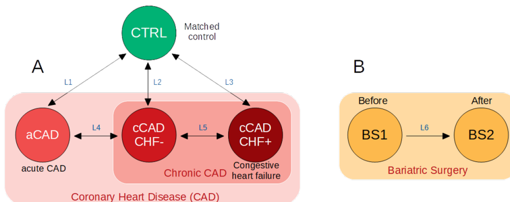
FIGURE 1.12 – Description of the ProteoCardis datasets. 188 individuals constitutes the dataset A, which comprises 138 patients suffering from CAD and 50 controls. 30 obese patients constitutes the dataset B, for whom a sample is collected before and 6 months after a bariatric surgery. The variables L are searched to discriminate the different patient groups.
