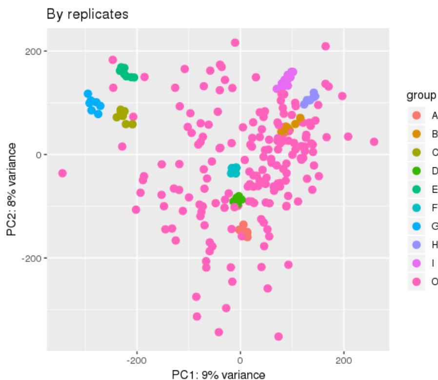
FIGURE 6.5 – Principal Component Analysis of raw Spectral Counts of proteins. The samples are coloured by replicates. A-H: replicates, each replicated seven times. I: Standard, replicated fourteen times. O: samples not replicated.
