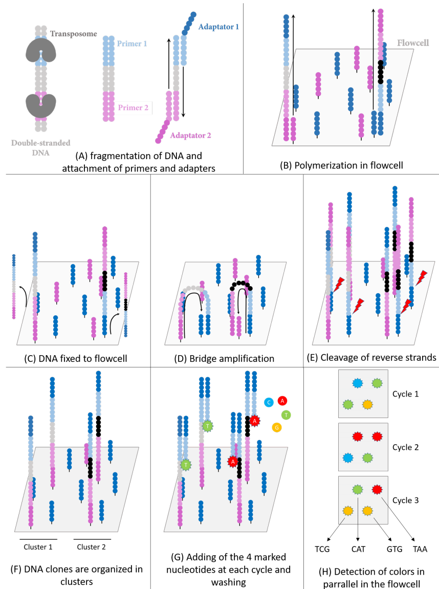
FIGURE 1.3 – Bridge amplification and Illumina sequencing. (A) DNA is fragmented into 200kb fragments and primers are attached by transposomes. The amplification adds two types of adaptors at each end. (B) The DNA fragments are floated onto a flowcell and elongated by DNA polymerase. (C) The unattached strands are washed by denaturation. (D) The strands form bridges at the surface of the flowcell and are amplified by cycles of polymerisation/denaturation. (E) The antisense strands are cut and washed, leaving only sense strands. (F) The sense strands form clusters of the same sequence of DNA, here a cluster of grey DNA and a cluster of black DNA. (G) At each cycle, the four types of nucleotides are introduced into the flowcell and are incorporated by polymerisation. After washing, a laser excites the last nucleotide incorporated, which emits a distinctive colour. (H) At each cycle, the clusters are sequenced in parallel thanks to the colour they emit. The succession of the colours at each cycle determines the sequence of the DNA of each cluster.
