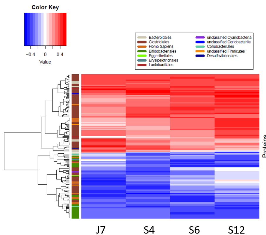
FIGURE 3.1 – Heatmap of proteins positively or negatively correlated with weight loss at a timepoint of the study.
