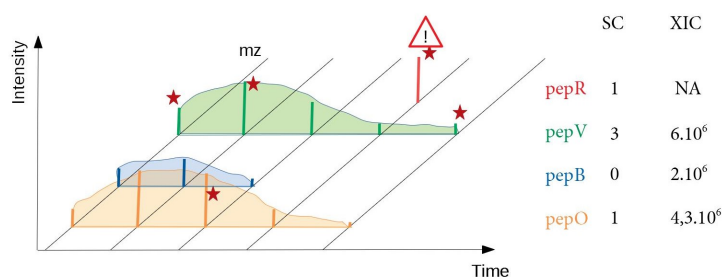
FIGURE 1.11 – Example of quantification of four peptiz by SC and XIC. At each time (x axis), the MS1 peak (coloured bands) with the greater abundance (y axis) is fragmented into MS2. The peak fragmented is symbolized by a red star. pepB is not fragmented, therefore it has a null quantification by SC but its presence is detectable by XIC and quantifiable if it has been fragmented and identified in another sample. The relative abundance of pepV and pepO is more accurate by XIC than by SC. PepR, which is fragmented in MS2 and therefore identified and quantified by SC, has no quantifiable MS1 area because the peptide is not detected at another timepoint.
