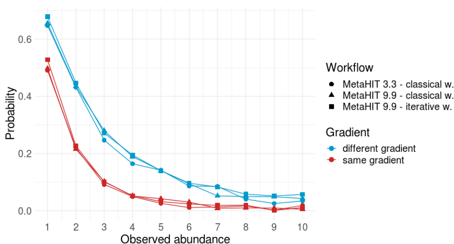
FIGURE 2.13 – Probability to get a zero abundance for a protein in a replicate, as a function of its abundance observed in another replicate. Abundance of a protein is calculated as the sum of its specific spectra.
