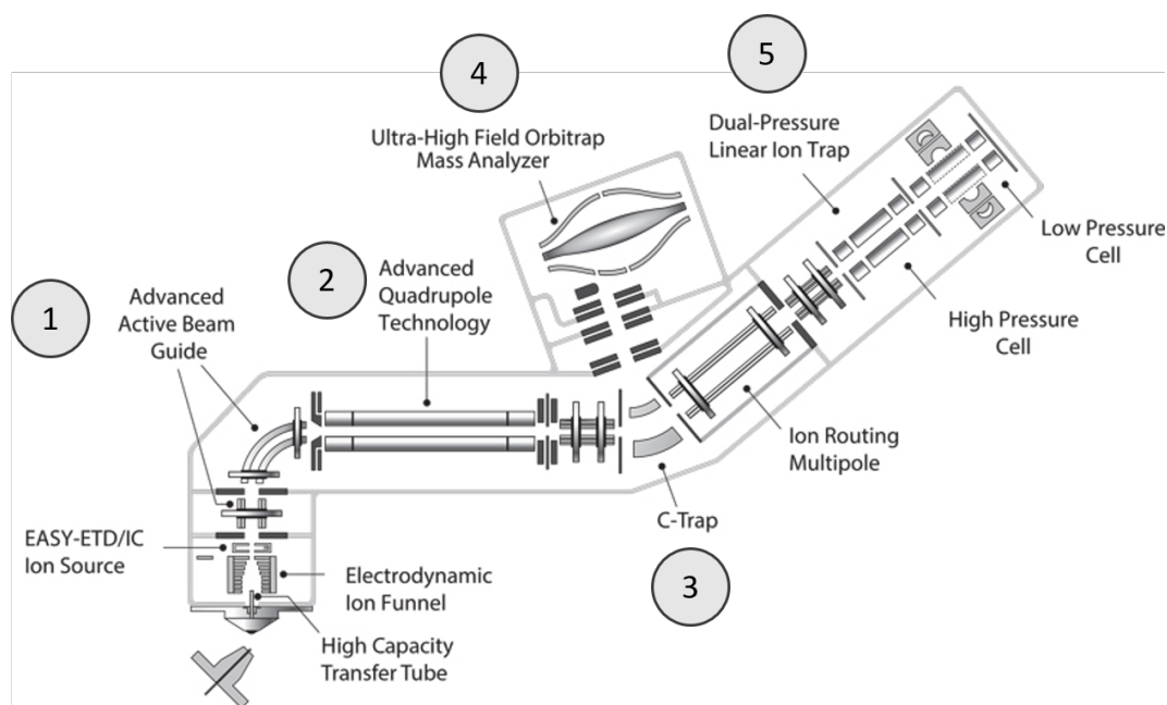
FIGURE 1.9 – Scheme of the Orbitrap Fusion TM Lumos TM Tribrid TM mass spectrometer. The sample is electrosprayed to the transfer tube, and filtered in ① the beam guide to exclude non-ionic molecules. ② The quadrupole selects the ions based on a m/z range. ③ The C-trap traps the ions and pulse them towards ④ the Orbitrap, which performs the first mass analysis (MS1). The ions of interest are selected and trapped in ⑤ the linear ion trap, which fragments them. The fragments are routed to the Orbitrap for the second analysis (MS2) [19].
