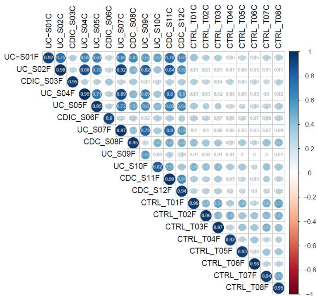
FIGURE 3.3 – Pearson's correlation between metaproteomic profiles (abundance of each of the 43 521 subgroups) of fresh and frozen samples. CTRL: controls; CDC: Colic Crohn's disease; CDIC: Ileo-Colic Crohn's disease; UC: Ulcerative Colitis.
