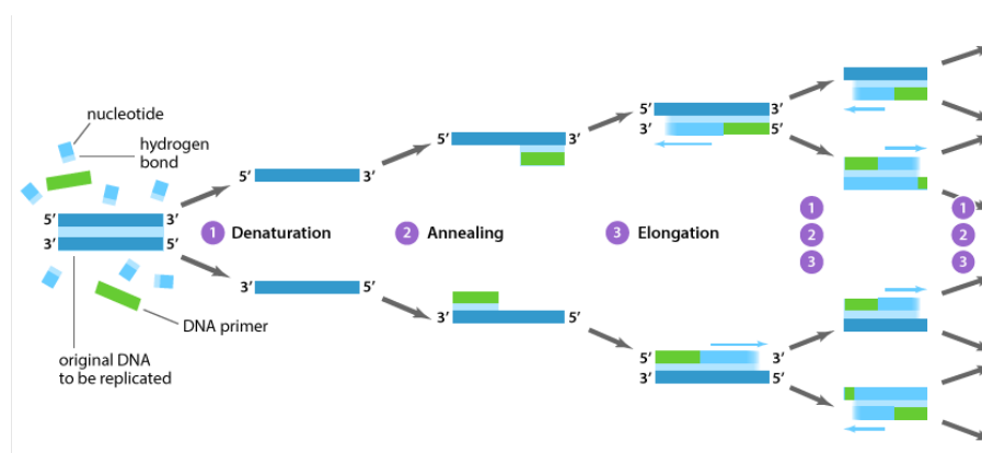
FIGURE A.1 – The different steps of a PCR, from [145].
