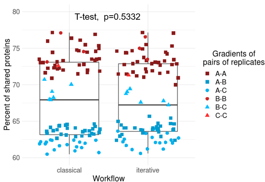
FIGURE 2.18 – Fraction of common proteins identified in each pair of replicates, with the classical and the iterative strategies.
