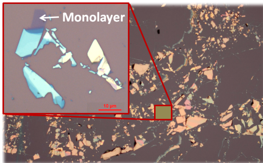
Figure 5: Typical example of a TMDC monolayer flake among other exfoliated flakes. Here one can see the difficulty of finding the monolayer area. The insert shows a zoom on the area of interest where lay several flakes of \text{MoS}_2 including the monolayer area (in grey). Its size is only few \mu\text{m} large, which underline the importance of the use of a micro-photoluminescence setup for the study of this material.
