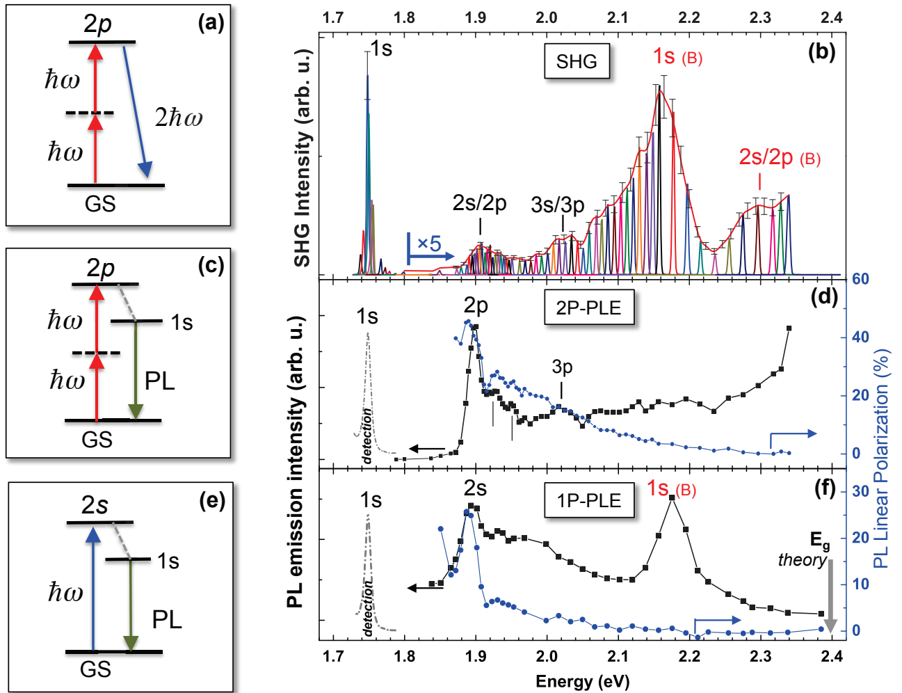
Figure 15: (a) schematic for SHG when 2 incident photons energy is resonant with the 2p state of the A-exciton (b) results of SHG spectroscopy at T=4\text{K} as a function of 2\hbar\omega . (c) schematic for 2 photon PLE (d) 2 photon PLE intensity (left axis, black squares) and linear polarization (right axis, blue circles) as a function of 2\hbar\omega = 2E_{\text{Laser}} . (e) schematic for 1 photon PLE (f) 1 photon PLE intensity (left axis, black squares) and linear polarization (right axis, blue circles) as a function of \hbar\omega . The dashed green line in (c) and (e) represent the energy relaxation path, e.g. by phonon emission.
