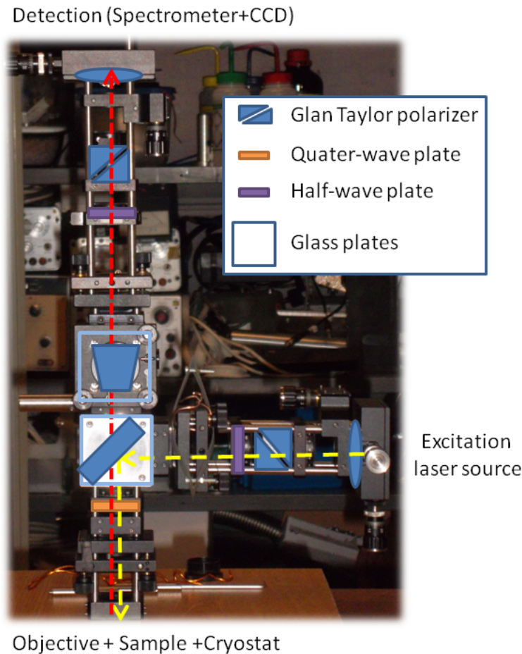
Figure 8: Atto1000 experimental setup. One can identify all the optical elements used, as well as the different light paths. The yellow large-dotted arrows represent the excitation path, the red thin-dotted arrows represent the detection path that is sent into one of our detection setup. The imaging camera, not visible here, is fixed to the above cube, capturing the light reflected on the sample.
