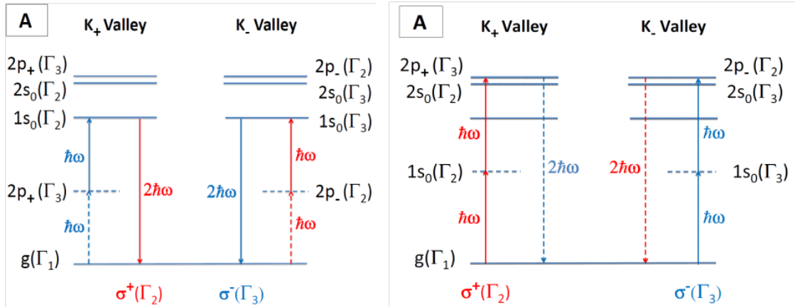
Figure 3: Second harmonic generation process with the 2\hbar\omega emitted photon in resonance with the A-1s 0 exciton states (left), or with the A-2p ± exciton (right). The solid arrows represent electric dipolar interactions, while the dashed one the magnetic dipolar transitions. Note that the selection rules deduced from the macroscopic description are indeed obtained again. The dashed horizontal lines represent virtual states. color code: red = σ + polarized; blue = σ - polarized; line code: solid line = DE; dashed line = DM
