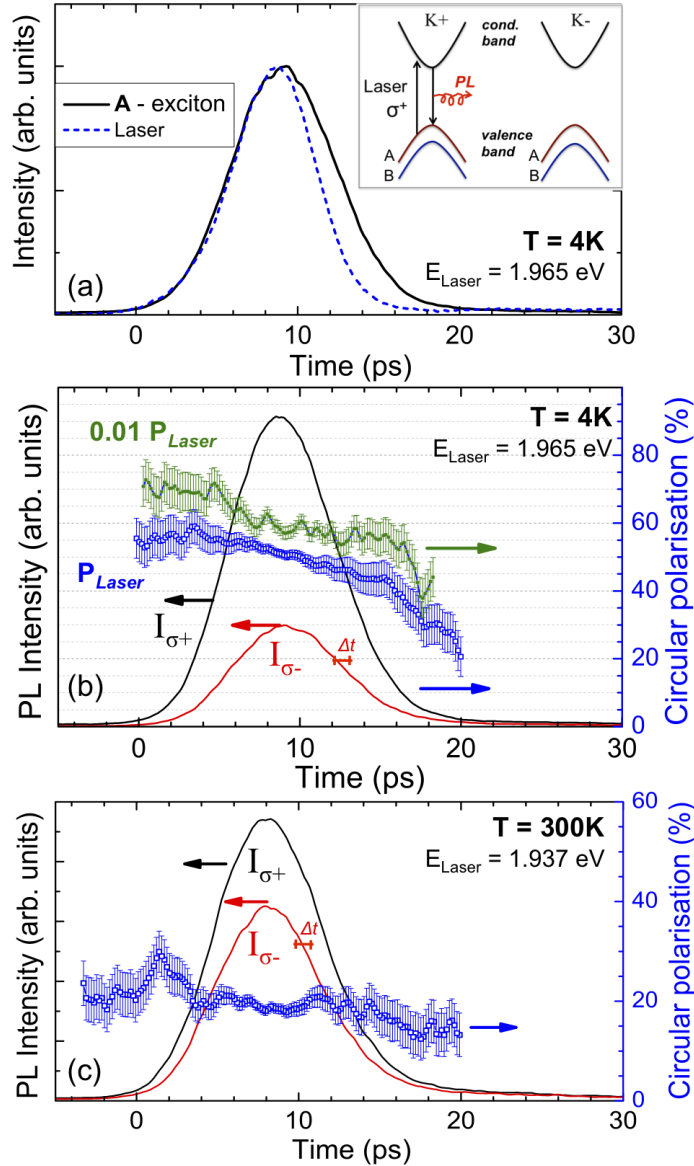
Figure 1: Time resolved photoluminescence of A-exciton. (a) Laser pulse (blue line) and PL emission (black line) intensity at T = 4 K detected at maximum of A-exciton PL E_{\text{Det}} = 1.867 eV as a function of time. Inset: Chiral optical selection rules in 1ML \text{MoS}_2 (b) T=4 K, E_{\text{laser}} = 1.965 eV, E_{\text{Det}} = 1.867 eV. Laser polarization \sigma^+ . Left axis: \sigma^+ ( \sigma^- ) polarized PL emission intensity presented in black (red) as a function of time. Right axis: Circular polarization degree during exciton emission (blue hollow squares: excitation power P_{\text{laser}} \approx 550 \mu\text{W}/\mu\text{m}^2 , green full squares: 0.01 P_{\text{laser}} ), errors bars take into account uncertainty in time origin \Delta t \sim 0.7 ps. (c) same as (b), but for T=300 K, E_{\text{laser}} = 1.937 eV, E_{\text{Det}} = 1.828 eV.
