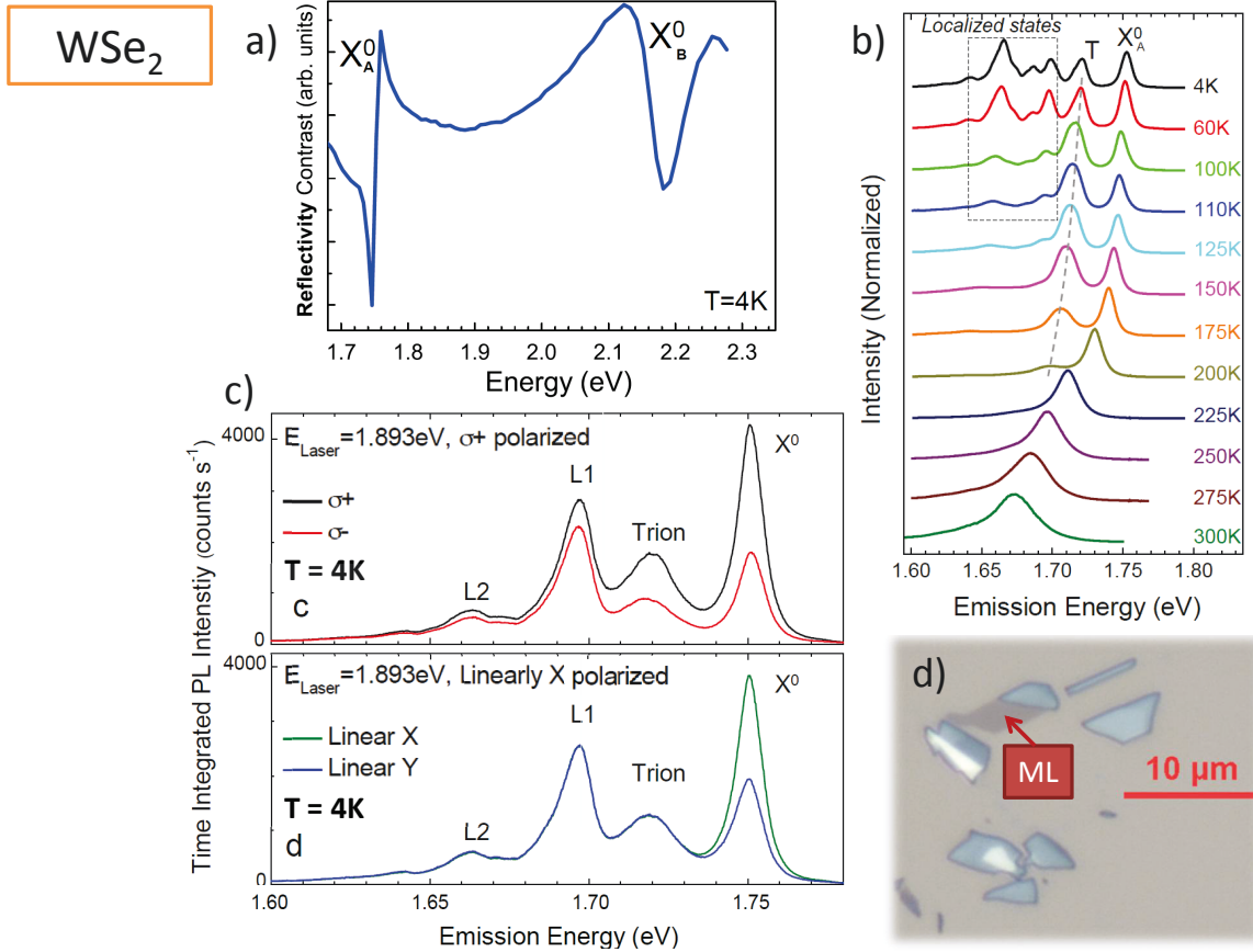
Figure 3: Overview of WSe 2 monolayer sample. (a) Reflectivity measurement allowing to extract an energy splitting between X A 0 and X B 0 lines of \approx 450 meV, in good agreement with both experimental and theoretical values of the literature [26] (b) Temperature dependence of the PL emission. (c) Circular and linear polarization of the PL under respectively circular and linear excitation (T = 4 K). (d) Picture of the monolayer area of the sample under an optical microscope.
