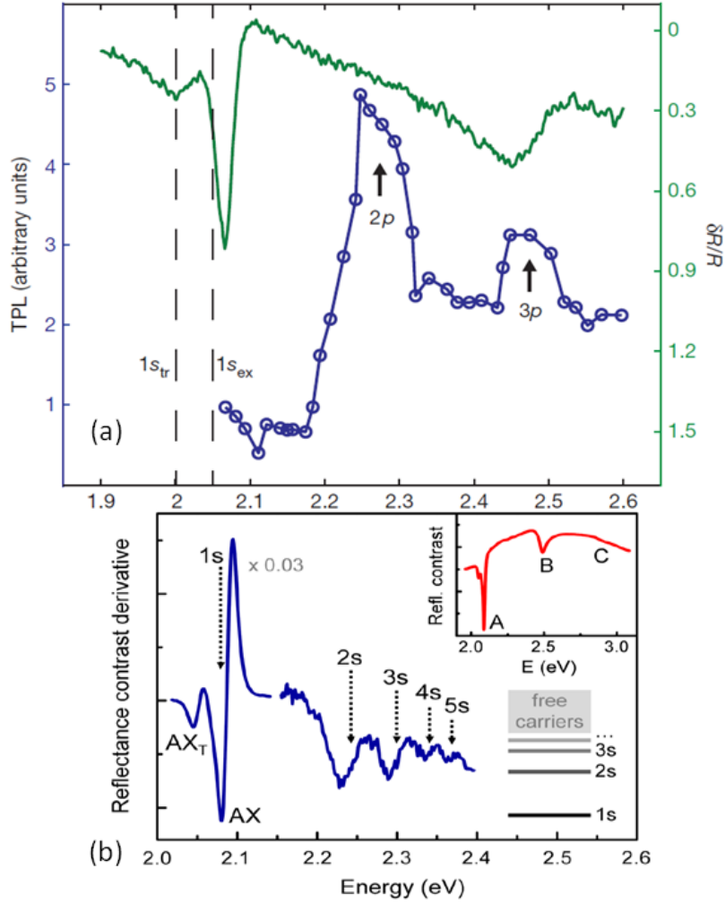
Figure 11: (a) 2photon absorption (blue) and one-photon absorption (green) spectra are measured in single-layer WS 2 at 10 K. Figure extracted from ref. [127] (X. Zhang group, Berkeley) (b) The derivative of the reflectance contrast spectrum \left(\frac{\partial}{\partial E}\right)\left(\frac{\Delta R}{R}\right) of the WS 2 monolayer. Figure extracted from ref. [87] (T. Heinz group, Columbia university)
