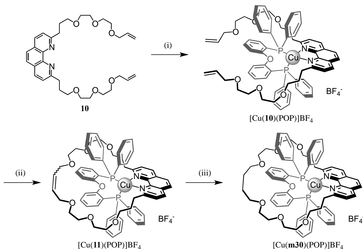
Scheme 7. Reagents and conditions: (i) POP, Cu(CH 3 CN) 4 BF 4 , CH 2 Cl 2 , CH 3 CN (85%); (ii) second generation Grubbs' catalysts, CH 2 Cl 2 (36%); (iii) H 2 , Pd/C, THF (40%).
