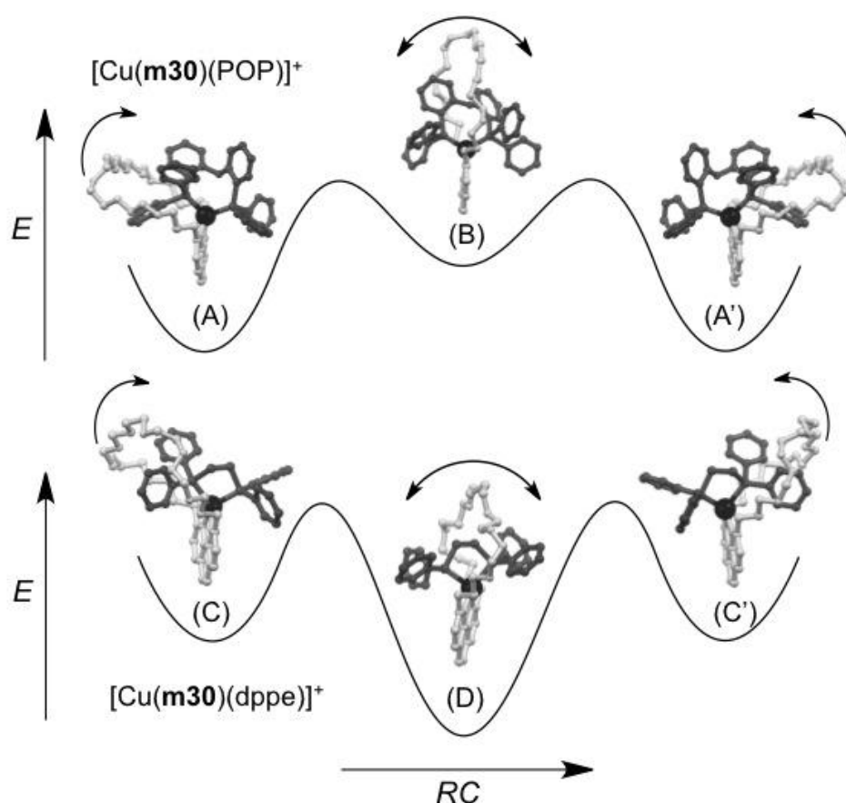
Figure 14. Calculated structures of the different topomers of [Cu(m30)(POP)] + (top) and [Cu(m30)(dppe)] + (bottom); m30 : pale gray, PP ligand: dark gray, Cu: black, the H atoms have been omitted for clarity. A potential energy diagram is proposed to explain the dynamic exchange between topomers, i.e. topomerization, evidenced for [Cu(m30)(POP)]BF 4 by the variable temperature 31 P and 1 H NMR studies. In the case of [Cu(m30)(dppe)]BF 4 , only topomer D was detected and no dynamic exchange could be evidenced.
