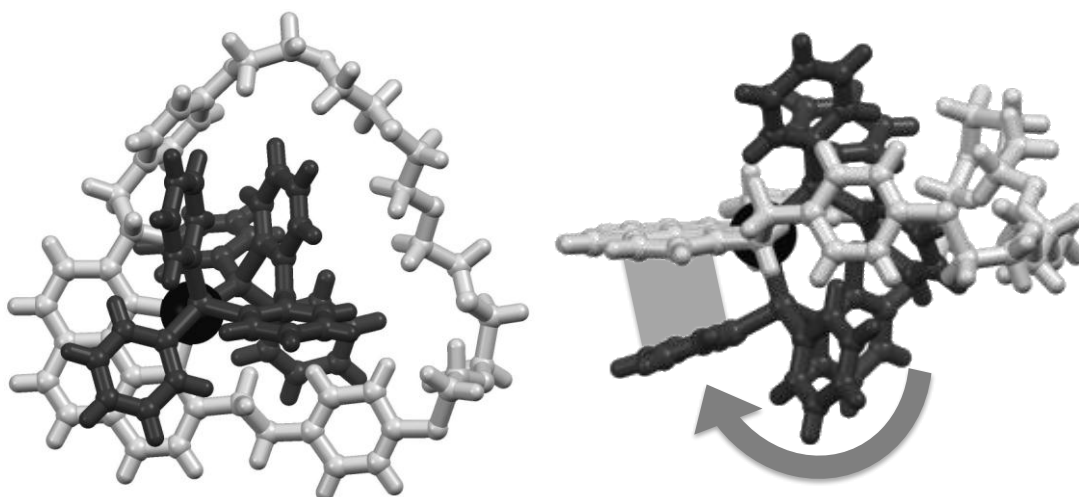
Figure 9. Top and side views of the X-ray crystal structure of [Cu( m37 )(POP)]BF 4 ( m37 : pale gray, POP: dark gray, Cu: black), the counteranion is omitted. The rocking of the POP ligand allowing the establishment of an intramolecular \pi - \pi interaction between a phenyl ring of the POP ligand and the phenanthroline moiety of m37 is highlighted (right).
