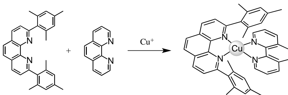
Figure 2. Approach developed by Schmittel for the quantitative preparation of heteroleptic bis-phenanthroline Cu(I) complexes.
