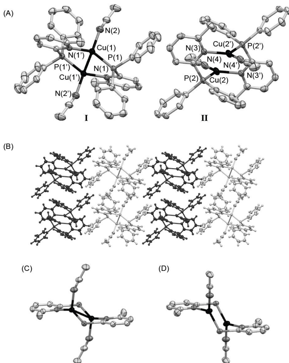
Figure 2. (A) X-ray crystal structure of [\text{Cu}_2(\mu\text{-dpPyMe})_2(\text{CH}_3\text{CN})_2](\text{BF}_4)_2 (view down crystallographic axis b ), two conformers ( I and II ) are observed in the crystal. (B) View of the packing down crystallographic axis b revealing alternating layers of the two conformers ( I : pale gray, II : dark gray). Views of the chair-like conformations adopted by I (C) and II (D).
