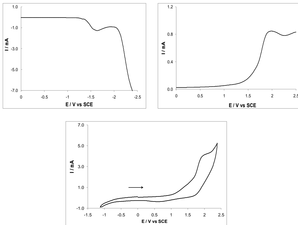
Figure 9. Top: OSWVs (cathodic and anodic scans) of compound 2 on a Pt electrode in \text{CH}_2\text{Cl}_2 + 0.1 \text{ M } n\text{Bu}_4\text{NBF}_4 at room temperature. Bottom: cyclic voltammogram showing the oxidation of 2 at v = 0.1 \text{ V}\cdot\text{s}^{-1} on a Pt electrode in \text{CH}_2\text{Cl}_2 + 0.1 \text{ M } n\text{Bu}_4\text{NBF}_4 .
