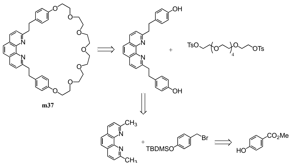
Figure 7. Structure of m37 and the proposed retrosynthetic scheme for its synthesis.
