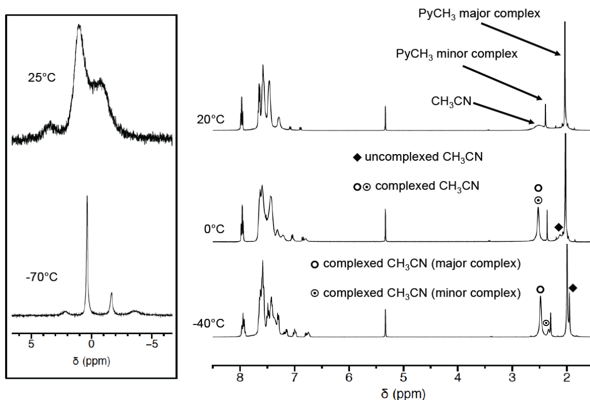
Figure 3. 1 H and 31 P NMR spectra (CD 2 Cl 2 ) recorded upon dissolution of the crystallized sample of [Cu 2 (μ-dpPyMe) 2 (CH 3 CN) 2 ](BF 4 ) 2 . Variable temperature studies reveal the presence of several species in solution.
