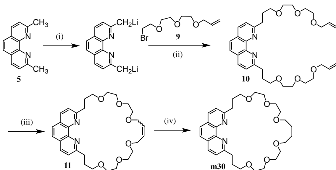
Scheme 5. Reagents and conditions: (i) LDA, THF, (ii) 9 , THF (41%); (iii) first generation Grubbs' catalysts, \text{CH}_2\text{Cl}_2 (86%); (iv) \text{H}_2 , Pd/C, THF (60%).
