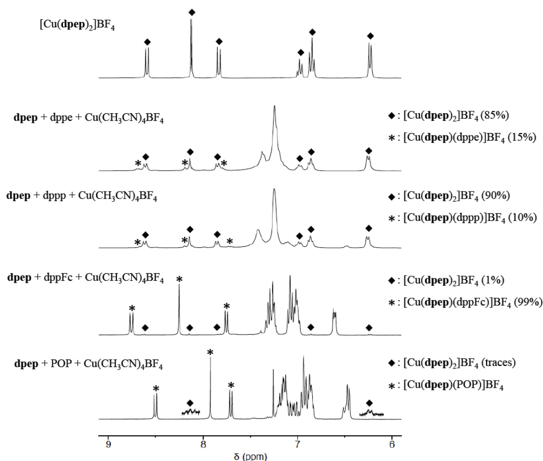
Figure 6. Aromatic region of the ^1\text{H} NMR spectra of the crude products obtained after the treatment of various PP ligands with \text{Cu}(\text{CH}_3\text{CN})_4\text{BF}_4 and dpep . For comparison purposes, the ^1\text{H} NMR spectrum of [\text{Cu}(\text{dpep})_2]\text{BF}_4 (top) is also represented.
