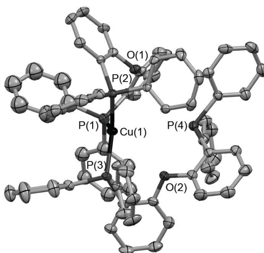
Figure 13. ORTEP plot of the structure of [\text{Cu}(\text{POP})_2]\text{BF}_4 . The H atoms and the counteranion are omitted for clarity, thermal ellipsoids are drawn at the 50% probability level. Selected bond lengths: Cu(1)-P(1): 2.273(1), Cu(1)-P(2): 2.261(1), Cu(1)-P(3): 2.263(1) Å; selected bond angles: P(1)-Cu(1)-P(2): 114.03(6), P(1)-Cu(1)-P(3): 121.49(6), P(2)-Cu(1)-P(3): 121.90(6)°. P(4) is at a non bonding distance from the Cu center (3.96 Å).
