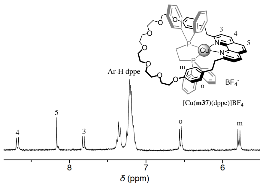
Figure 8. Aromatic region of the ^1\text{H} NMR spectrum ( \text{CD}_2\text{Cl}_2 , 300 MHz) of [\text{Cu}(\mathbf{m37})(\text{dppe})]\text{BF}_4 .
