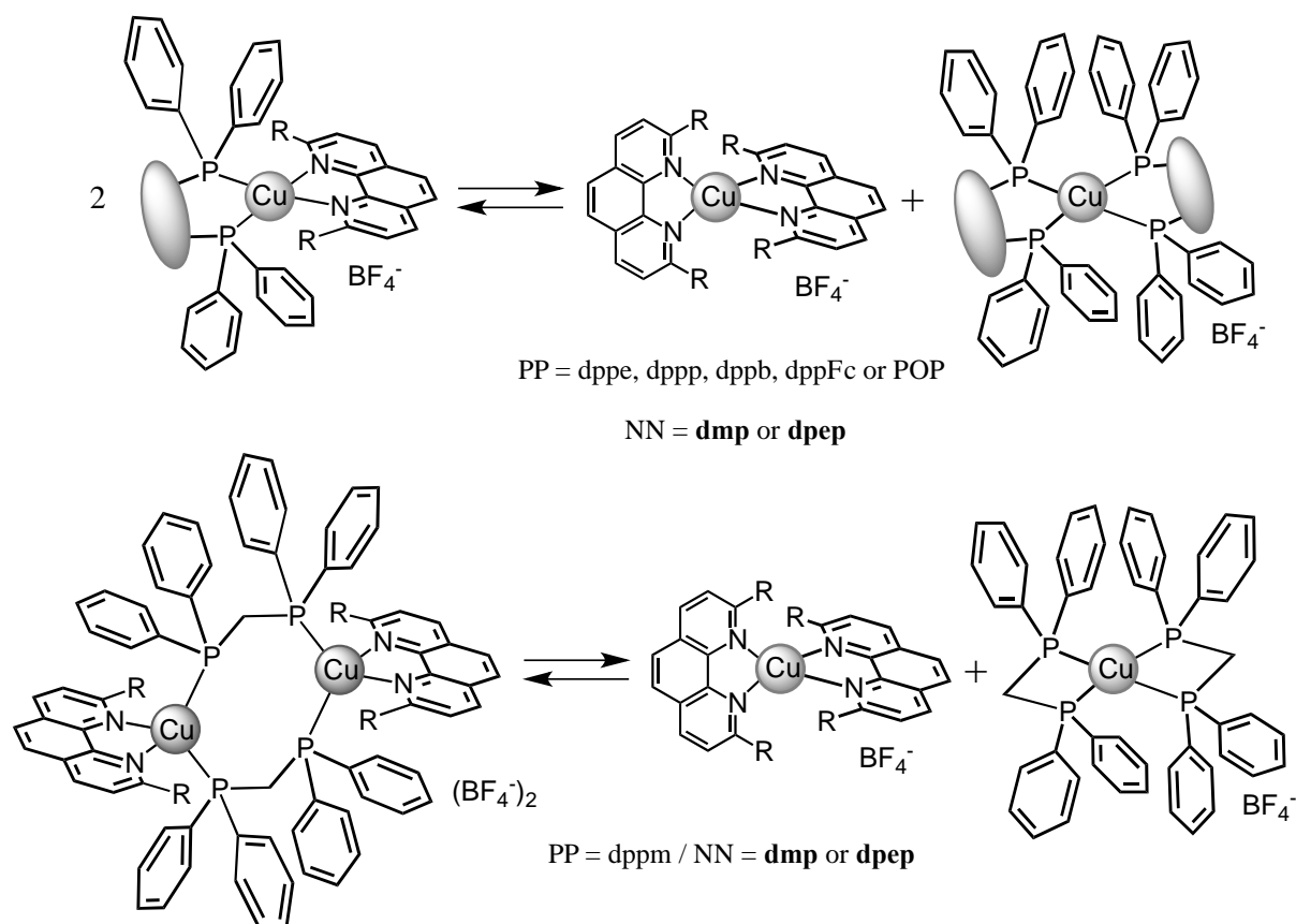
Figure 8. Dynamic equilibrium evidenced in solution between the heteroleptic complexes and their corresponding homoleptic species.
