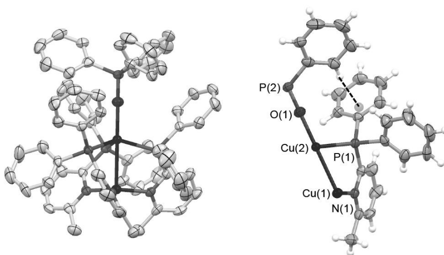
Figure 6. ORTEP plots of the [\text{Cu}_2(\mu\text{-dpPyMe})_3(\text{L})]^{2+} dication observed in the structure of 5 . \text{CHCl}_3 (the H atoms are omitted for clarity, thermal ellipsoids are drawn at the 50% probability level). Left: complete structure of the dication; right: asymmetric unit. An intramolecular C-H \pi interaction is highlighted (dashed line). Selected bond lengths: Cu(1)-N(1): 2.055(7), Cu(2)-P(1): 2.316(2), Cu(2)-O(1): 2.060(9) Å. Selected bond angles: N(1)-Cu(1)-N(1'): 119.6(3), P(1)-Cu(2)-P(1'): 114.44(9), P(1)-Cu(2)-O(2): 103.9(3).
