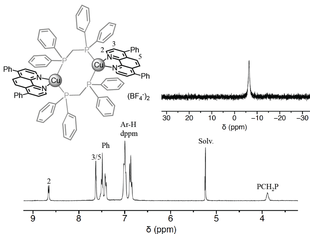
Figure 4. ^1\text{H} (bottom) and ^{31}\text{P} (top right) NMR spectra of [\text{Cu}_2(\text{Bphen})_2(\mu\text{-dppm})_2](\text{BF}_4)_2 recorded in \text{CD}_2\text{Cl}_2 at room temperature.
