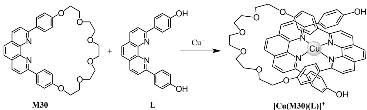
Figure 1. Approach developed by Sauvage for the quantitative preparation of heteroleptic bis-phenanthroline Cu(I) complexes.
