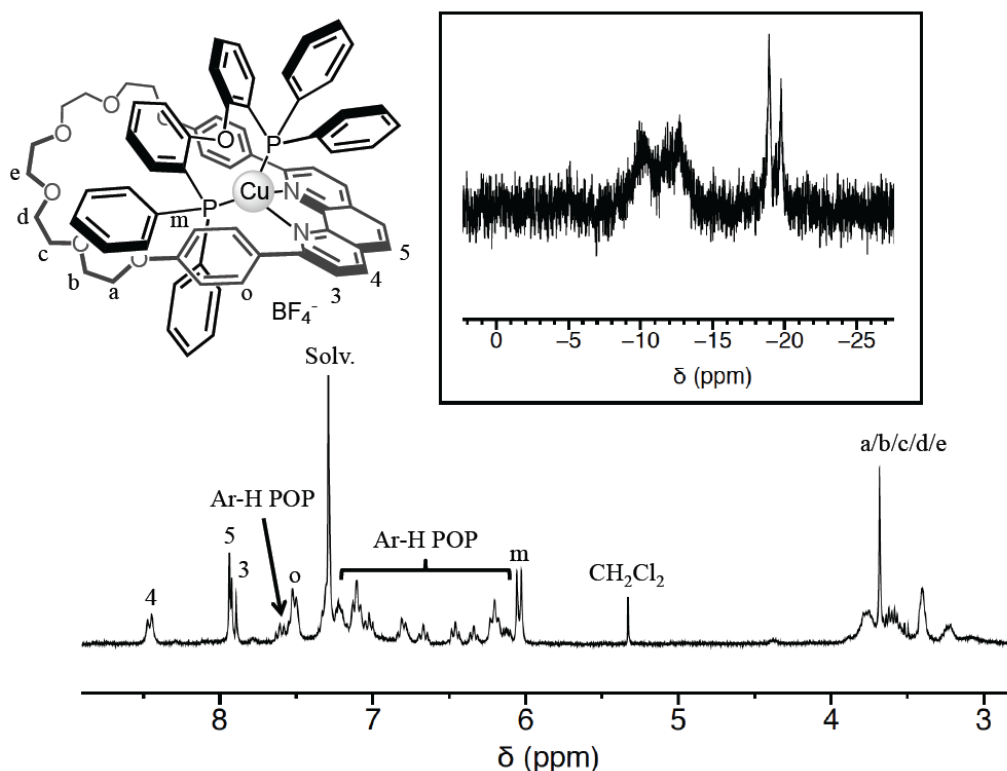
Figure 4. 1 H and 31 P NMR spectra (CDCl 3 ) of [Cu( M30 )(POP)]BF 4 .
