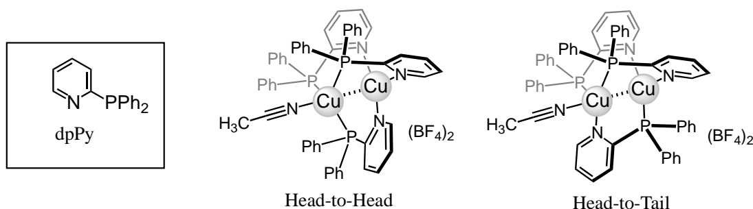
Figure 1. The two isomeric forms of [\text{Cu}_2(\mu\text{-dpPy})_3] (\text{BF}_4)_2 obtained from the reaction of dpPy and \text{Cu}(\text{CH}_3\text{CN})_4\text{BF}_4 in a 3:2 ratio. 6
