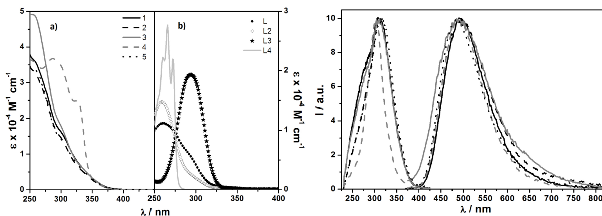
Figure 10. Left: electronic absorption spectra of (a) complexes 1-5 (solid-black, dashed-black, solid-grey, dashed-grey, dotted-black, respectively) and (b) ligands L (dots), L2 (squares), L3 (stars) and L4 (solid-grey) in CH 2 Cl 2 . Right: excitation and emission spectra of complexes 1-5 (solid-black, dashed-black, solid-grey, dashed-grey, dotted-black, respectively, uncorrected) in degassed CH 2 Cl 2 . Emission spectra are recorded upon exciting 1 and 3 at 320 nm, and 2 , 4 and 5 at 340 nm. Excitation spectra are collected at the respective emission maximum for each complex.
