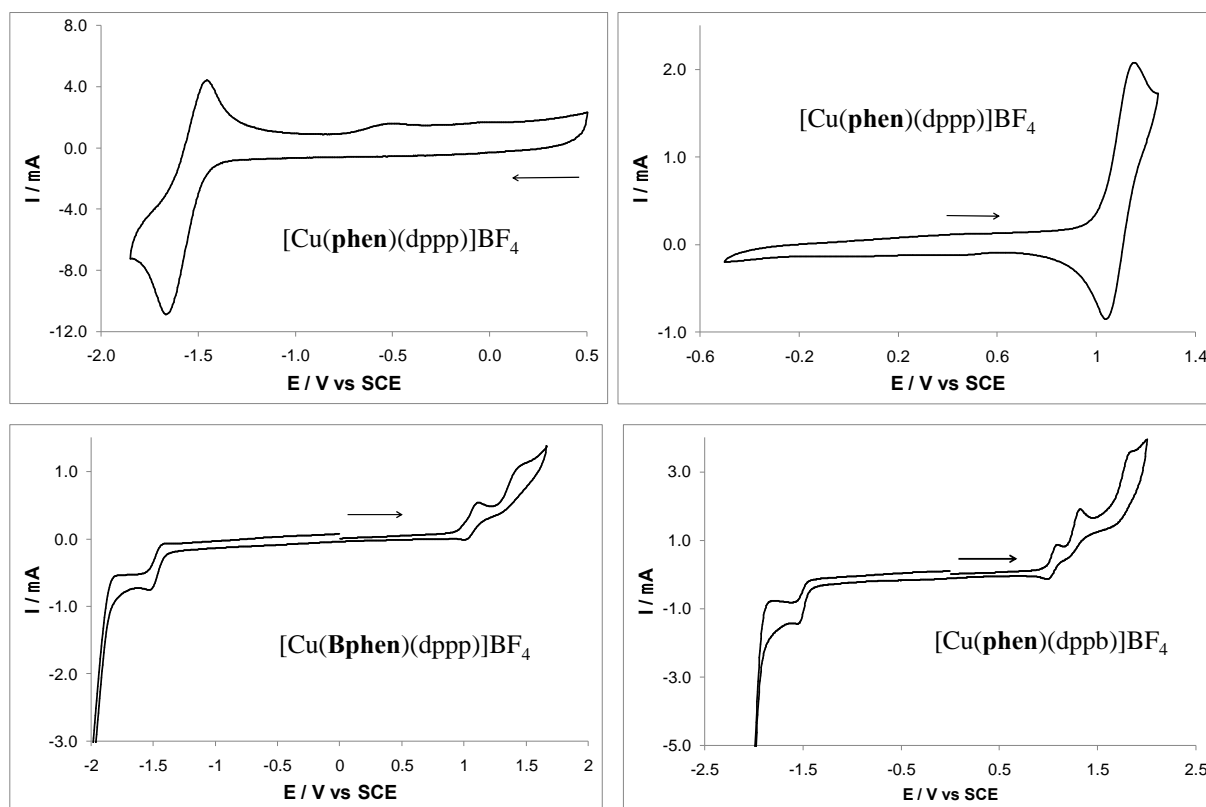
Figure 15. Typical examples of cyclic voltammograms on a Pt electrode in CH 2 Cl 2 + 0.1 M n Bu 4 NBF 4 (top left: v = 20 \text{ Vs}^{-1} , top right: v = 10 \text{ Vs}^{-1} , bottom left: v = 0.1 \text{ Vs}^{-1} , bottom right: v = 0.1 \text{ Vs}^{-1} ).
