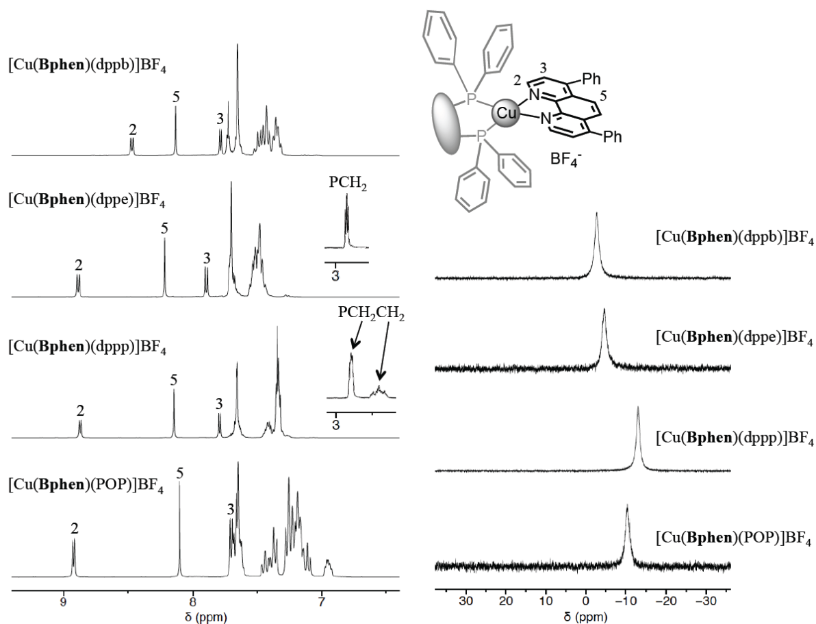
Figure 2. ^1\text{H} (left) and ^{31}\text{P} (right) NMR spectra of [\text{Cu}(\text{Bphen})(\text{PP})]^+ (PP = dppb, dppe, dppp and POP) recorded in \text{CD}_2\text{Cl}_2 at room temperature.
