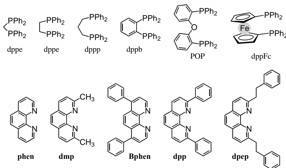
Figure 1. The library of NN and PP ligands used for the preparation of heteroleptic [\text{Cu}(\text{NN})(\text{PP})]^+ derivatives.
