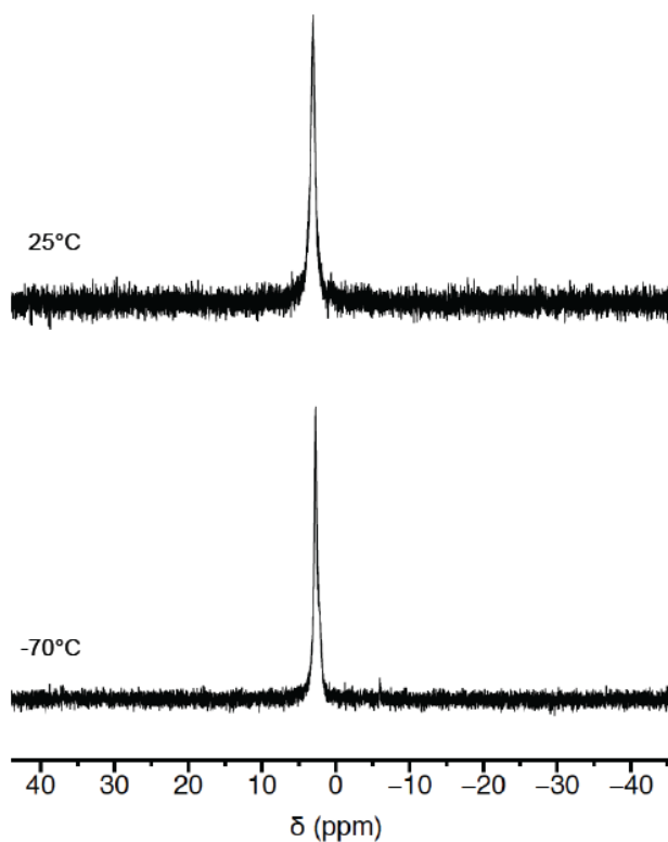
Figure 8. Top: 31 P NMR spectra of 6 recorded at different temperature in CD 2 Cl 2 .
