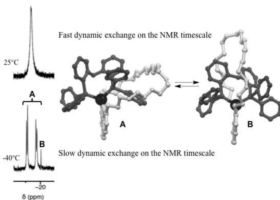
Figure 13. 31 P NMR spectra (CD 2 Cl 2 , 162 MHz) of [Cu( m30 )(POP)]BF 4 recorded at different temperatures revealing a dynamic exchange between different topomers, i.e. topomerization.
