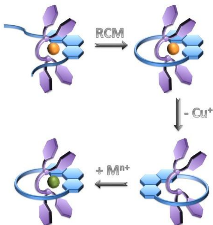
Figure 16. Proposed synthetic strategy for the preparation of rotaxane ligands containing both phenanthroline and bis-phosphine chelating subunits.
