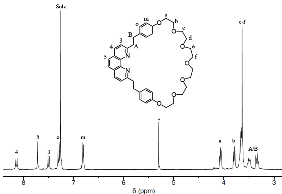
Figure 7. 1 H NMR spectrum (CDCl 3 , 300 MHz) of m37 (* = CH 2 Cl 2 ).
