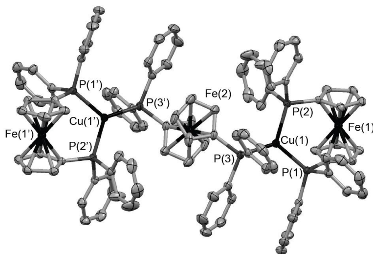
Figure 14. ORTEP plot of the structure of [\text{Cu}_2(\text{dppFc})_3](\text{BF}_4)_2 \cdot (\text{H}_2\text{O})_2 \cdot \text{CH}_2\text{Cl}_2 . The H atoms, the solvent molecules and the counteranions are omitted for clarity, thermal ellipsoids are drawn at the 50% probability level. Selected bond lengths: Cu(1)-P(1): 2.264(1), Cu(1)-P(2): 2.274(1), Cu(1)-P(3): 2.248(2) Å; selected bond angles: P(1)-Cu(1)-P(2): 111.75(5), P(1)-Cu(1)-P(3): 122.48(5), P(2)-Cu(1)-P(3): 125.02(5)°.
