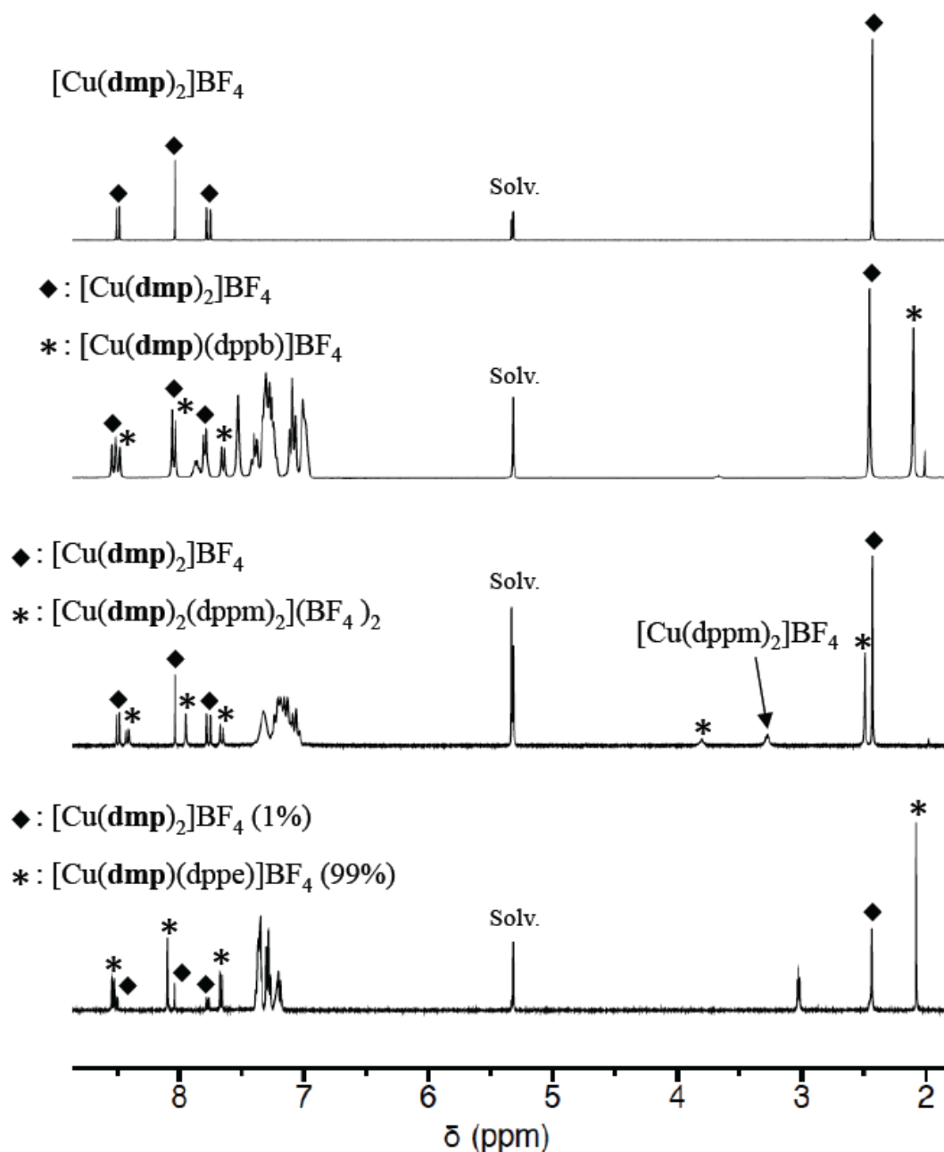
Figure 9. ^1\text{H} NMR (CD 2 Cl 2 ) recorded upon dissolution of recrystallized samples of [\text{Cu}_2(\text{dmp})_2(\mu\text{-dppm})_2](\text{BF}_4)_2 , [\text{Cu}(\text{dmp})(\text{dppe})]\text{BF}_4 , and [\text{Cu}(\text{dmp})(\text{dppb})]\text{BF}_4 . In all the cases, ligand exchange reactions take place and the typical resonances of [\text{Cu}(\text{dmp})_2]\text{BF}_4 are clearly observed. For comparison purposes, the ^1\text{H} NMR spectrum of [\text{Cu}(\text{dmp})_2]\text{BF}_4 (top) is also represented.
