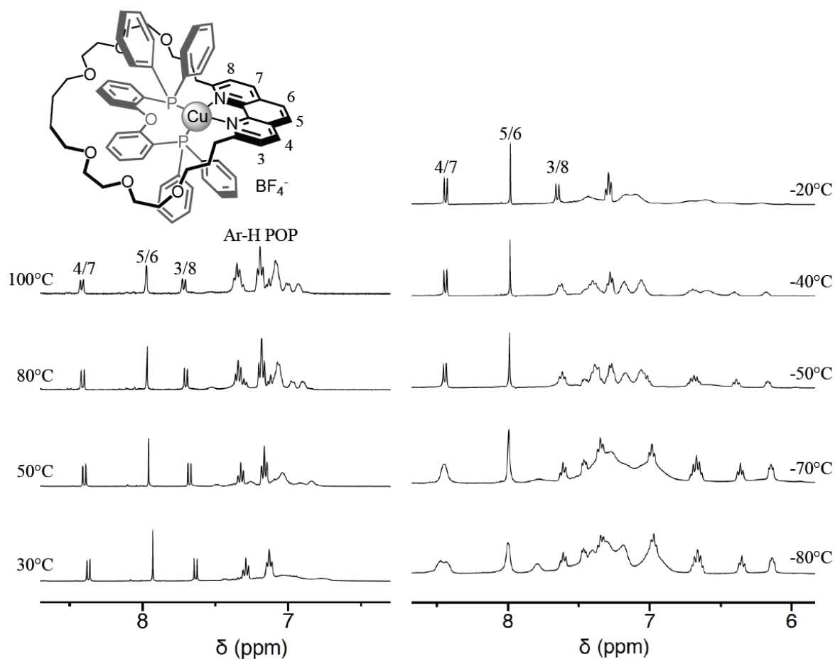
Figure 15. 1 H NMR spectra of [Cu( m30 )(POP)]BF 4 recorded at different temperatures in CDCl 2 CDCl 2 (left) and CD 2 Cl 2 (right).
