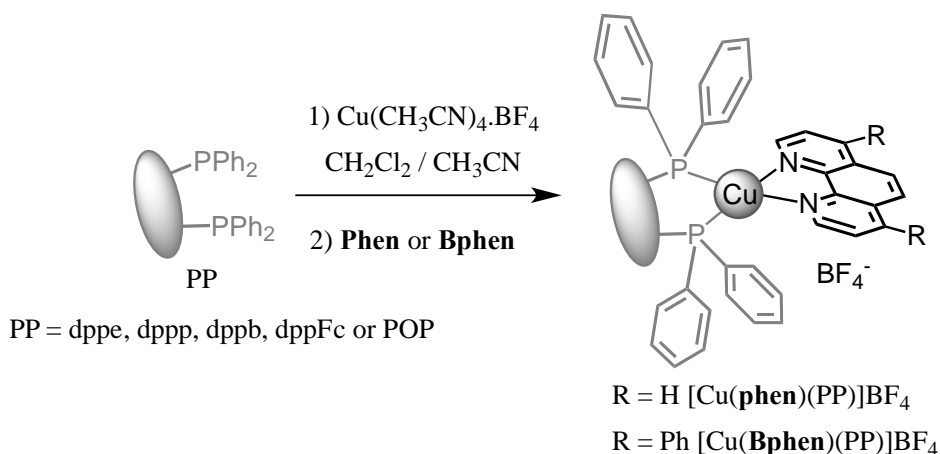
Scheme 1. Preparation of heteroleptic [\text{Cu}(\text{NN})(\text{PP})]^+ derivatives from phen and Bphen .
