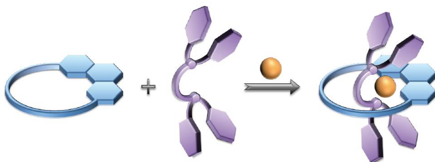
Figure 3. Proposed concept for the preparation of stable [\text{Cu}(\text{phen})(\text{PP})]^+ derivatives based on the approach using topological constraints developed by Sauvage.
