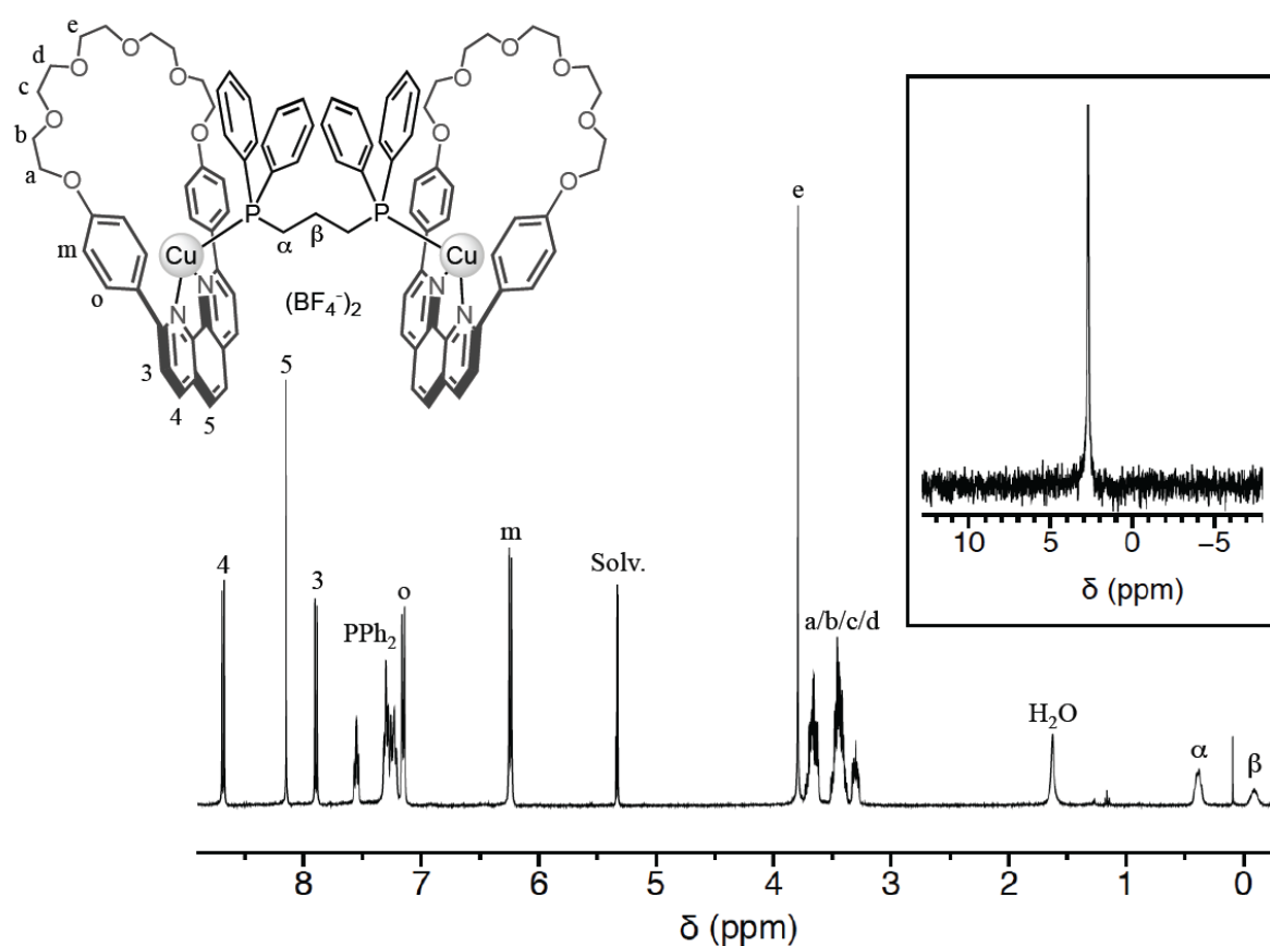
Figure 6. 1 H and 31 P NMR spectra (CD 2 Cl 2 ) of [Cu 2 ( M30 ) 2 (μ-dppp)](BF 4 ) 2 .
