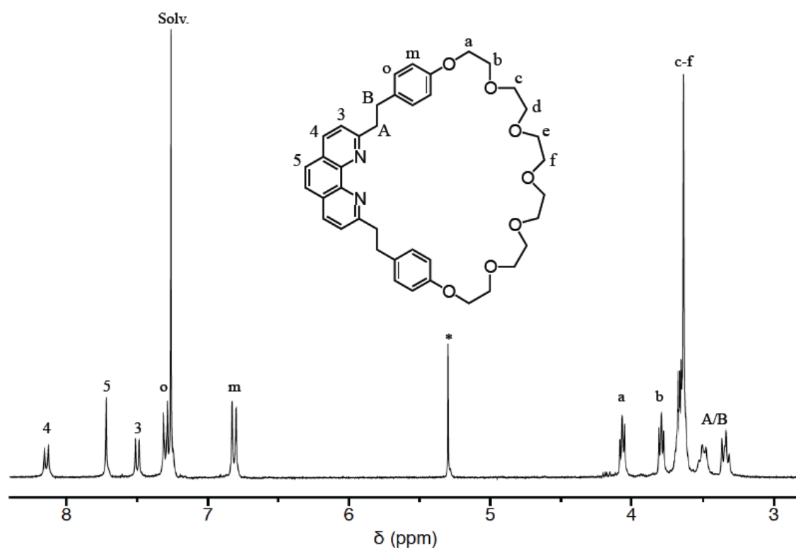
Figure 7. 1 H NMR spectrum (CDCl 3 , 300 MHz) of m37 (* = CH 2 Cl 2 ).
