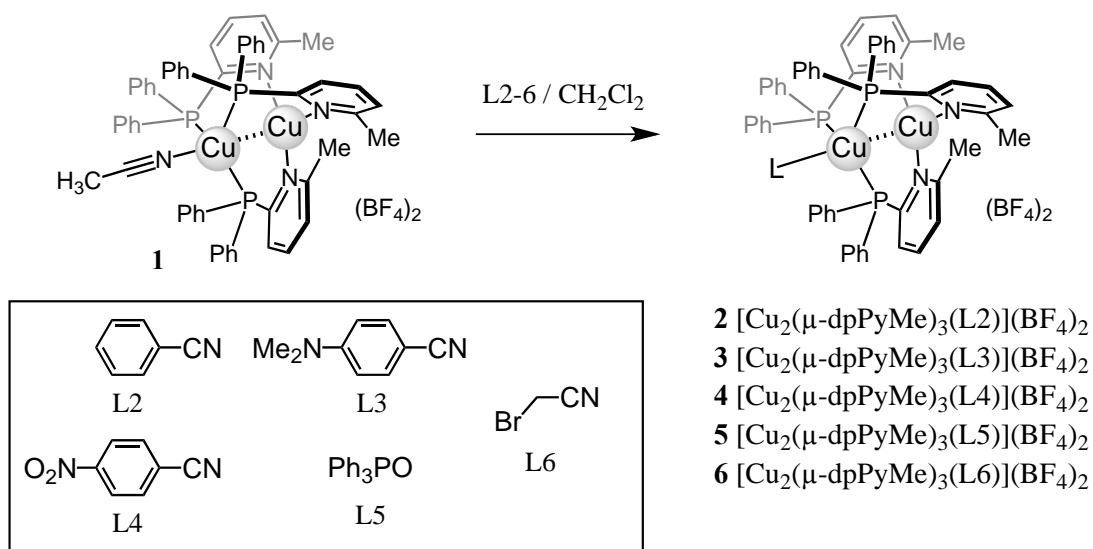
Scheme 1. Ligand exchange reactions.
