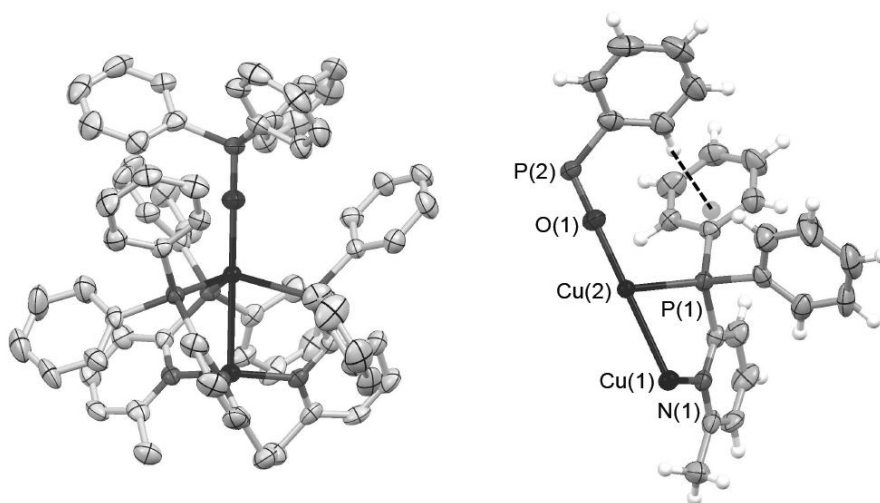
Figure 6. ORTEP plots of the [\text{Cu}_2(\mu\text{-dpPyMe})_3(\text{L})]^{2+} dication observed in the structure of 5 .CHCl 3 (the H atoms are omitted for clarity, thermal ellipsoids are drawn at the 50% probability level). Left: complete structure of the dication; right: asymmetric unit. An intramolecular C-H \pi interaction is highlighted (dashed line). Selected bond lengths: Cu(1)-N(1): 2.055(7), Cu(2)-P(1): 2.316(2), Cu(2)-O(1): 2.060(9) Å. Selected bond angles: N(1)-Cu(1)-N(1'): 119.6(3), P(1)-Cu(2)-P(1'): 114.44(9), P(1)-Cu(2)-O(2): 103.9(3).
