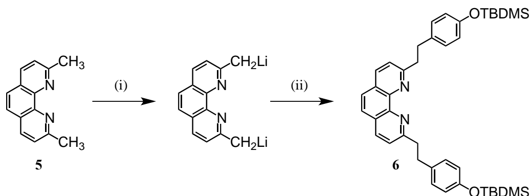
Scheme 2. Reagents and conditions: (i) LDA, THF, (ii) 4 , THF (38%).
