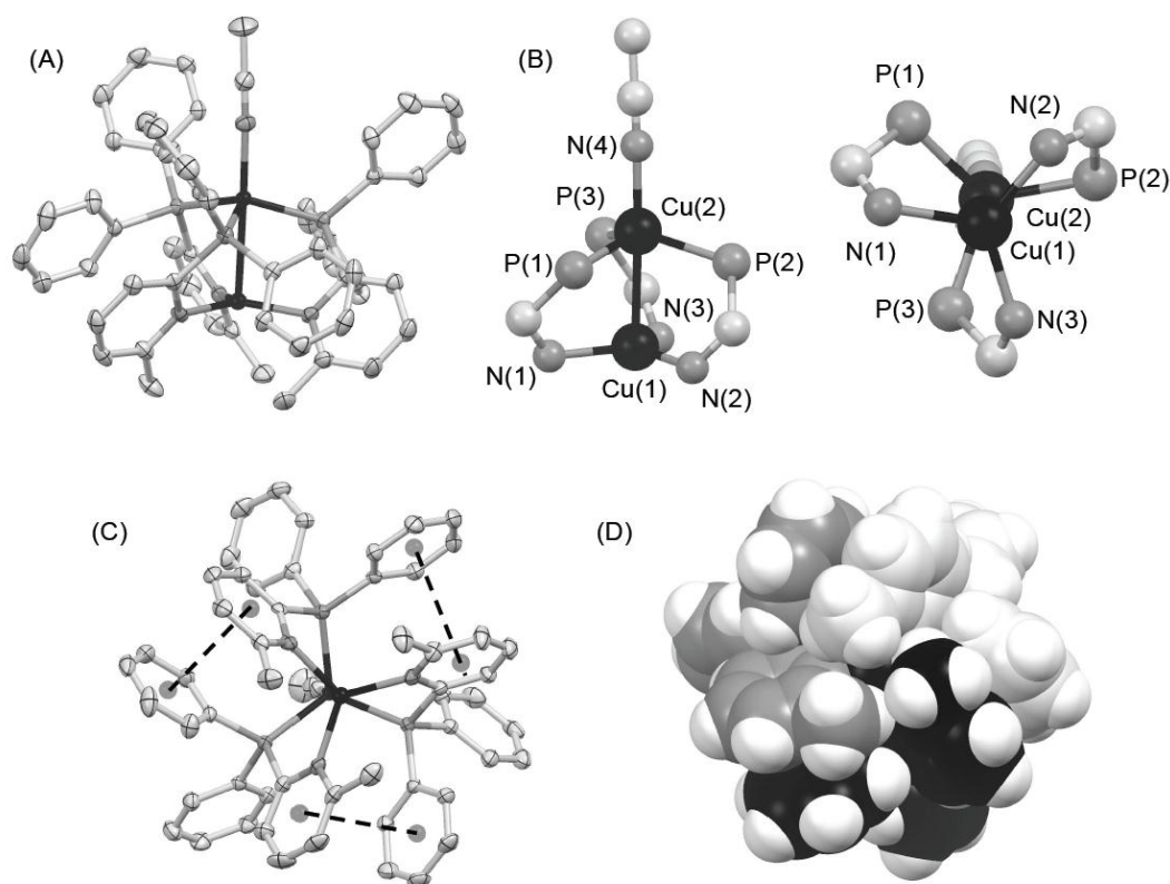
Figure 4. (A) ORTEP plot of the [\text{Cu}_2(\mu\text{-dpPyMe})_3(\text{CH}_3\text{CN})]^{2+} dication observed in the structure of 1 . (\text{CH}_2\text{Cl}_2)_2 (the H atoms are omitted for clarity, thermal ellipsoids are drawn at the 50% probability level). (B) Two views showing the details of the coordination sphere around the two metal centers. (C) View highlighting the interligand \pi - \pi interactions in the [\text{Cu}_2(\mu\text{-dpPyMe})_3(\text{CH}_3\text{CN})]^{2+} dication. (D) View along the Cu(1)-Cu(2) axis showing the shielding of Cu(1) due to the presence of the CH 3 groups.
