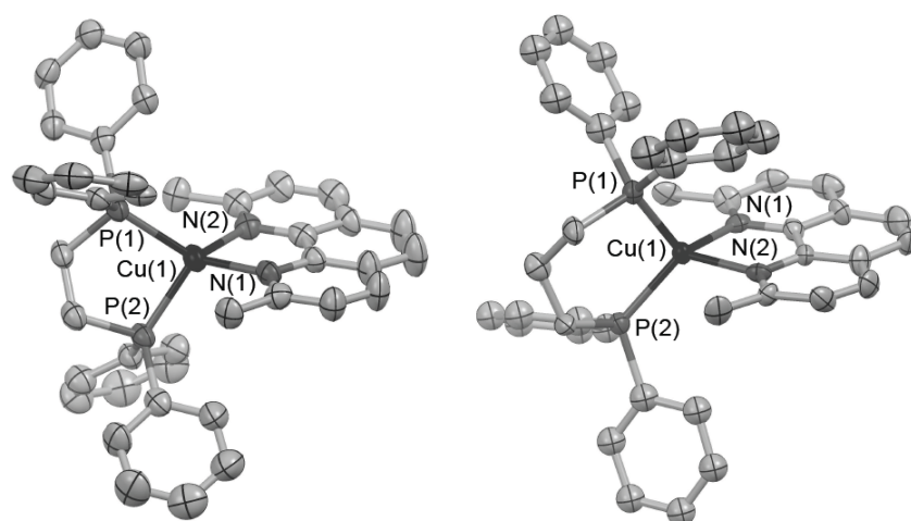
Figure 7. ORTEP plot of the structures of [Cu( dmp )(dppe)]BF 4 .Et 2 O (left) and [Cu( dmp )(dppp)]BF 4 (right). The H atoms, the solvent in the case of dppe, and the counteranion are omitted for clarity, thermal ellipsoids are drawn at the 50% probability level.
