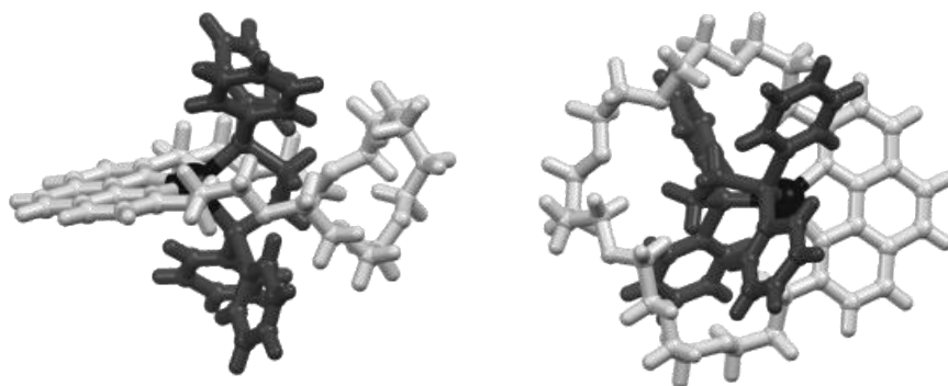
Figure 10. Top and side views of the X-ray crystal structure of [Cu( m30 )(dppe)]BF 4 ( m30 : pale gray, dppe: dark gray, Cu: black, the counteranion is omitted).
