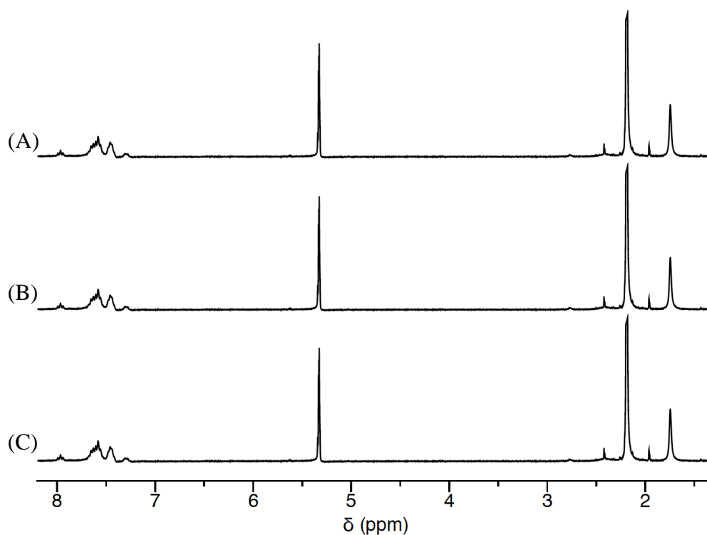
Figure 11. 1 H NMR (CD 2 Cl 2 ) of the crude reaction mixtures obtained after evaporation. (A) dpPyMe (1 equiv.) and Cu(CH 3 CN) 4 BF 4 (1 equiv.), (B) dpPyMe (3 equiv.) and Cu(CH 3 CN) 4 BF 4 (2 equiv.), (C) dpPyMe (2 equiv.) and Cu(CH 3 CN) 4 BF 4 (1 equiv.).
