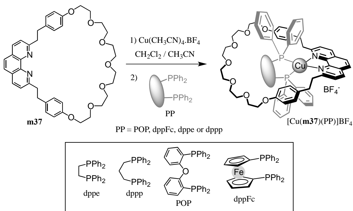
Scheme 4. Preparation of pseudo-rotaxanes [Cu( m37 )(PP)]BF 4 from m37 and various bis-diphenylphosphino-bridged ligands (dppe: 59%, dppp: 61%, POP: 85%, dppFc: 81%).
