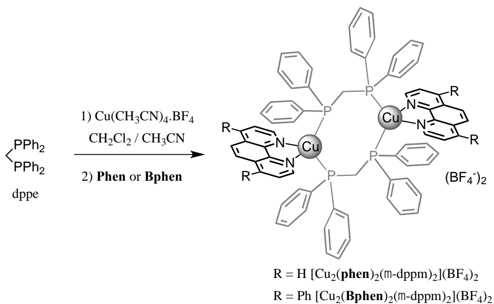
Scheme 2. Preparation of [\text{Cu}_2(\text{phen})_2(\mu\text{-dppm})_2](\text{BF}_4)_2 and [\text{Cu}_2(\text{Bphen})_2(\mu\text{-dppm})_2](\text{BF}_4)_2 .
