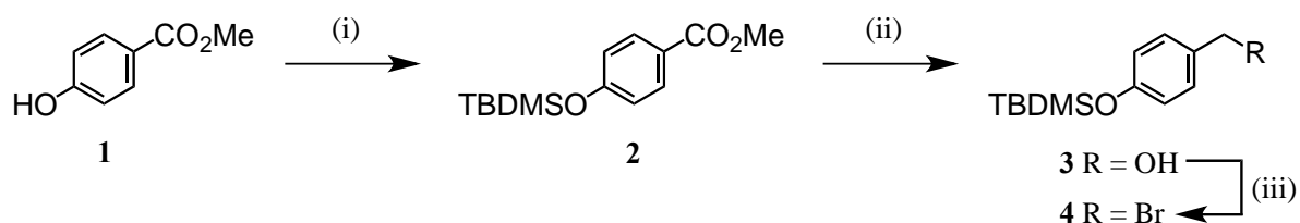
Scheme 1. Reagents and conditions: (i) TBDMSCl, Imidazole, DMF (98%); (ii) LiAlH 4 , THF (98%); (iii) TMSBr, CHCl 3 (72%)
