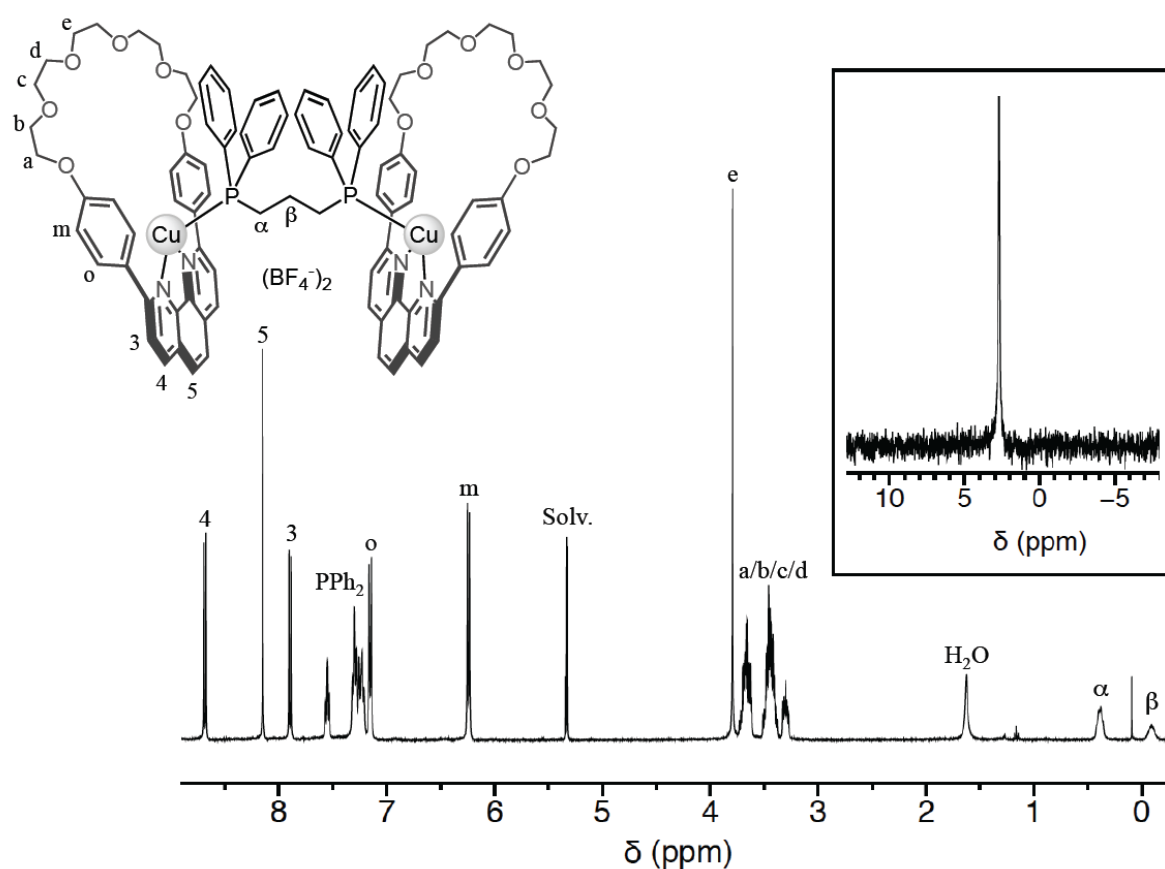
Figure 6. ^1\text{H} and ^{31}\text{P} NMR spectra ( \text{CD}_2\text{Cl}_2 ) of [\text{Cu}_2(\text{M30})_2(\mu\text{-dppp})](\text{BF}_4)_2 .
