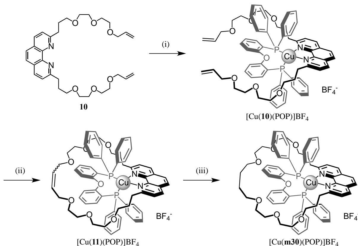
Scheme 7. Reagents and conditions: (i) POP, Cu(CH 3 CN) 4 BF 4 , CH 2 Cl 2 , CH 3 CN (85%); (ii) second generation Grubbs' catalysts, CH 2 Cl 2 (36%); (iii) H 2 , Pd/C, THF (40%).
