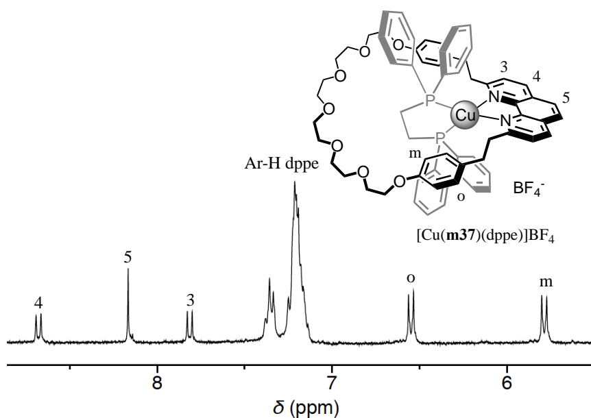
Figure 8. Aromatic region of the 1 H NMR spectrum (CD 2 Cl 2 , 300 MHz) of [Cu( m37 )(dppe)]BF 4 .
