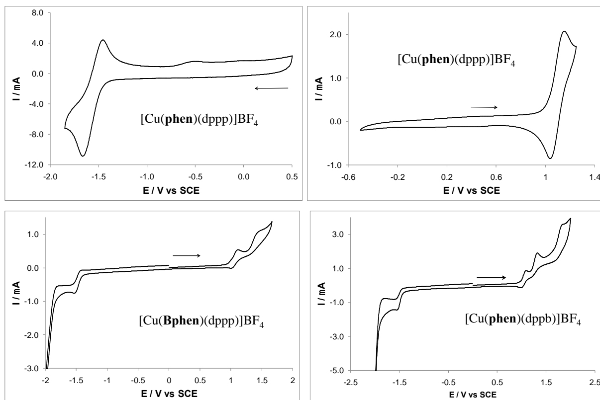
Figure 15. Typical examples of cyclic voltammograms on a Pt electrode in \text{CH}_2\text{Cl}_2 + 0.1 \text{ M } n\text{Bu}_4\text{NBF}_4 (top left: v = 20 \text{ Vs}^{-1} , top right: v = 10 \text{ Vs}^{-1} , bottom left: v = 0.1 \text{ Vs}^{-1} , bottom right: v = 0.1 \text{ Vs}^{-1} ).
