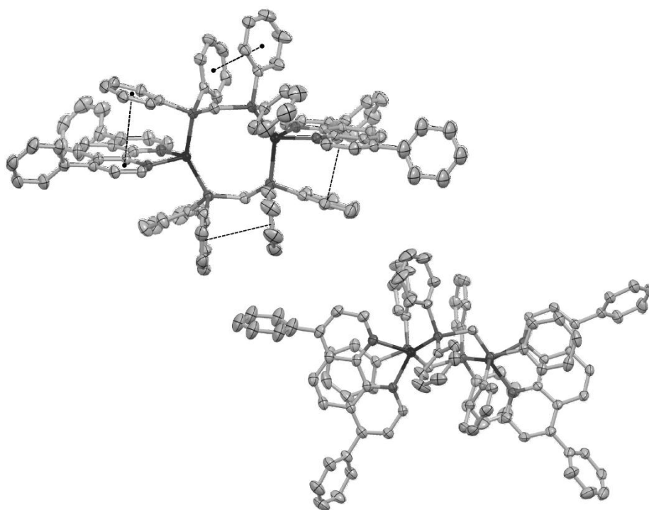
Figure 5A. Two views of the structure of [\text{Cu}_2(\text{Bphen})_2(\mu\text{-dppm})_2](\text{BF}_4)_2 \cdot \text{CH}_2\text{Cl}_2 (the H atoms, the counteranions and the \text{CH}_2\text{Cl}_2 molecule are omitted for clarity, thermal ellipsoids of the ORTEP plot are drawn at the 50% probability level).
