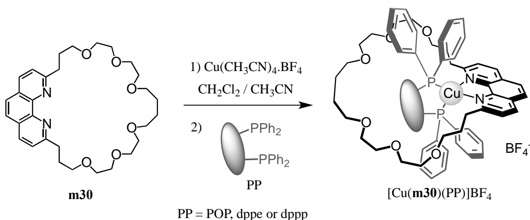
Scheme 6. Preparation of pseudo-rotaxanes [Cu( m30 )(PP)]BF 4 from m30 and various bis-phosphine ligands (dppe: 63%, dppp: 77%, POP: 75%).
