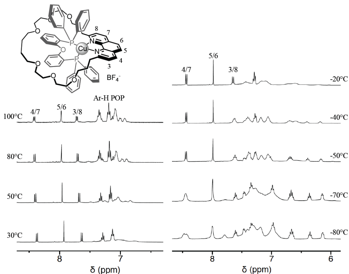
Figure 15. 1 H NMR spectra of [\text{Cu}(\text{m30})(\text{POP})]\text{BF}_4 recorded at different temperatures in \text{CDCl}_2\text{CDCl}_2 (left) and \text{CD}_2\text{Cl}_2 (right).
