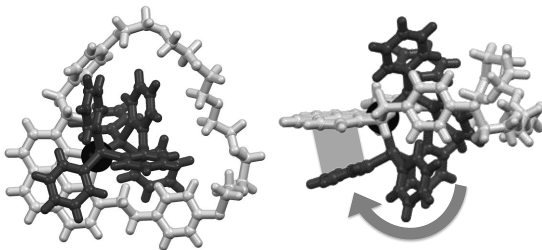
Figure 9. Top and side views of the X-ray crystal structure of [Cu( m37 )(POP)]BF 4 ( m37 : pale gray, POP: dark gray, Cu: black), the counteranion is omitted. The rocking of the POP ligand allowing the establishment of an intramolecular \pi - \pi interaction between a phenyl ring of the POP ligand and the phenanthroline moiety of m37 is highlighted (right).
