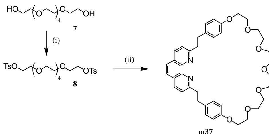
Scheme 3. Reagents and conditions: (i) TsCl, pyridine, DMAP, CH 2 Cl 2 (86%); (ii) 6 , CH 3 CN, CsF (18%)
