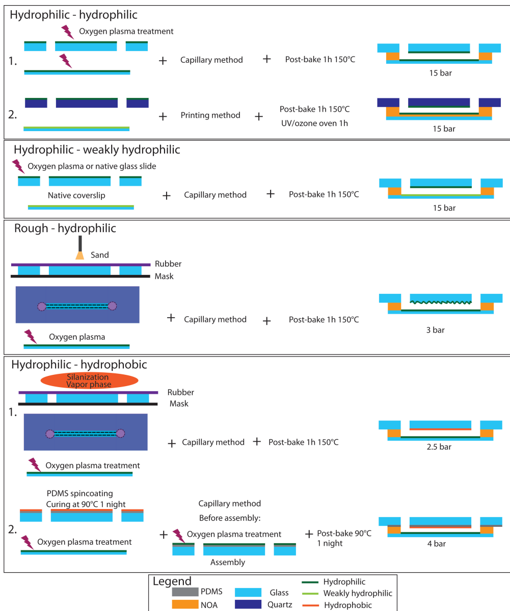
Figure 3.5 – Fabrication of microchannel with different wall wetting properties and roughness that sustain high pressure drops
