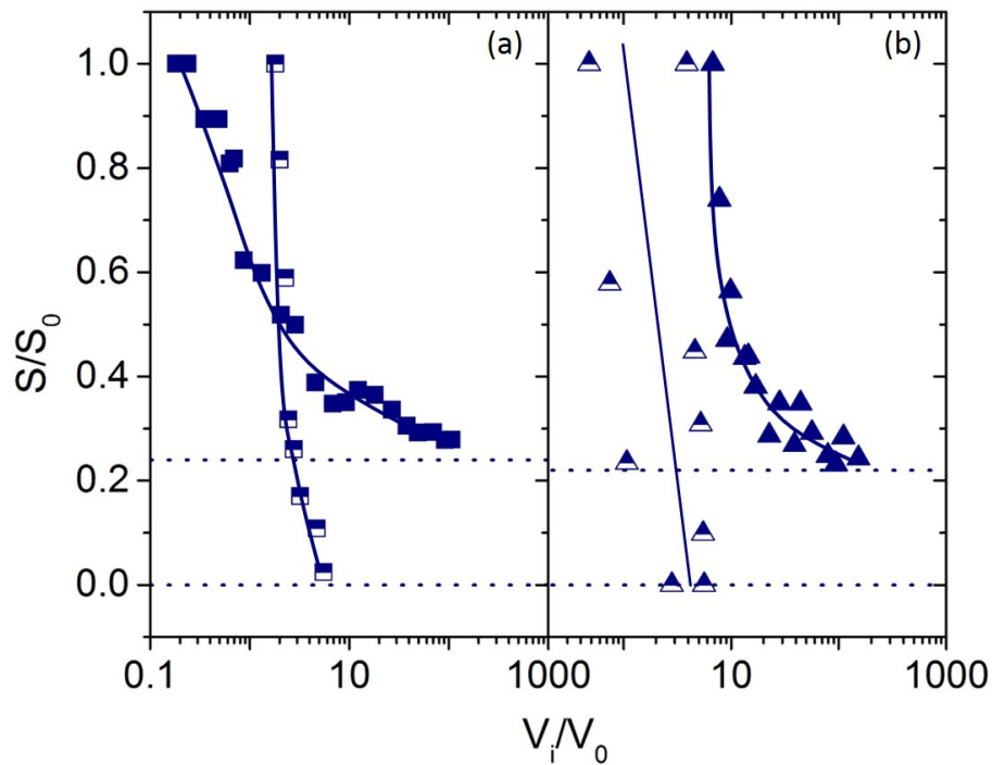
Figure 5.25 – Area of displaced fluid remaining in the corrugation scaled by the area of a corrugation as a function of the number of injected channel volume V_i/V_0 in the geometry A with no slip (full symbols) and with slip in the geometries A and B (half full symbols) for the displacement of (a) a microgel 2.2% (b) a microgel 3% with a microgel 1.6% at the highest velocity (0.8 bar). The solid lines are guides for the eyes.
