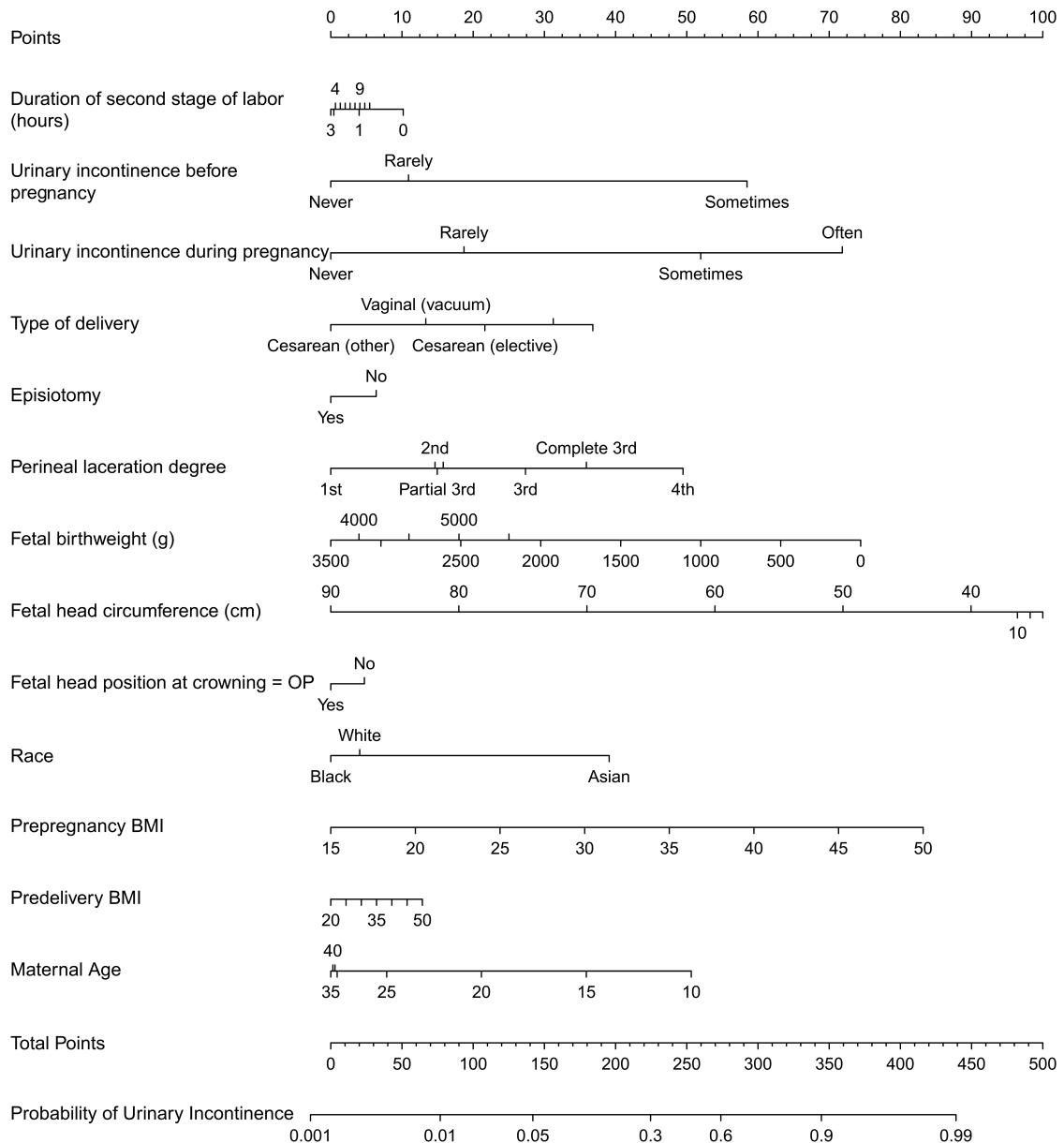
FIGURE 4. Nomogram for probability of developing UI after L&D. OP, occiput posterior.
