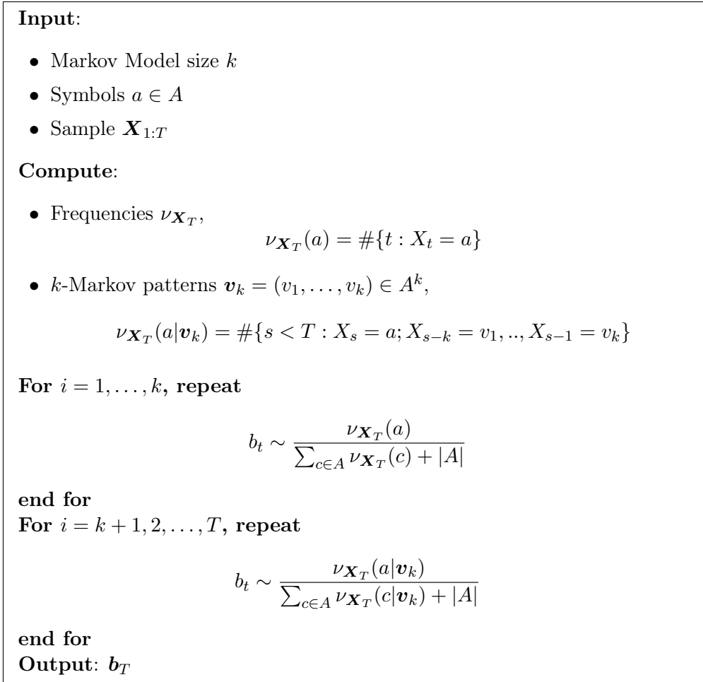
Figure 2.4: Markov Bootstrap Algorithm
