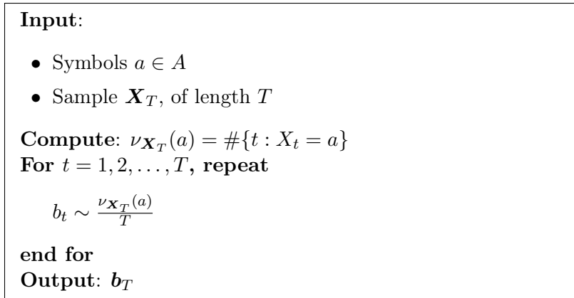
Figure 2.2: i.i.d. Bootstrap Algorithm
