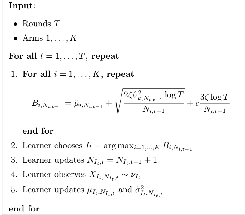
Figure 3.2: UCB-V
