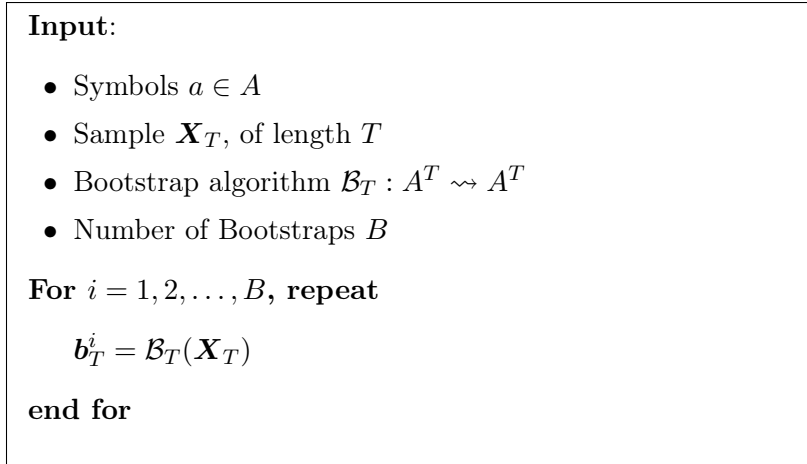
Figure 2.1: The Bootstrap Protocol
