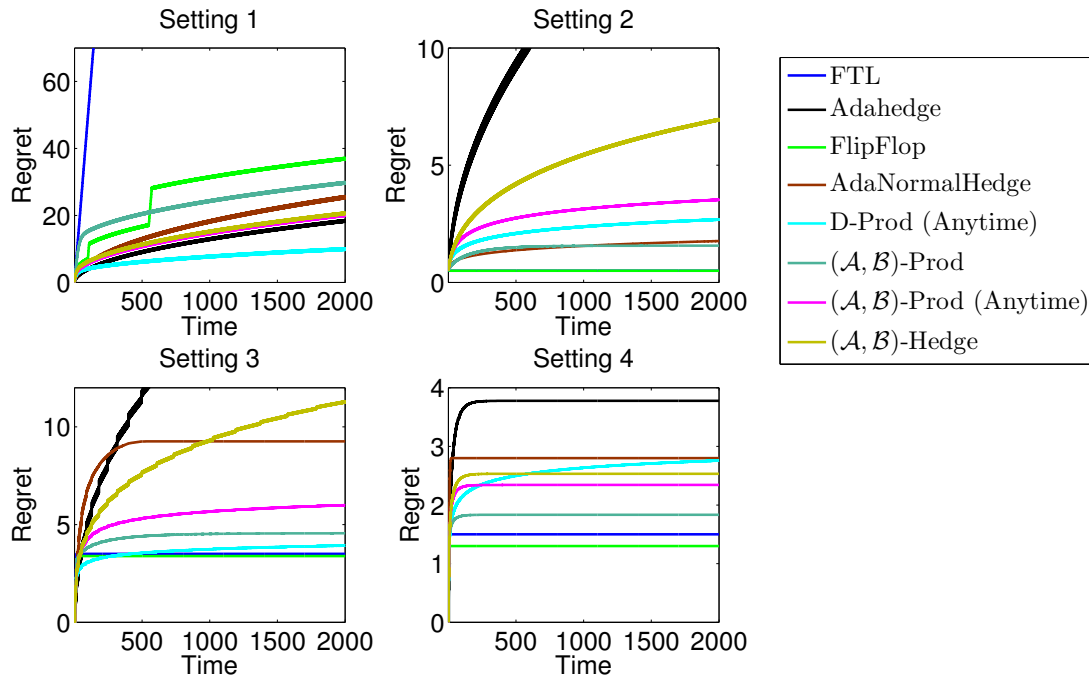
Figure 4.13: Hand tuned loss sequences from de Rooij et al. [2014]
