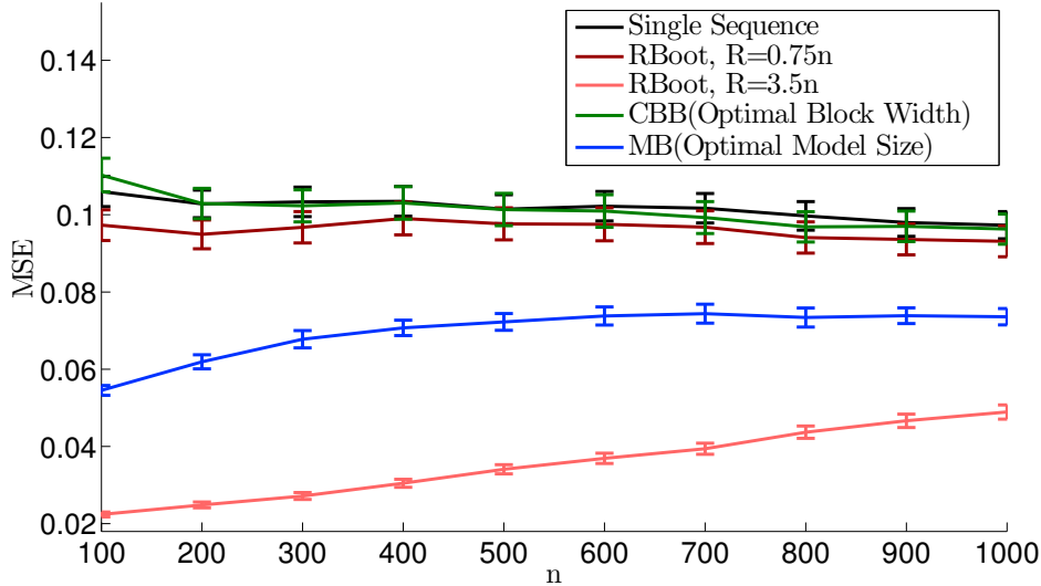
Figure 2.9: MSE on the FBM process for the maximum drawdown statistic.
