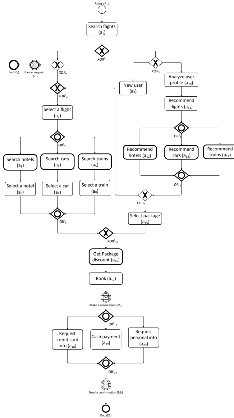
Figure 5.1: P^c : A configurable travel booking process
