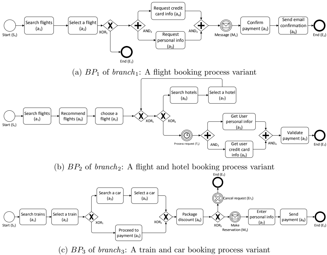
Figure 1.4: Three process variants of a travel booking process
