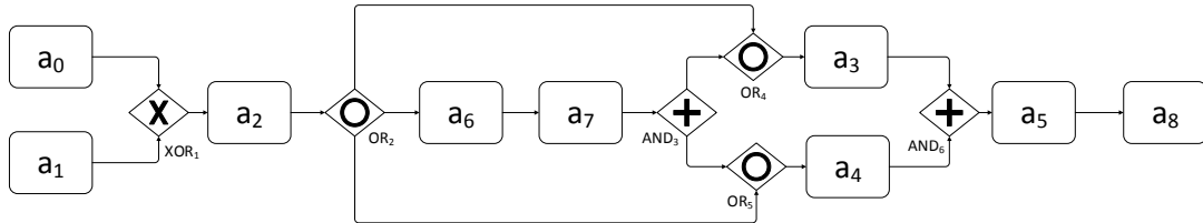
Figure 6.8: The process fragment discovered from the logs L_{a_{21}}^2 and L_{a_{42}}^2 in Table 6.3 and Table 6.4 respectively
