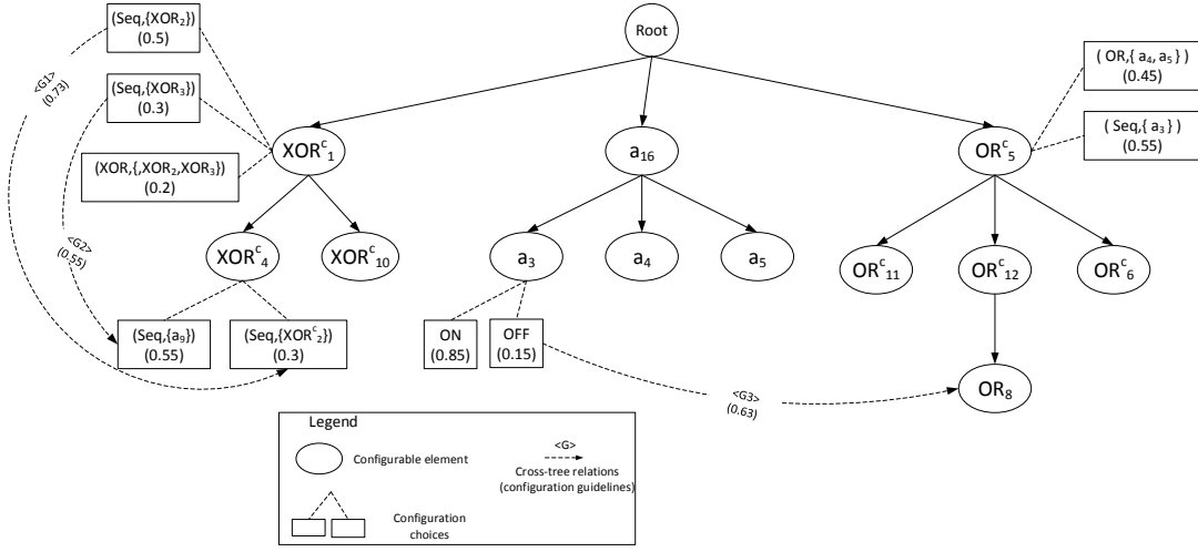
Figure 5.2: An excerpt of the configuration guidance model extracted for the configurable process model in Figure 5.1
