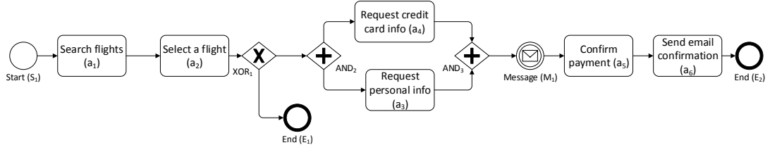
(a) BP_1 : A flight booking process variant
