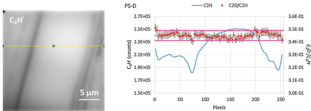
Fig. 3. On the left, scanning image (size = 25 μm × 25 μm) of C 2 H - on PS-D summed over 100 frames (from 40 to 139) when the plateau of Fig. 2 is reached, with a horizontal line profile (yellow line) of 3 pixels line width. On the right is the number of counts of C 2 H - secondary ion and C 2 D - /C 2 H - ratio, along the profile every 3 pixels. Error bars (in black) are at 2σ level. The mean value is calculated on the plateau and plotted as the orange dotted line. The pink lines represent the experimental standard deviation at 2σ level. (For interpretation of the references to color in this figure legend, the reader is referred to the web version of this article.)
