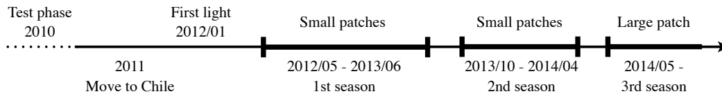
Figure 5.2: Timeline for the first campaign of the POLARBEAR experiment. I started to work on POLARBEAR in April 2012, just before the first season, and my thesis finishes at the end of 2015, at the end of the 3rd season of observation.
