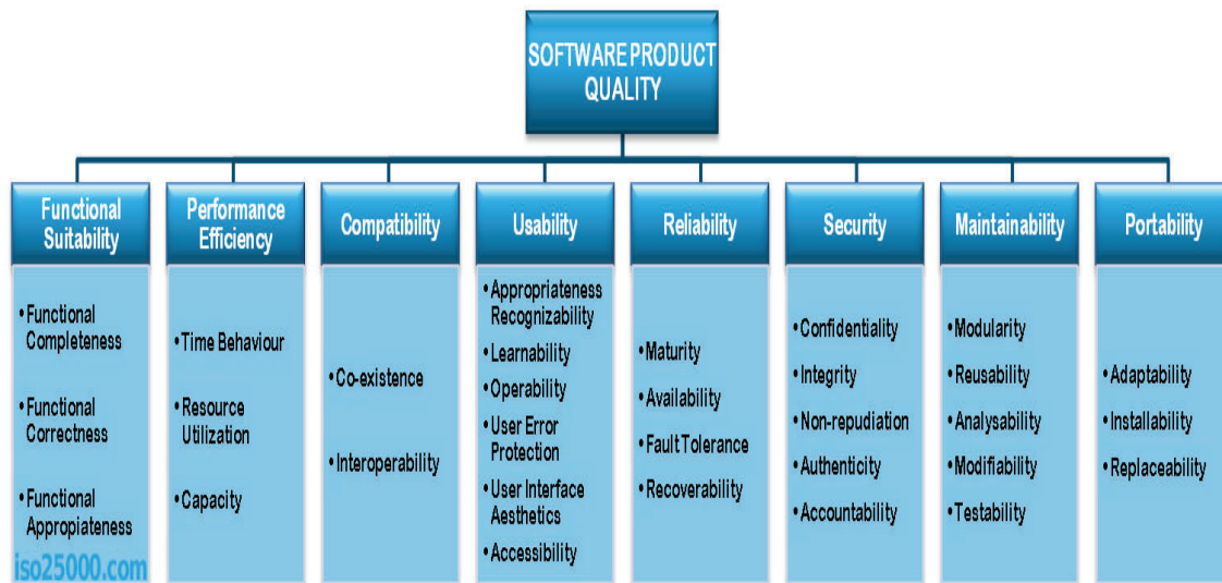
Fig. 3.23. ISO 25000 quality model
