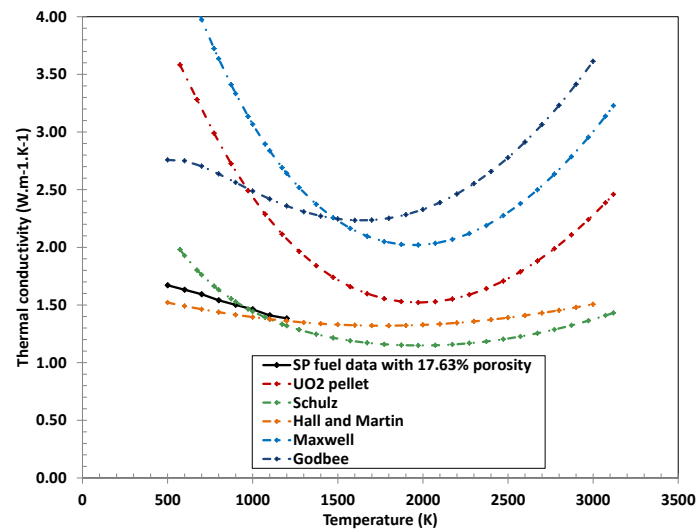
Figure 7-7. Thermal conductivity of \text{UO}_2 sphere-pac fuels of Figure 7-6 with various correlations. SP stands for sphere-pac.
