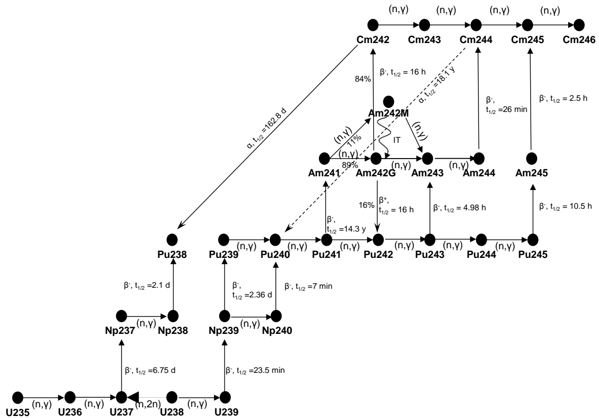
Figure 2-3. Uranium conversion chain (several \alpha -decay processes have been omitted for simplification).
