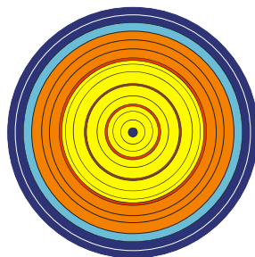
Figure 8-3. SIMMER-III radial layout of the CP-ESFR Working Horse core [13].
