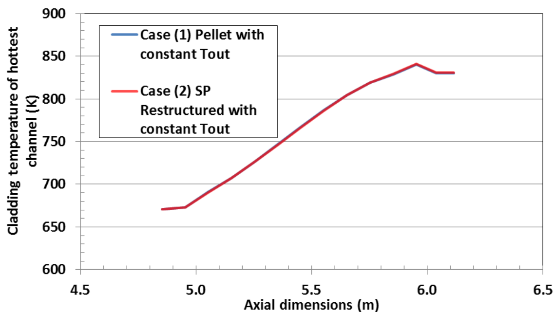
Figure H-2. Axial distribution of the cladding temperature in the hottest ring of the CP-ESFR CONF2 core at equilibrium cycle.
