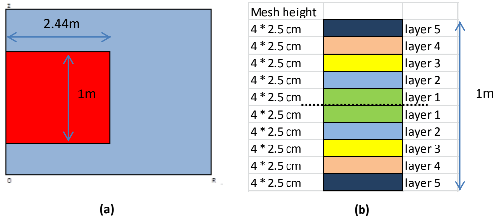
Figure 6-10. (a) Schematics of the simplified CP-ESFR model. Red: fissile core zone of the CP-ESFR core. Blue: liquid Sodium. (b) Axial layout of the fissile zone with symmetric layers.
