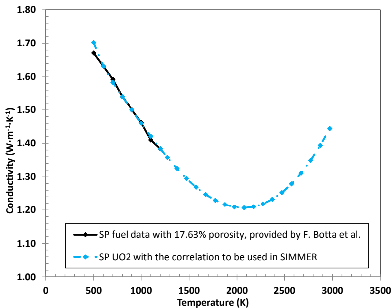
Figure 7-10. Thermal conductivity extrapolation for non-restructured \text{UO}_2 sphere-pac fuels based on data in [181].
