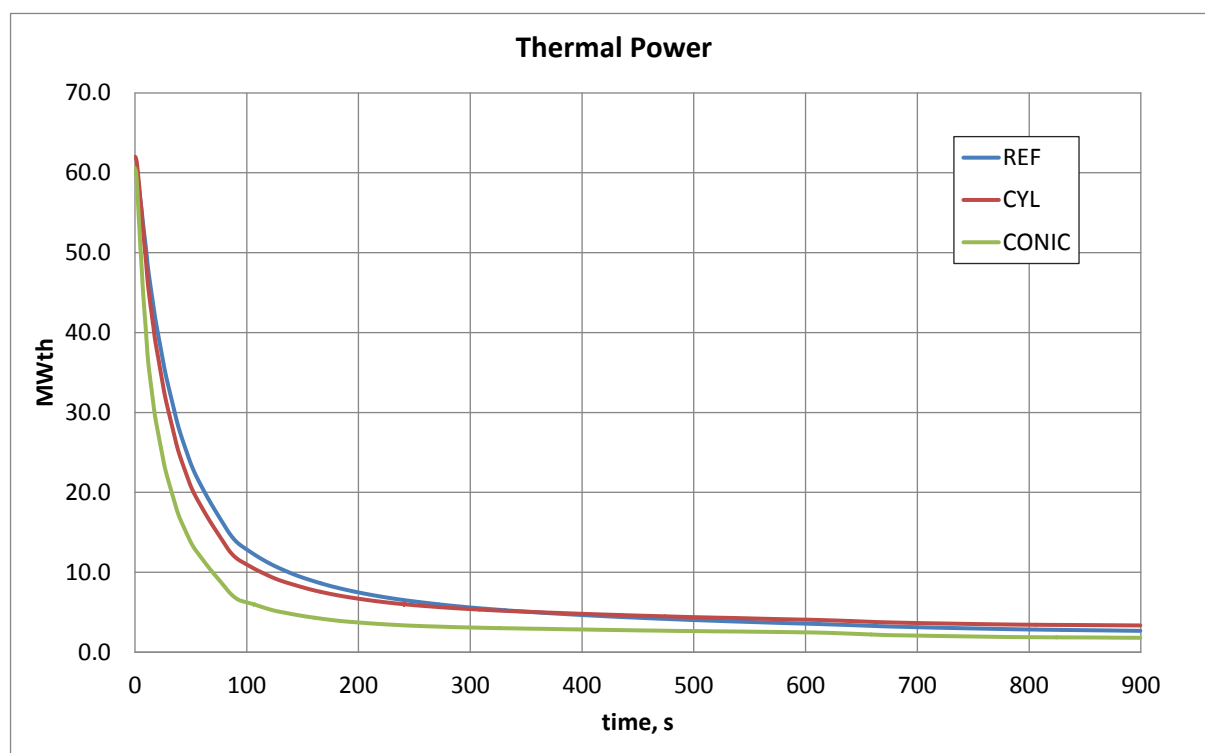
Figure I-4. EBR-II SIMMER results: thermal power versus time comparison three cases: REF, CYL and CONIC
