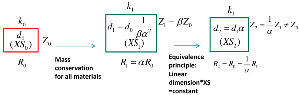
Figure 6-15. Uniform anisotropic expansion. XS stands for cross-section.
