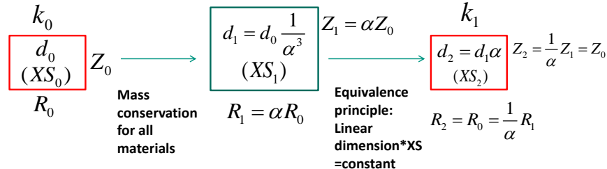
Figure 6-14. Uniform isotropic expansion. XS stands for cross-section.
