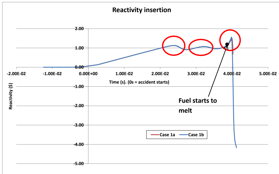
Figure F-6. Reactivity evolution in case of pellet fuel, during a UTOP of 50$/$s.
