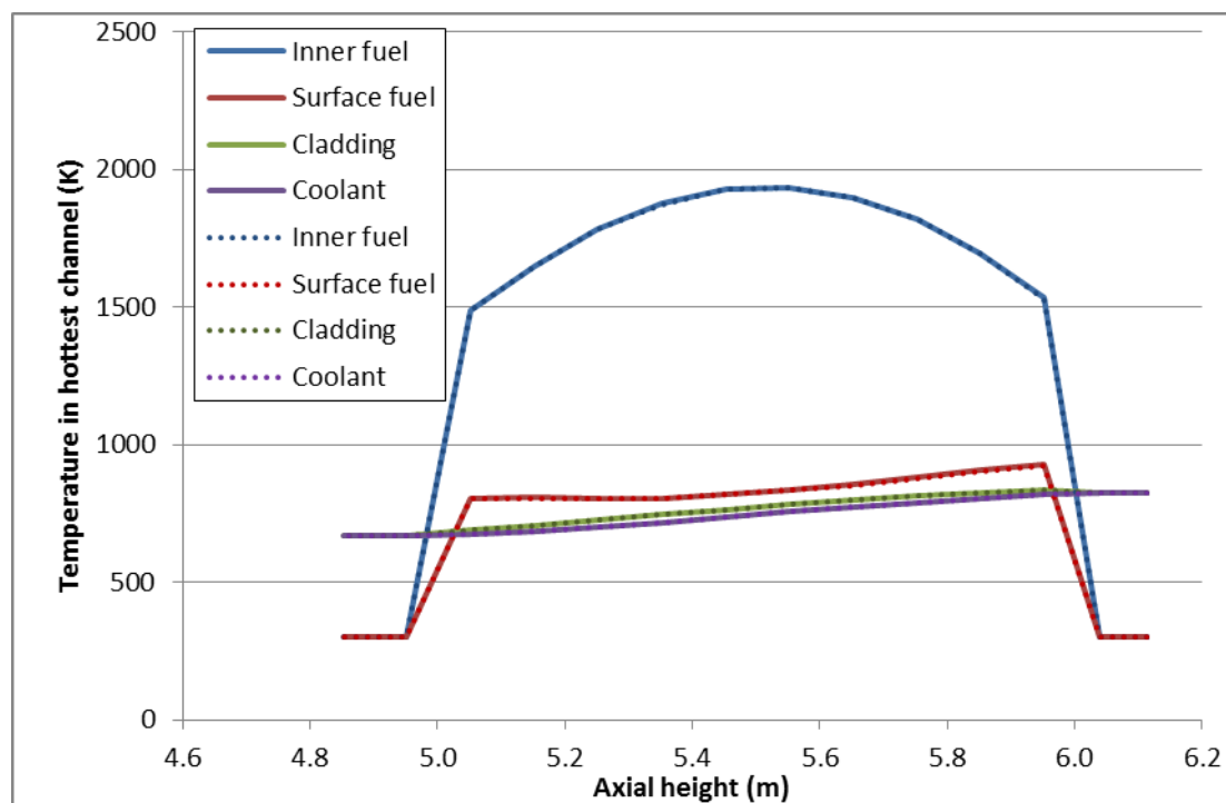
Figure F-5. Axial temperature distribution in the hottest channel, pellet type fuel. Dotted lines: Case 1b, full lines: Case 1a.
