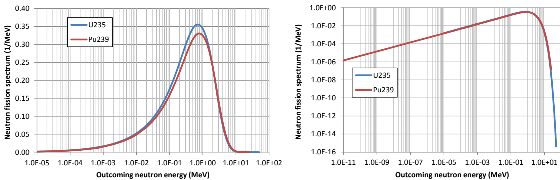
Figure 6-2. Prompt neutron fission spectra of ^{239}\text{Pu} and ^{235}\text{U} based on JEFF3.1 data (in lin-log and in log-log scale).
