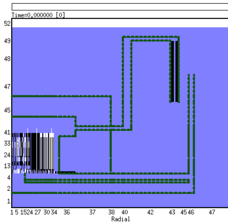
Figure I-1. EBR-II model: reactor vessel and components (core, inlet plenum, upper plenum, Z-pipe, inlet pipes)
