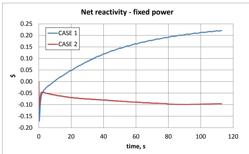
Figure I-10. EBR-II SIMMER results: Cylindrical model, comparison of different steel temperature in input specification (fixed power calculation)
