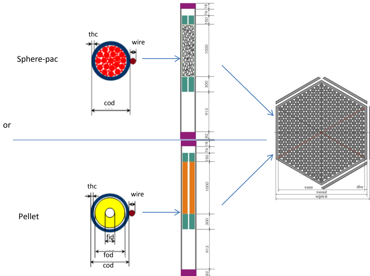
Figure 8-2. Layout of fuel SAs and fuel pins in case of sphere-pac (upper part) and pellet fuel (lower part) [6] (thw=wrapper thickness, xwin= Internal flat-to-flat distance of wrapper tube, xwout= external flat-to-flat distance of wrapper tube, wptch= Fuel assemblies pitch, fid = fuel inner diameter).
