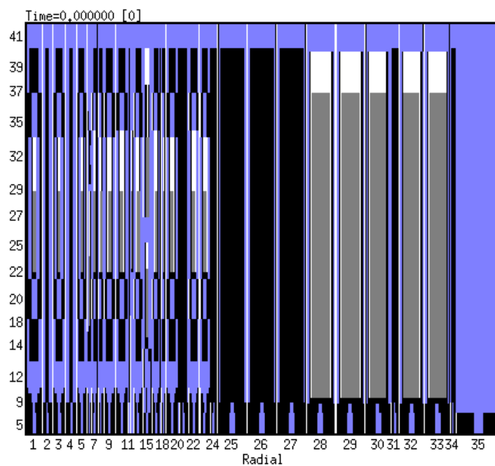
Figure I-2. EBR-II model: core zone
