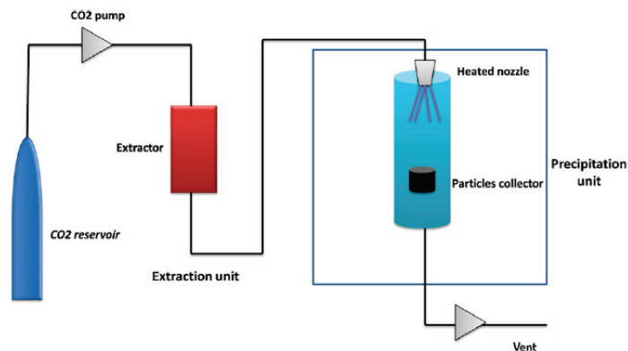
Fig. 7. Rapid expansion of supercritical solutions technique (RESS).
