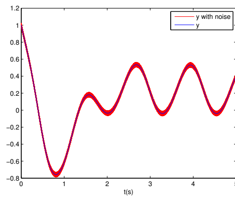
Fig. 5.1 The bounded output and the measurement with noise.
