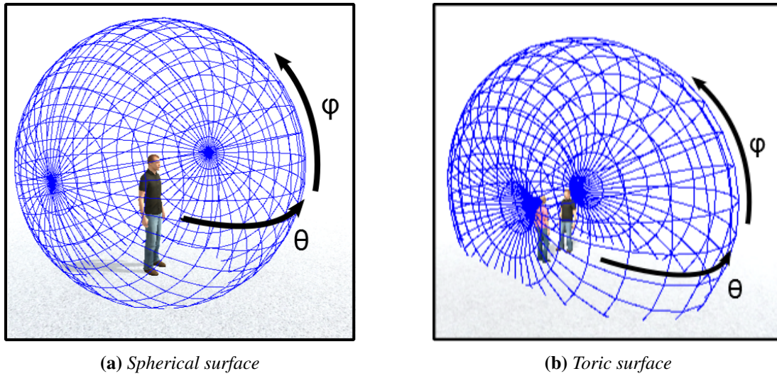
Figure 6.1: Manifold surfaces used to define visual properties in the case of (a) one target and (b) two targets. In both cases, profile and vantage angles are given respectively by \theta and \varphi .
