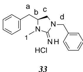
(4S)-1,4-dibenzyl-3-methyl-imidazolidin-2-imine hydrochloride
