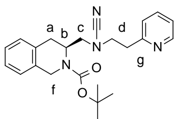
tert-butyl (3S)-3-[[cyano-[2-(2-pyridyl)ethyl]amino]methyl]-3,4-dihydro-1H-isoquinoline-2-carboxylate
