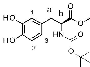
Boc-136
