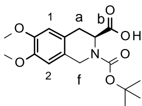
(3S)-2-tert-butoxycarbonyl-6,7-dimethoxy-3,4-dihydro-1H-isoquinoline-3-carboxylic acid 339
