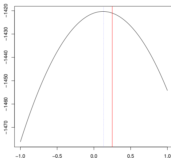
Figure 1.4: Log-likelihood function for 1 000 observations and \vartheta = 0.25
