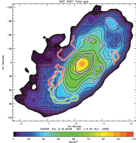
Fig. 7. NGC 4501 total gas surface density \Sigma_g = \Sigma_{\text{HI}} + \Sigma_{\text{H}_2} . Thin black contours levels are (4.0, 4.36, 5.44, 7.24, 9.76, 13.0, 16.96, 21.64, 27.04, 33.16, 40.0, 47.56, 55.84, 64.84, 74.56) \text{M}_\odot \text{pc}^{-2} . The resolution is 17'' . Blue contour: high atomic gas surface density regions. Green contour: southern "U" shaped region with low SFE_{\text{H}_2} . Orange contour: northern low SFE_{\text{H}_2} region. Red contour: high R_{\text{mol}}/P_{\text{tot}} region. Purple contour: central region defined from the stellar surface density excluded from the fit.
