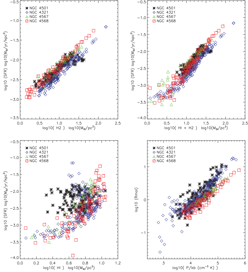
Fig. 22. NGC 4501, NGC 4567/8, and NGC 4321. Upper left panel: SFR as a function of \Sigma_{H_2} . Upper right panel: SFR as a function of total gas surface density. Lower left panel: SFR as a function of atomic gas surface density. Lower right: molecular ratio as a function of the ISM pressure P_{\text{tot}} .
