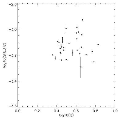
Fig. 28. NGC 4567. Same panels as in Fig. 27
