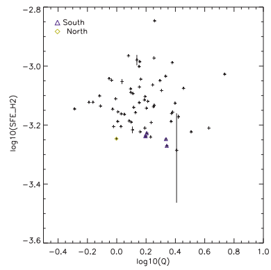
Fig. 29. NGC 4568. Same panels as in Fig. 27
