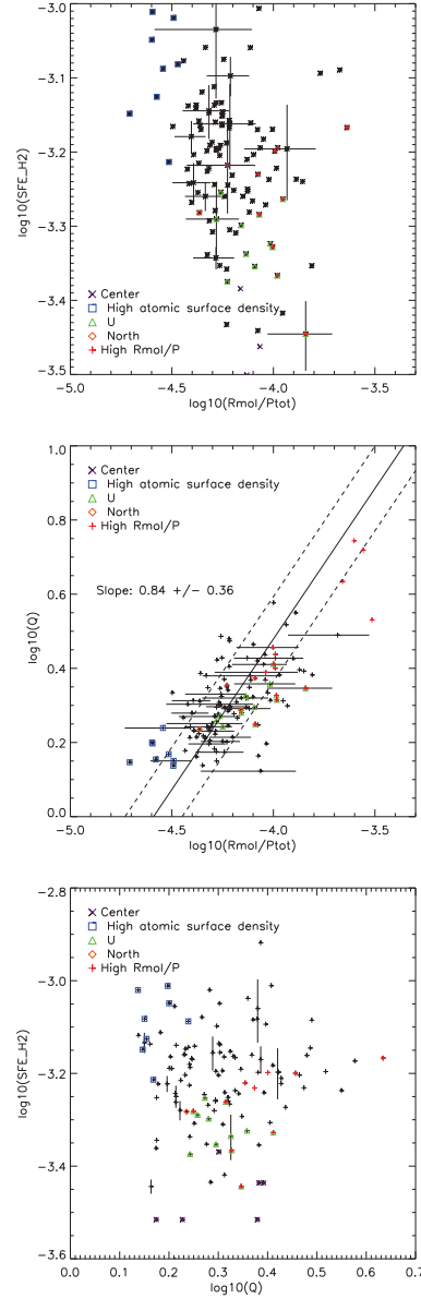
Fig. 27. NGC 4501: left panel: \text{SFE}_{\text{H}_2} as a function of the molecular fraction over ISM pressure. Right panel: Toomre Q as a function of R_{\text{mol}}/P_{\text{tot}} . Lower panel: \text{SFE}_{\text{H}_2} as a function of Toomre Q .
