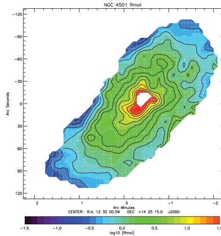
Fig. 9. NGC 4501 molecular ratio R_{\text{mol}} = \Sigma_{\text{H}_2}/\Sigma_{\text{HI}} . The resolution is 17'' . Contour levels are (0.04, 0.06, 0.1, 0.16, 0.25, 0.4, 0.63, 1, 1.58, 2.51, 3.98, 6.31, 10, 15.84, 25.11)
