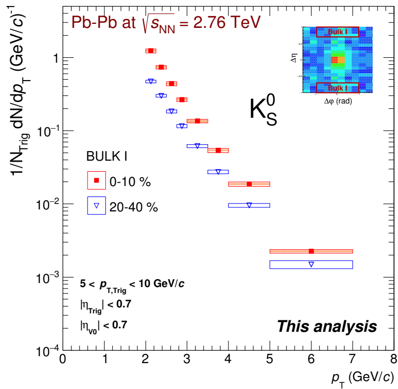
Figure 4.1: Per-trigger yield of K_S^0 in the Bulk I sample for 0-10% and 20-40% centrality selections of the 2011 Pb–Pb collisions. The markers are located at the middle value of the p_T -bin. The horizontal extension of the boxes represents the p_T -bin width. Statistical uncertainties are plotted as vertical lines. The empty (shaded) boxes stand for the uncorrelated (partially correlated) systematic uncertainties.
