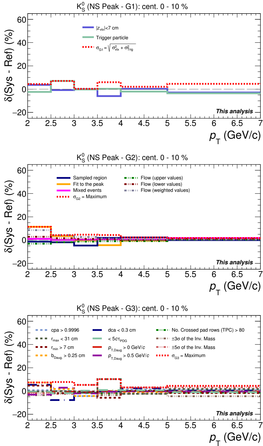
Figure 4.18: Systematics uncertainties for K_S^0 per-trigger yield in the near-side peak (NS) for the centrality 0-10%.
