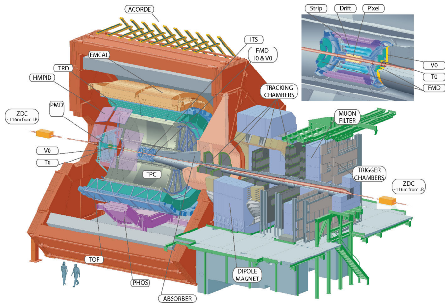
Figure 2.3: The layout of the ALICE experiment [134].
