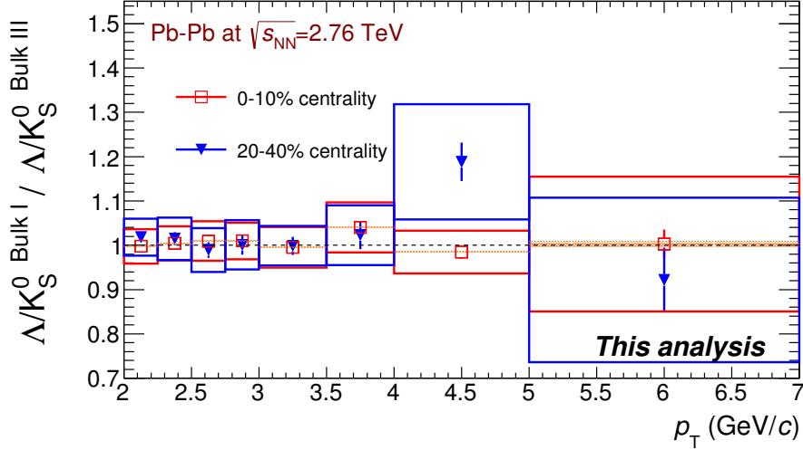
Figure 4.10: Double ratio of \Lambda/K_S^0 in Bulk I to Bulk III. The results are presented for the 0-10% (open square) and 20-40% (up-side-down triangle) centrality intervals in 2011 Pb–Pb run. The \bar{\Lambda} is not included in the single ratio results. The vertical lines are the statistical uncertainties. The empty (filled) boxes are the uncorrelated (partially correlated) systematic uncertainties.
