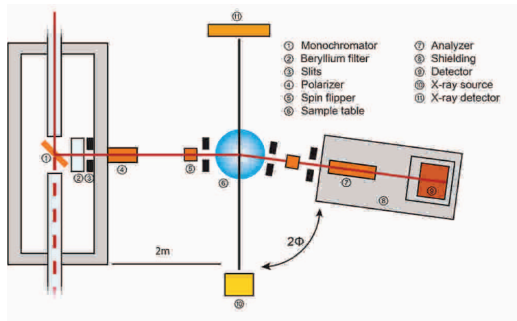
Figure 2.9: Schematic layout of the N-REX+ reflectometer. Reprinted from reference [24].
