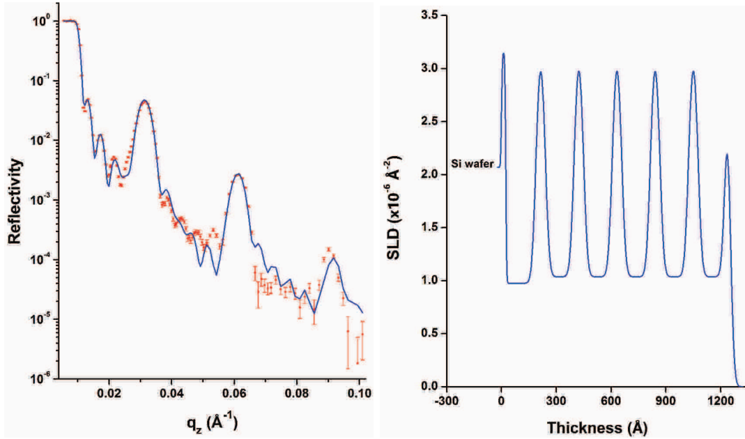
Figure 5.1: On the left, the experimental specular reflectivity curve (points) and the corresponding theoretical model (line). On the right, the SLD profile extracted from the fit.
