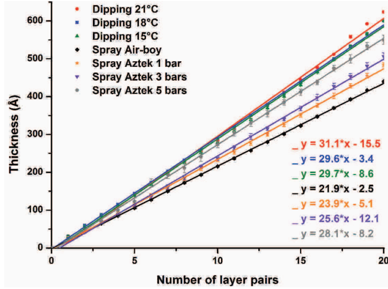
Figure 2.17: Evolution of the thickness of multilayer films composed of 20 layer pairs ( \text{PSS}_{h7} -PAH) as a function of the number of layer pairs. Films prepared by dipping at different temperature and by spraying at different gas pressure are shown. Lines correspond to linear fits of the curves.
