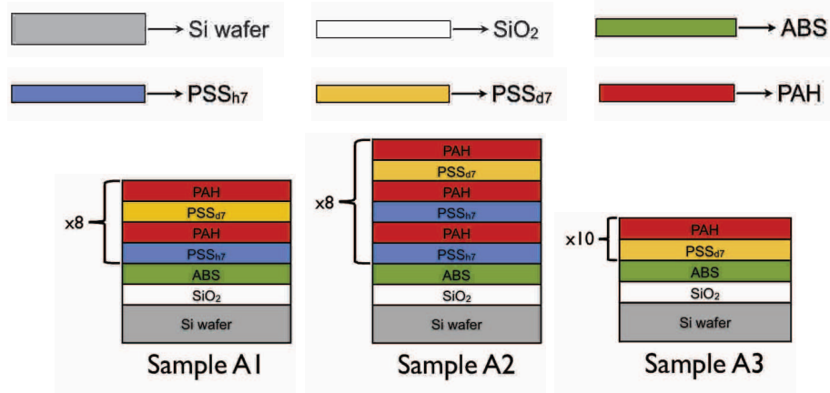
Figure 3.2: Layer sequences for Sample A1, A2 and A3. The proportions of the layer thicknesses are not kept.
