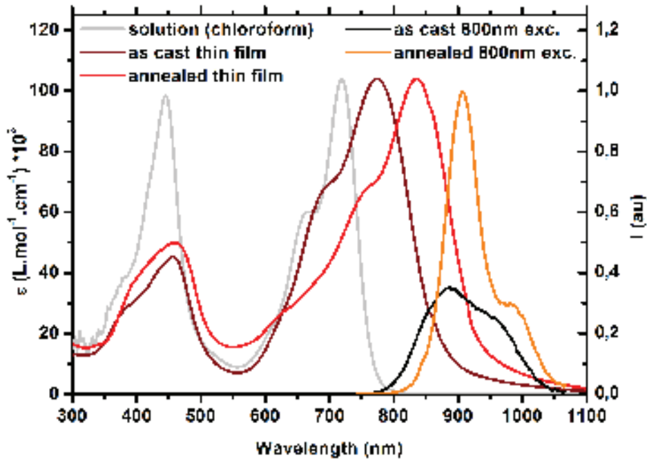
Figure 5.3.: Molar absorption spectrum of TB2 in solution, as cast in film and after 10min annealing at 110^{\circ}C (left scale) and fluorescence spectra normalised for the number of absorbed photons of as cast and annealed TB2 films excited at 800nm (right scale).
