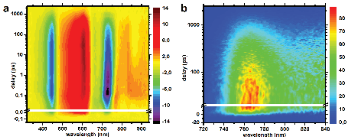
Figure 5.10.: Transient absorption (left) and fluorescence (right) data of TB2 excited at 600nm.
