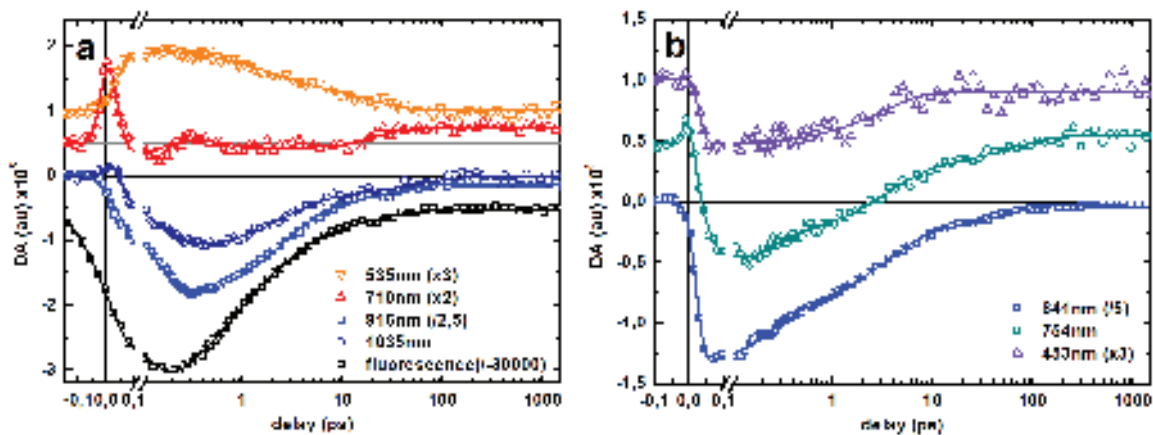
Figure 5.22.: Transient absorption kinetics of pristine TB2 films annealed on ITO/PEDOT:PSS at different wavelengths. ESA and SE dominated kinetics are presented in panel a, together with the TF kinetic trace obtained by fluorescence up-conversion. Panel b shows GSB dominated kinetic traces. Raw data are displayed as scatter plots and multi exponential fits in thick lines of the corresponding color.
