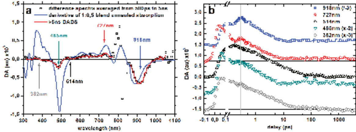
Figure 6.17.: Polaron signature and its hundred femtosecond formation in annealed 1:0.5 weight ratio blend of BODIPY:PCBM on ITO/PEDOT:PSS substrate. On the right, scaled kinetics at characteristic wavelengths of the polaron spectrum (positive, negative and null signal). See legends on the graphs.
