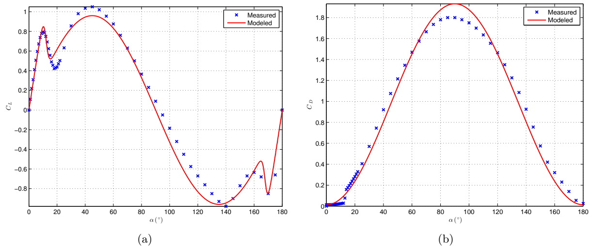
Figure 2.18: The measured (wind tunnel measurement and computer synthesis [56]) and modeled (a) lift and (b) drag coefficients versus the angle of attack at \text{Re} = 160000 for NACA0018 airfoil
