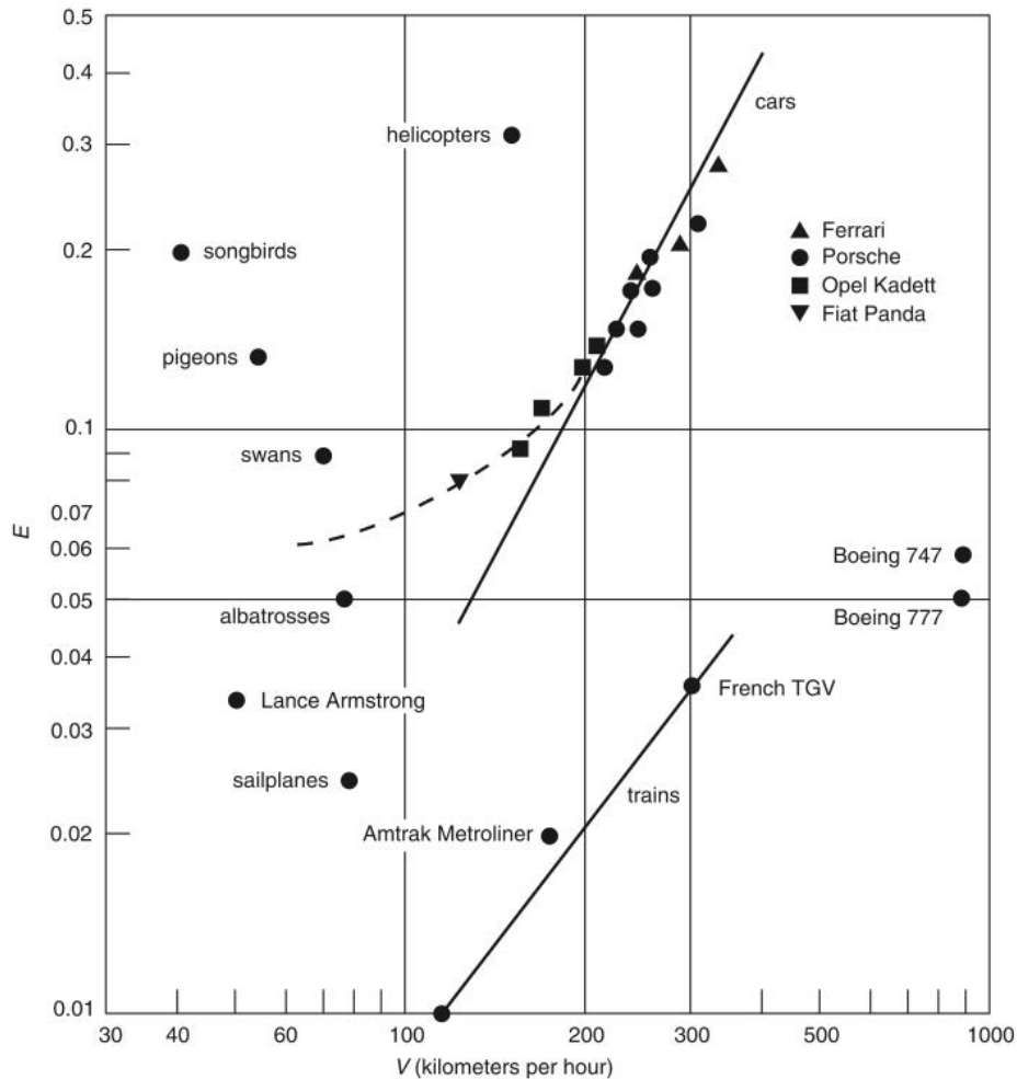
Figure 1.24: Specific energy consumption plotted against the speed [39]
