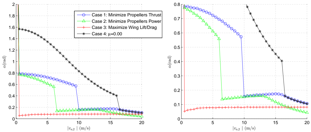
Figure 2.29: The angle of attack \alpha versus the speed (when |\mathbf{v}_a| = 0 , \alpha is not defined)
