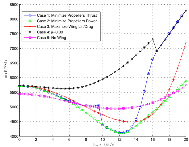
Figure 2.31: The rotor angular velocity versus the speed
