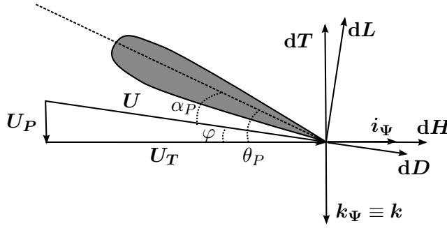
Figure 2.9: Force components on a blade element (adapted from [23, p. 68 Fig. 5.4])
