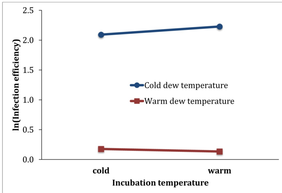
Figure 1. Infection efficiency for the four combinations of cold and warm dew and incubation temperatures. Non-parallel lines illustrate the significant dew temperature * incubation temperature interaction in Table 3.
