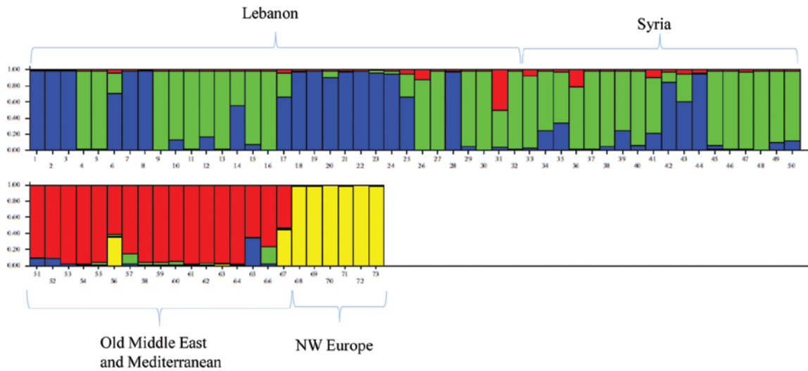
Supplementary figure 2: Clustering of 362 Puccinia striiformis f. sp. tritici isolates collected in Lebanon and Syria in 2010-2011 (50 MLG), in Middle East and Mediterranean in 2004-2005 (17 MLG), and in North-Western Europe in 2008-2009 (6 MLG), using STRUCTURE at K=4 following the method of Evanno et al. (2005).
